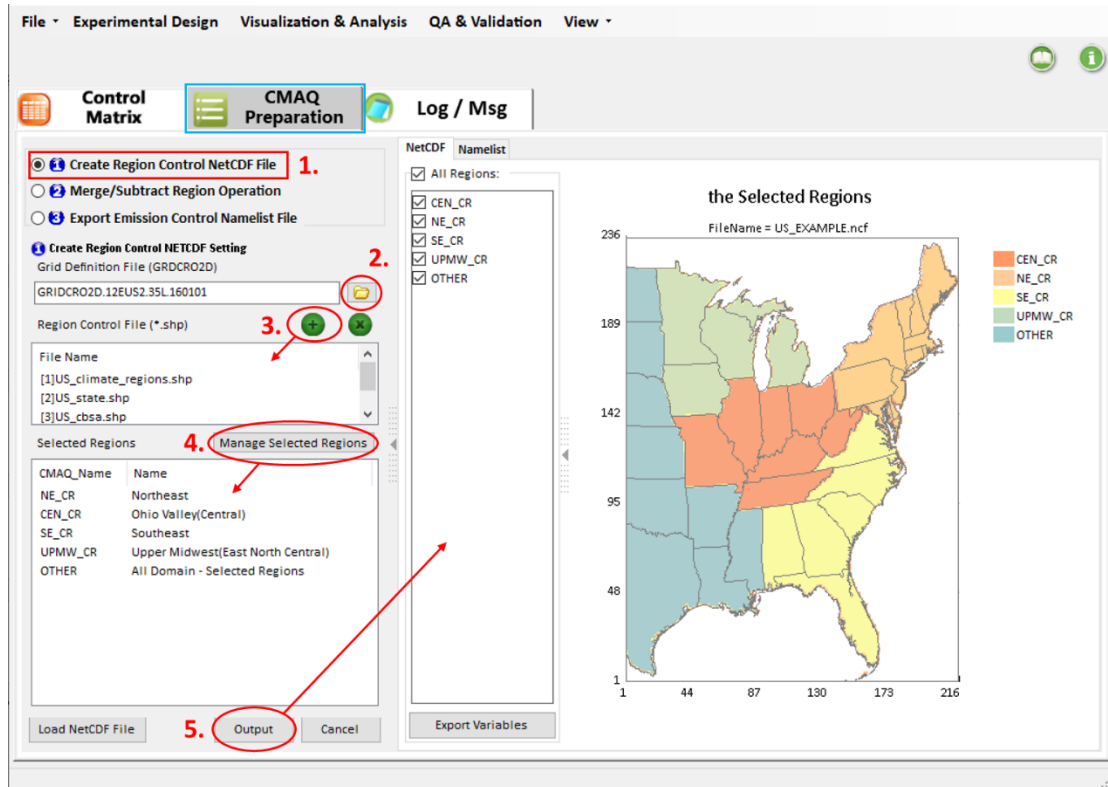
Fig. 12 Create Region Control NetCDF File
