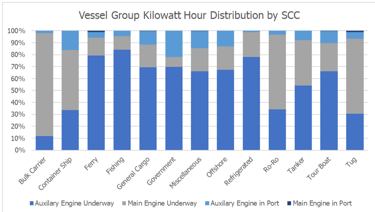
Figure 8. Ship Type Kilowatt Hour Distribution by SCC
