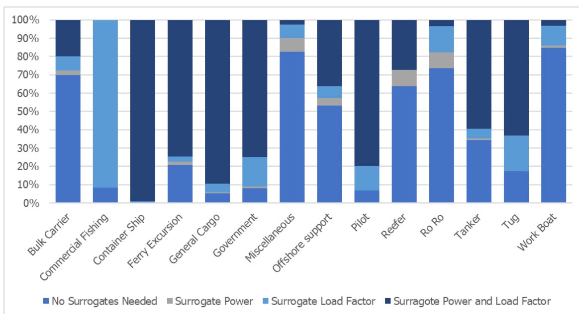
Figure 5. Use of Propulsion Surrogates for the 2021 Vessel Fleet (percent)
