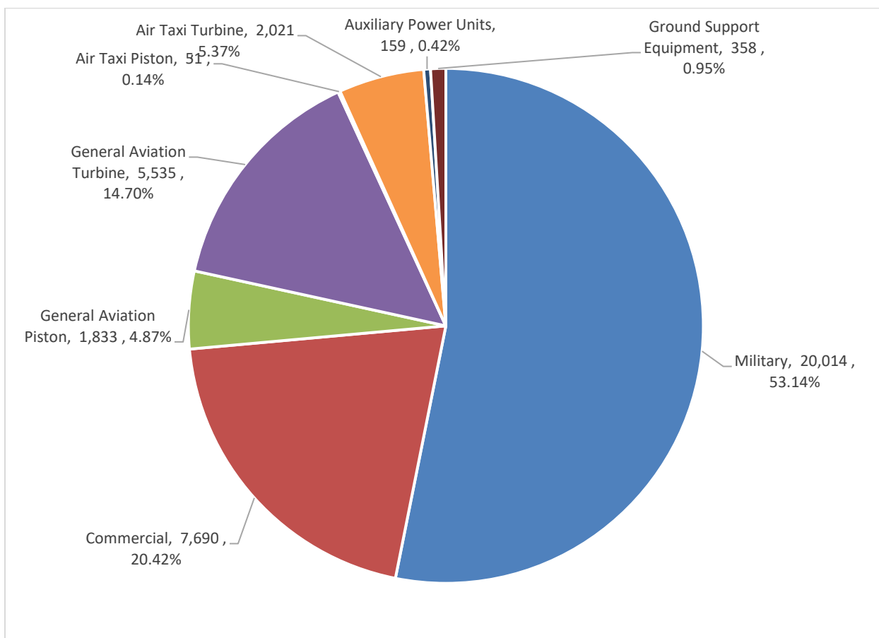
Figure 5-1. Total Annual 2020 Airport VOC Emissions (tons) by SCC Descriptions
