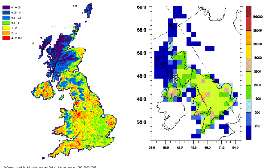
Fig. 1. Comparison of UK NAEI (left) and EMEP (right) emission maps for NH 3 for the year 2005
