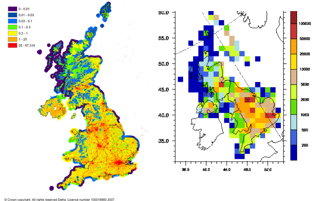
Fig. 2. Comparison of UK NAEI (left) and EMEP (right) emission maps for NO x for the year 2005
