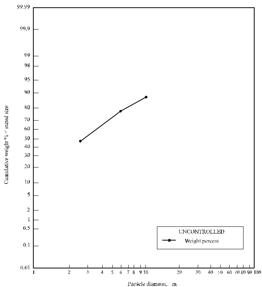
8.10 SULFURIC ACID: SECONDARY ABSORBER
