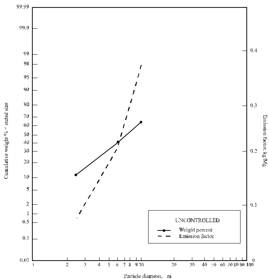
9.9.1 FEED AND GRAIN MILLS AND ELEVATORS: CONVEYING
