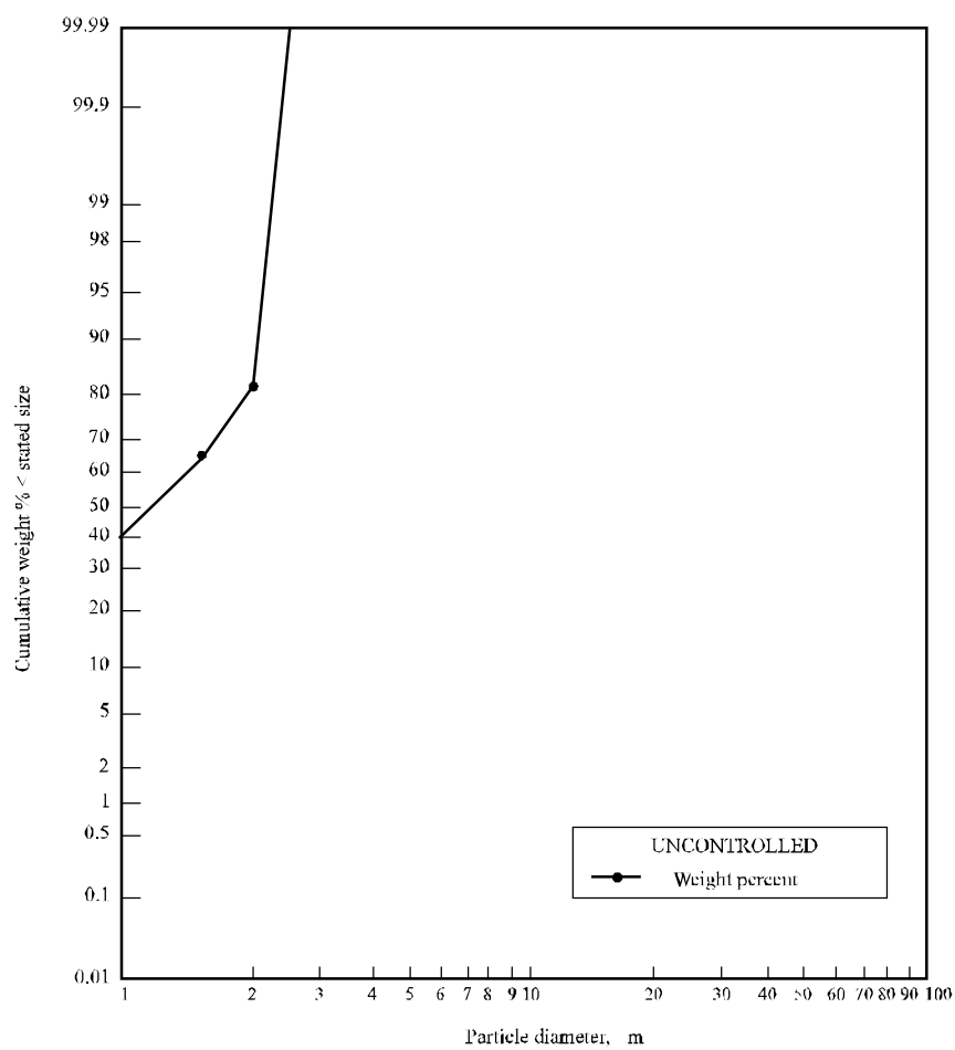
8.10 SULFURIC ACID: ABSORBER, 32% OLEUM
