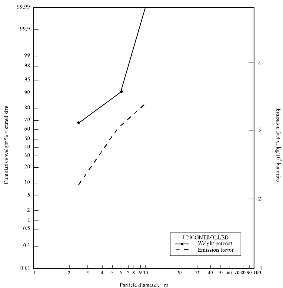
12.15 STORAGE BATTERY PRODUCTION: GRID CASTING AND PASTE MIXING
