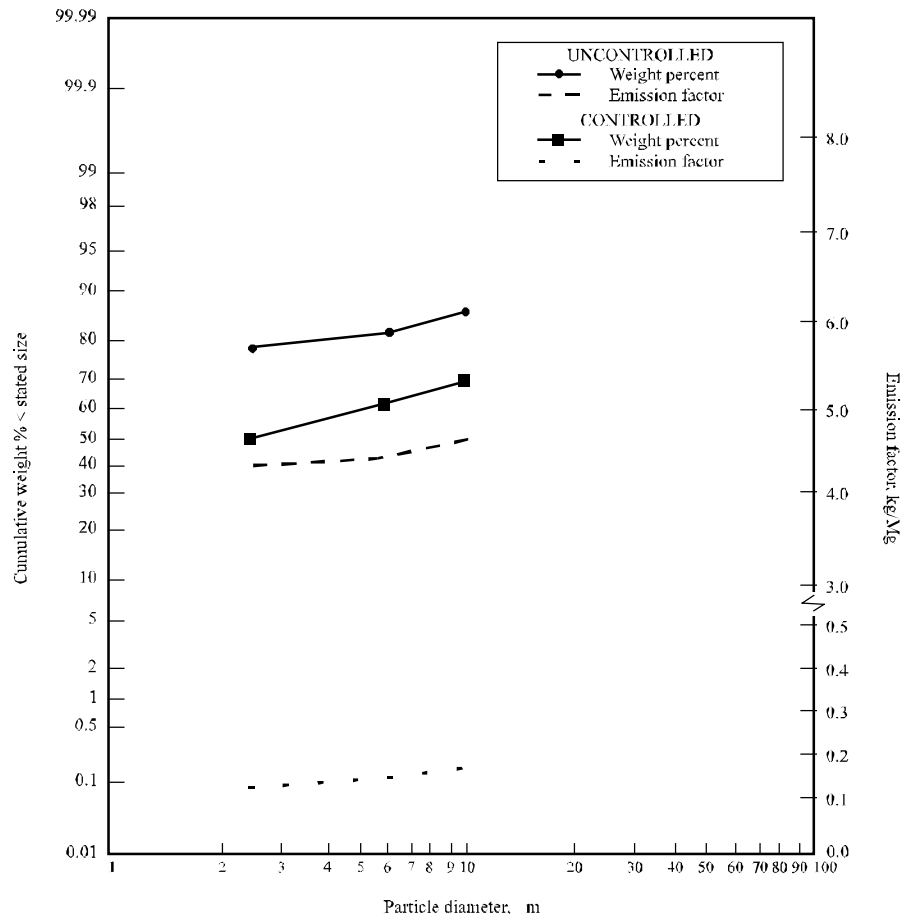
12.13 STEEL FOUNDRIES: OPEN HEARTH EXHAUST
