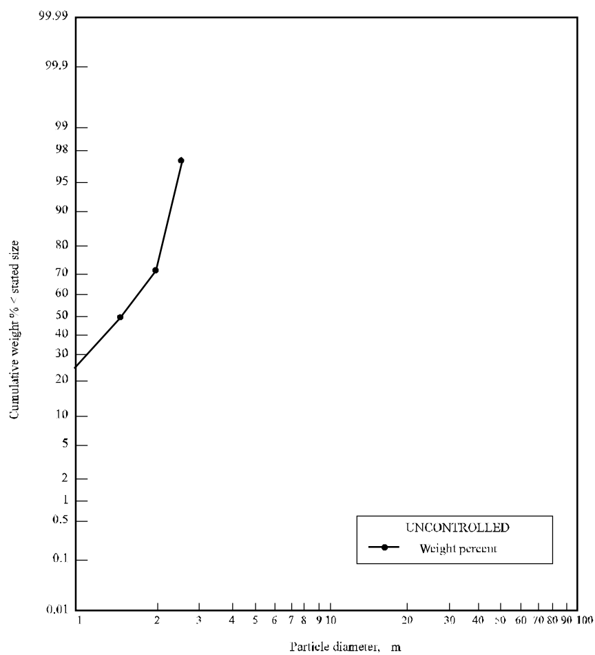
8.10 SULFURIC ACID: ABSORBER, 20% OLEUM
