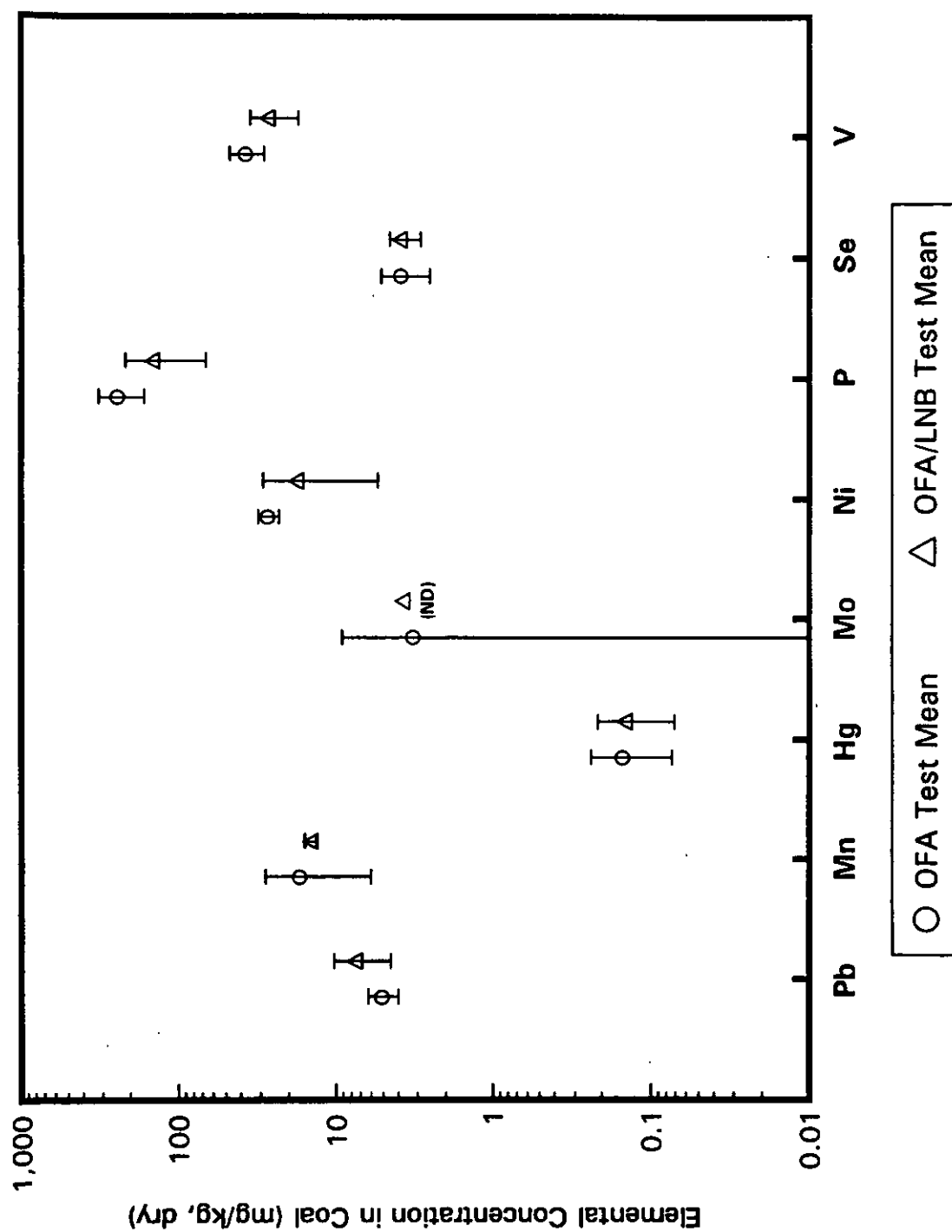
Figure 4-1b Comparison of Coal Compositions
