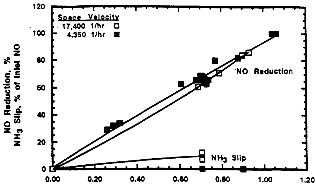
Figure 5-49a. T_1O_2 corrugated plate catalyst NO_x conversion and residual NH_3 versus NH_3 -to- NO_x ratio. 133
