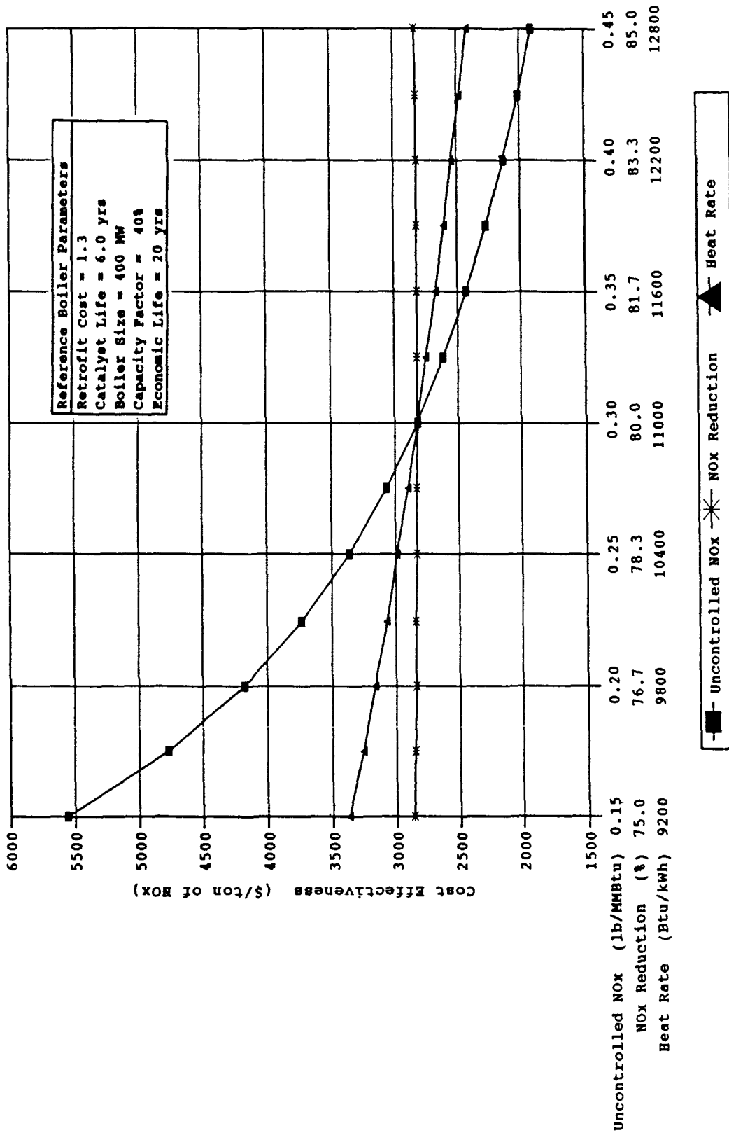
Figure 6-58. Impact of NO x emission characteristics and heat rate on SCR cost effectiveness for oil-fired tangential boilers.
