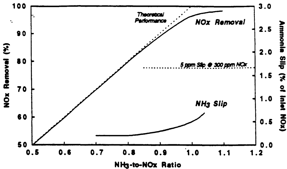
Figure 5-47a. Extruded catalyst \text{NO}_x conversion and residual \text{NH}_3 versus \text{NH}_3 -to- \text{NO}_x Ratio. 131
