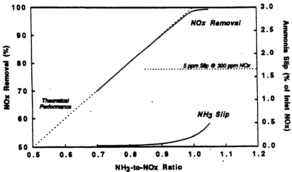
Figure 5-47b. Replacement composite catalyst \text{NO}_x conversion and residual \text{NH}_3 versus \text{NH}_3 -to- \text{NO}_x Ratio. 131
