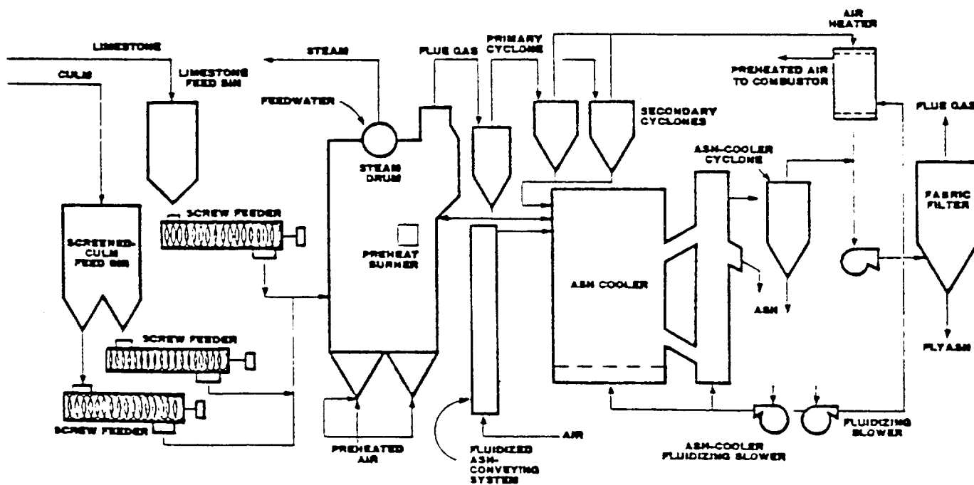
Figure 3.3 Boiler System
