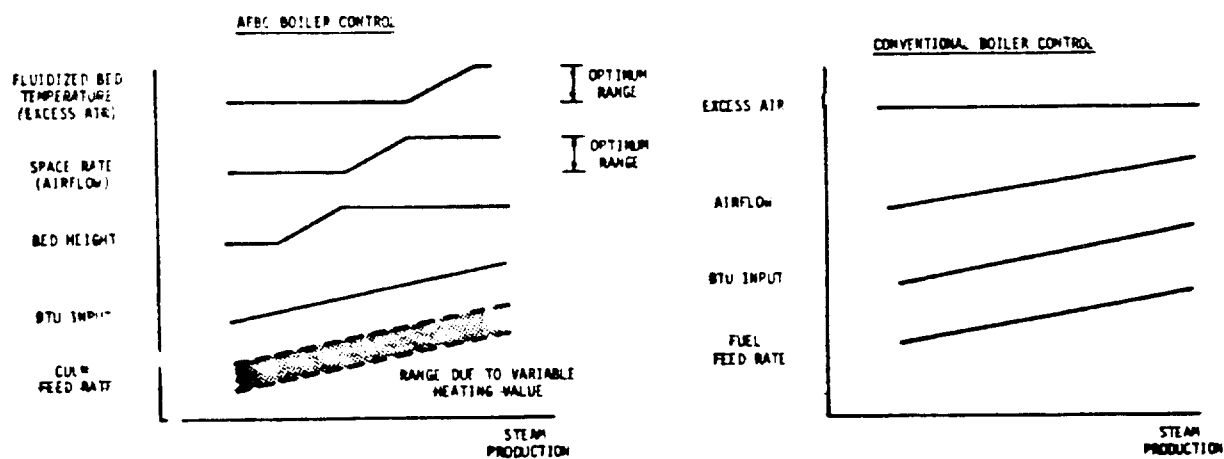
Figure 3.7 Comparison Between AFBB Control and Conventional Boiler Control
