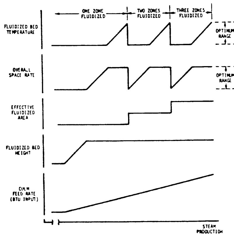
Figure 3.9 Operating Variables During Load-Following Turndown
