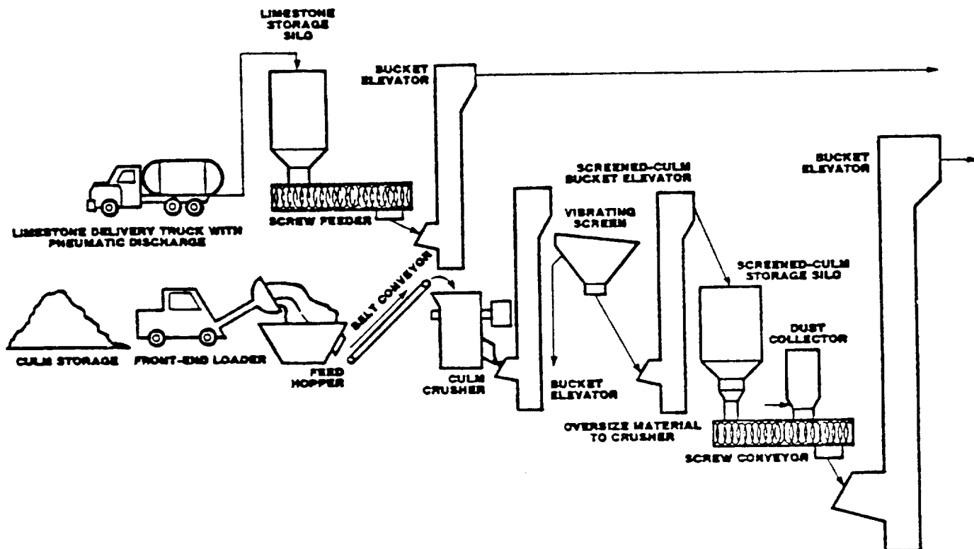
Figure 3.2 Feed Preparation and Storage
