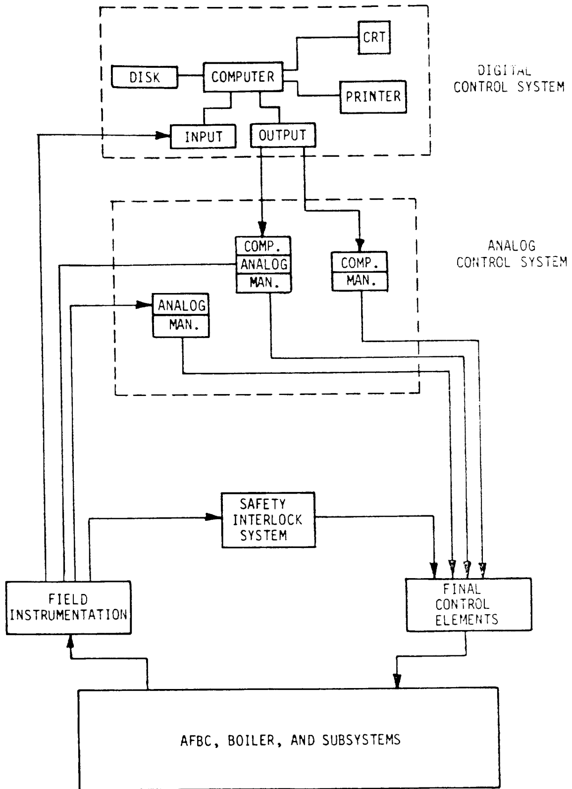
AFBB Process Control System
