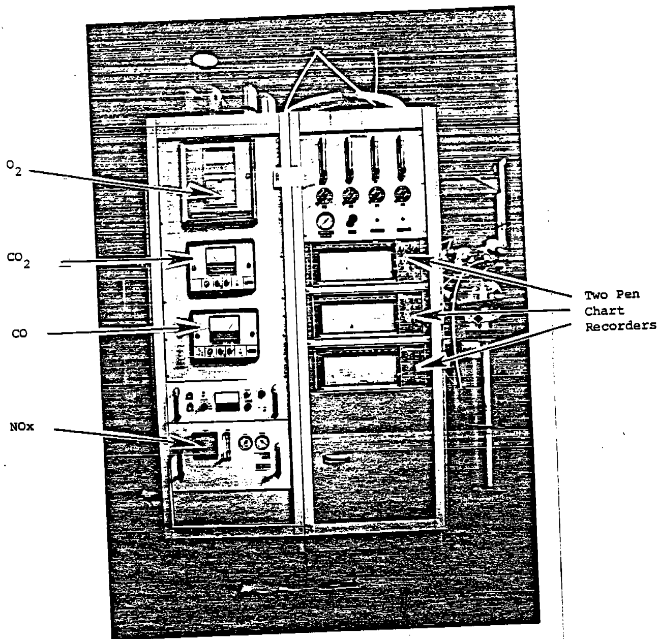
Figure 2-1. Photograph of KVB Continuous Monitor for Measuring Gaseous Emissions
