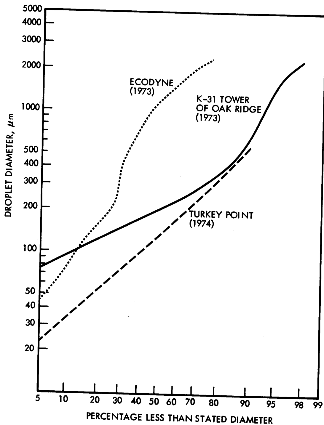
Figure 6. Cumulative Drift Droplet Size Distributions of Three Mechanical Draft Cooling Towers
