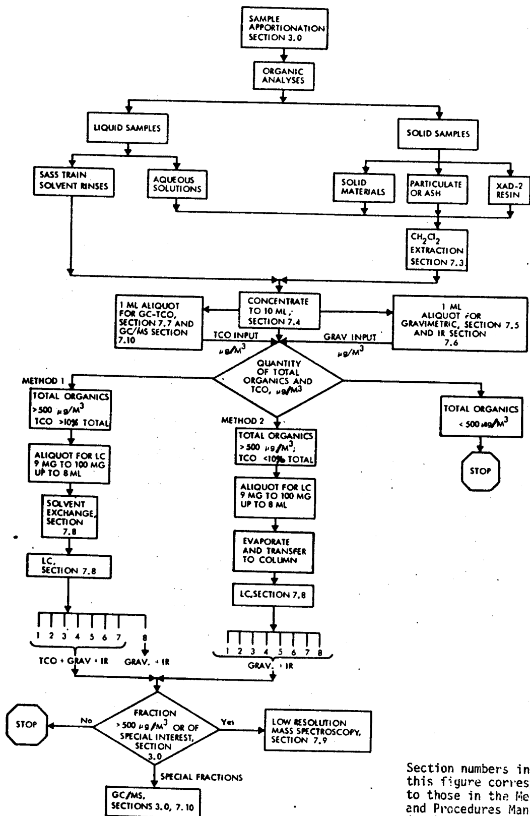
Figure 14. Level I Organic Analysis Methodology
