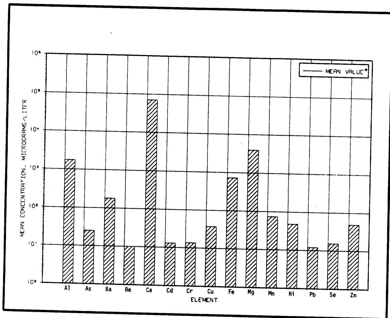
Figure 23. Mean Trace Element Concentrations in Combined Ash Pond Overflow Obtained by Combining Data from Present and Past Studies
