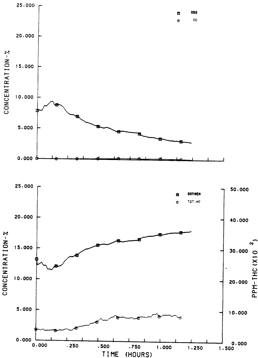
FIGURE B-3. COMPOSITION OF GAS FROM DOWN DRAFT BURNING Burning small split oak cordwood Burning rate 19.1 lb/hr (8.7 Kg/hr).
