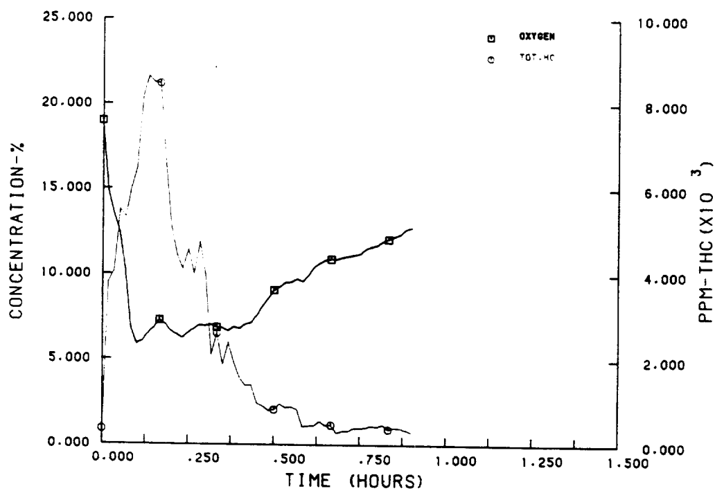
FIGURE B-2. COMPOSITION OF GAS FROM SIDE DRAFT BURNING Burning split oak logs Burning rate 16.6 lb/hr (7.5 Kg/hr).
