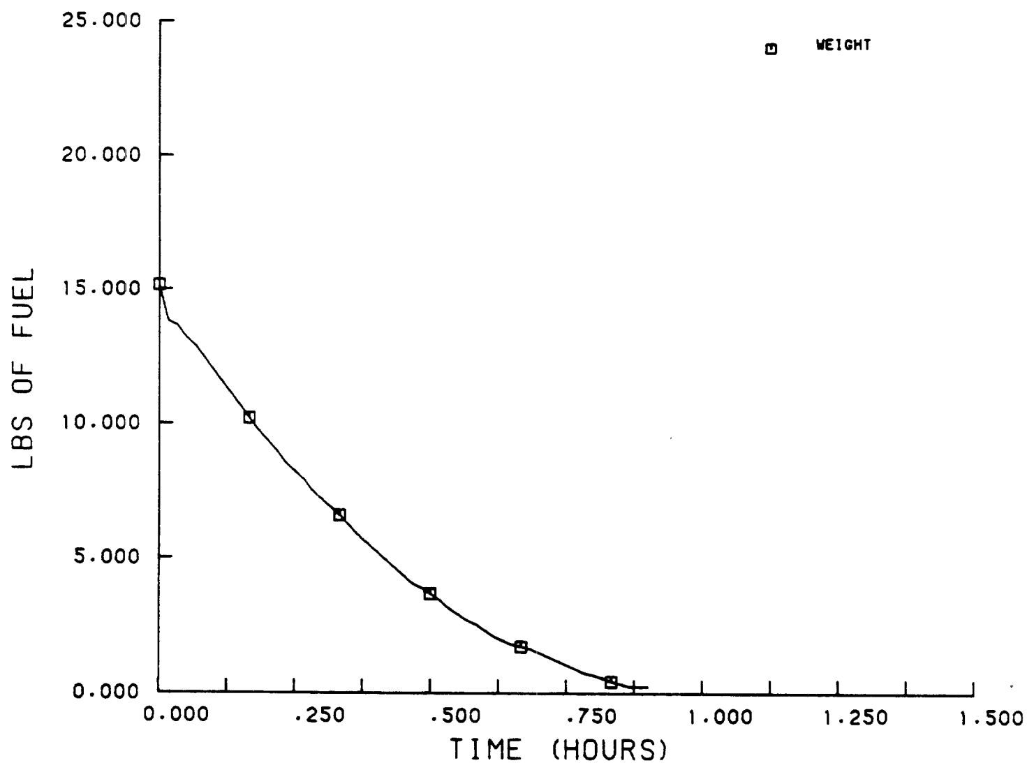
FIGURE B-5. WEIGHT LOSS DURING SIDE DRAFT BURNING Burning split oak logs Burning rate: 16.6 lb/hr (7.5 Kg/hr).
