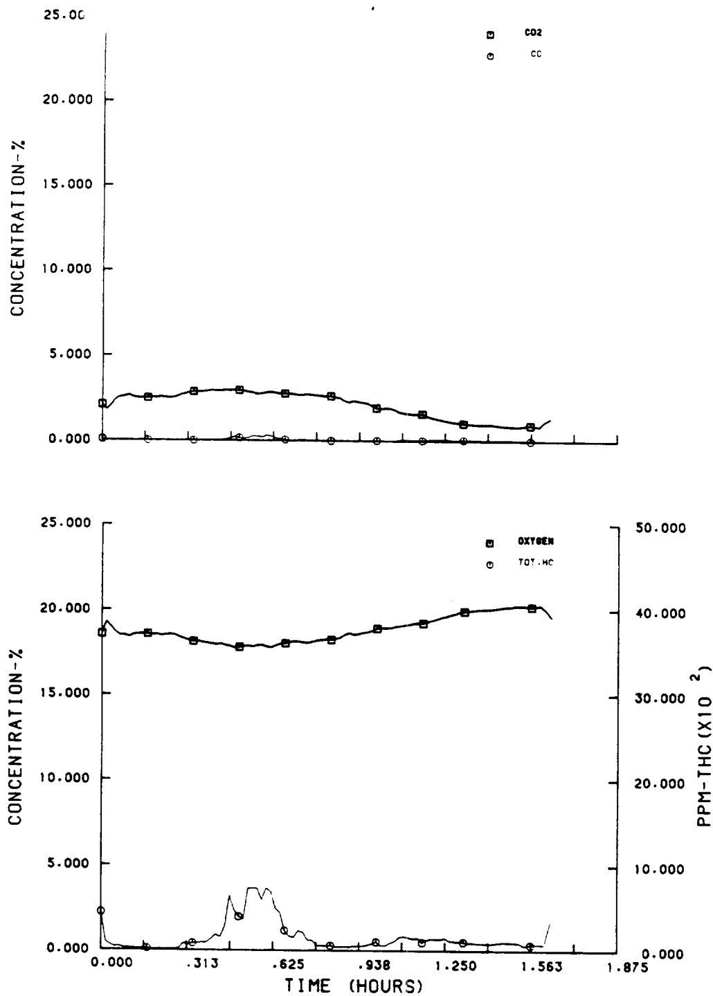
FIGURE B-4. COMPOSITION OF GAS FROM HIGH TURBULENCE BURNING Burning split oak logs Burning rate 24.1 lb/hr (11 Kg/hr).
