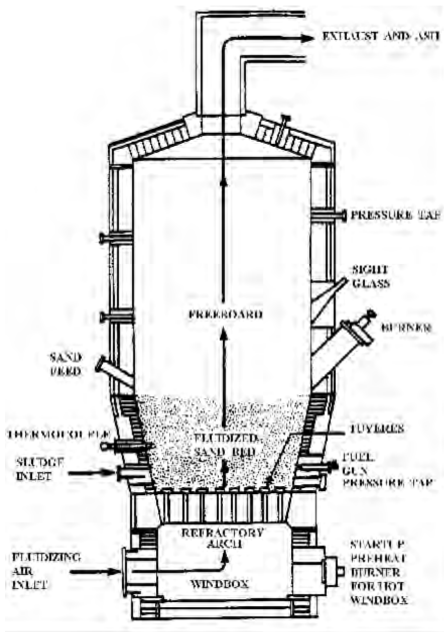
Figure 2.2-2. Cross Section of a Fluidized Bed Furnace
