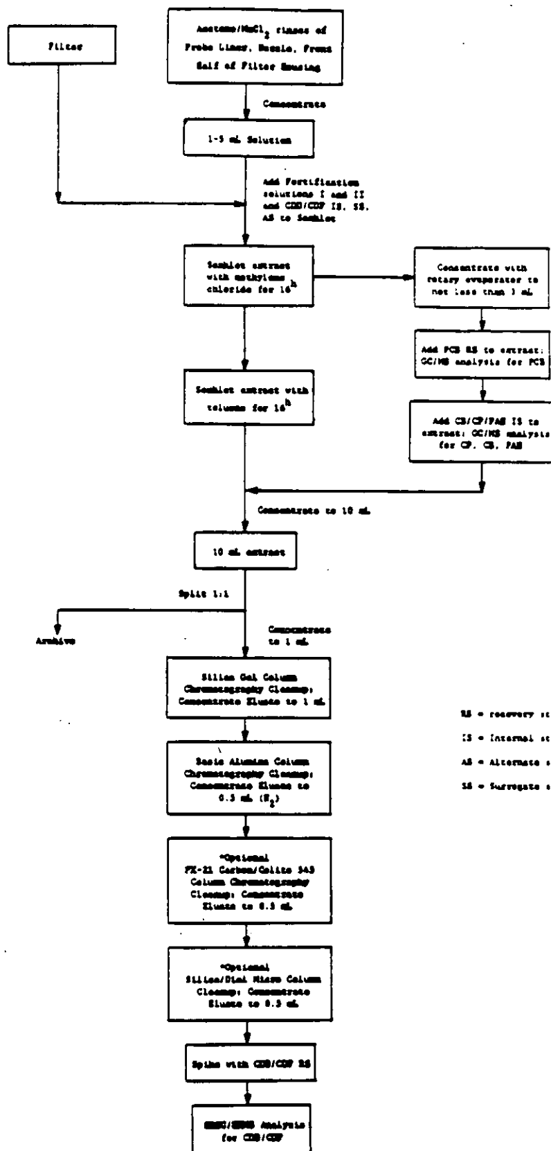
Figure 5-5. Extraction and analysis schematic for CDD/CDF/CB/CP/PCB/PAH flue gas samples.
