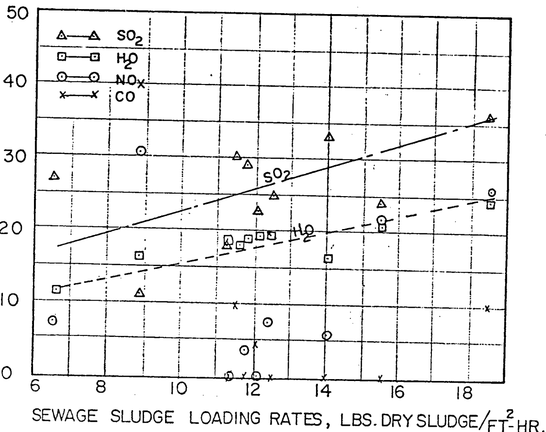
FIGURE 3. GASEOUS POLLUTANT EMISSIONS AT VARIOUS SLUDGE LOADINGS
