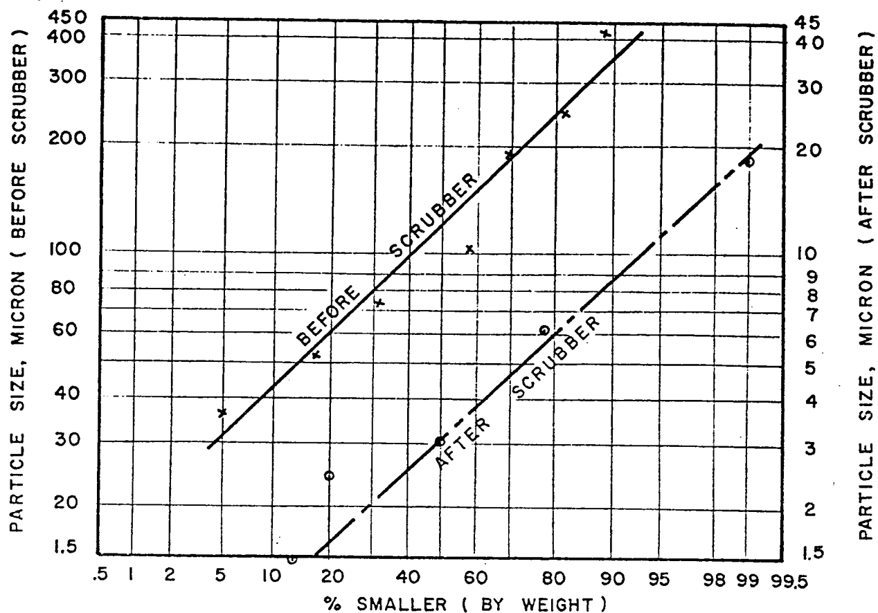
FIGURE 4. EXHAUST PARTICLE SIZE DISTRIBUTION
