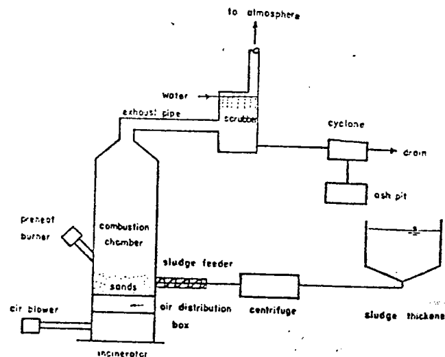
FIGURE 1. FLUIDIZED BED SEWAGE SLUDGE INCINERATION
