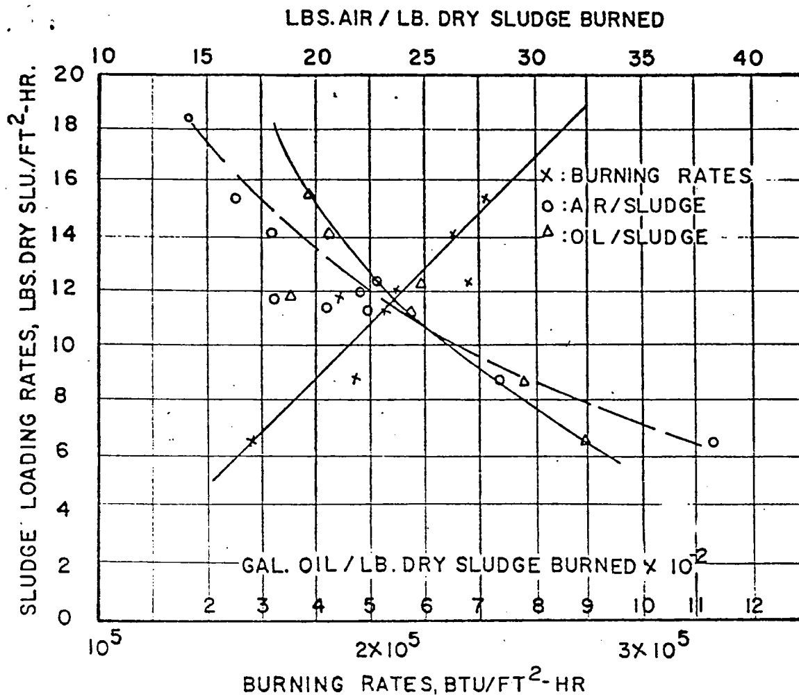
FIGURE 5. AUXILIARY FUEL AND AIR REQUIREMENTS AT DIFFERENT SLUDGE LOADINGS
