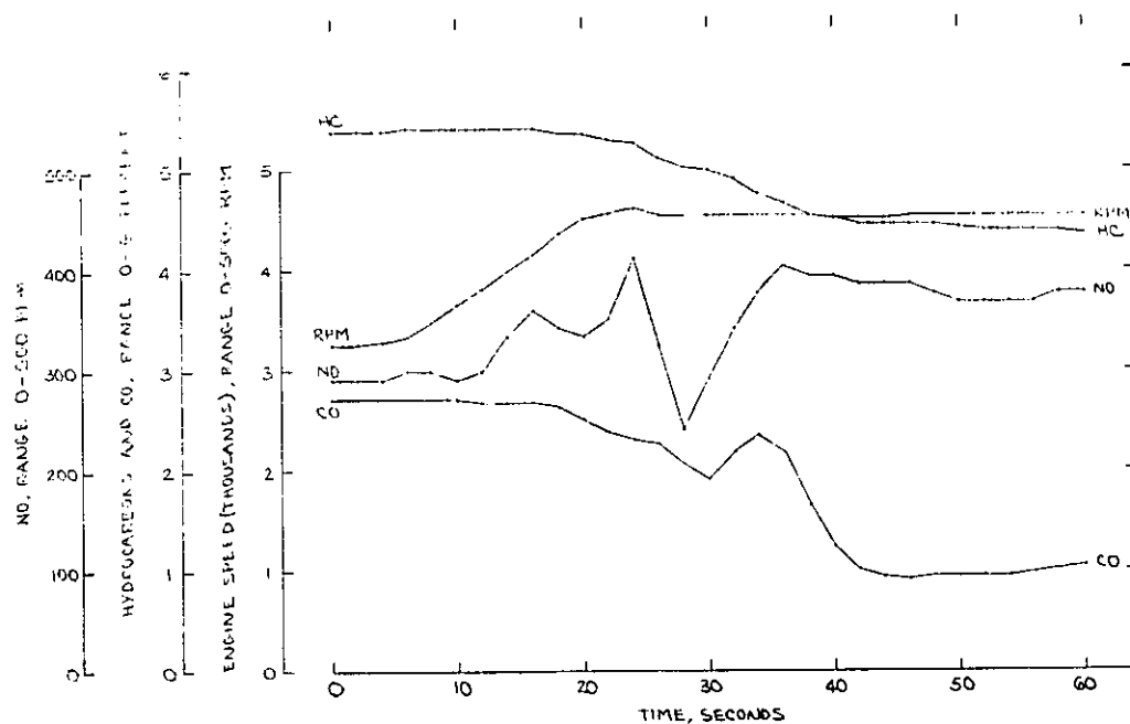
FIGURE C-16. TRANSITION BETWEEN 3300 RPM (FULL LOAD) AND 4500 RPM (FULL LOAD) FOR THE TECUMSEH AHS20 TYPE 1448 ENGINE (RUN T4B) — CONSTANT THROTTLE, LOAD DECREASING
