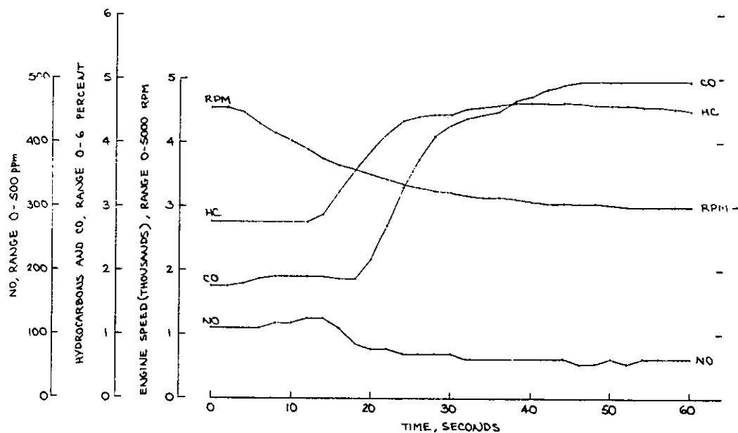
FIGURE C-14. TRANSITION BETWEEN 4500 RPM (NO LOAD) AND 3000 RPM (NO LOAD) FOR THE TECUMSEH AH520 TYPE 1448 ENGINE (RUN T1A) — CONSTANT LOAD, THROTTLE CLOSING
