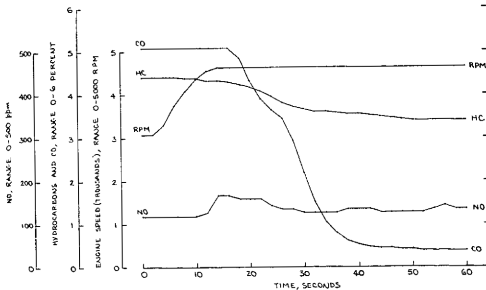
FIGURE C-19. TRANSITION BETWEEN 3100 RPM (NO LOAD) AND 4600 RPM (NO LOAD) FOR THE TECUMSEH AH520 TYPE 1448 ENGINE (RUN 78A) — CONSTANT LOAD, THROTTLE BEING OPENED
