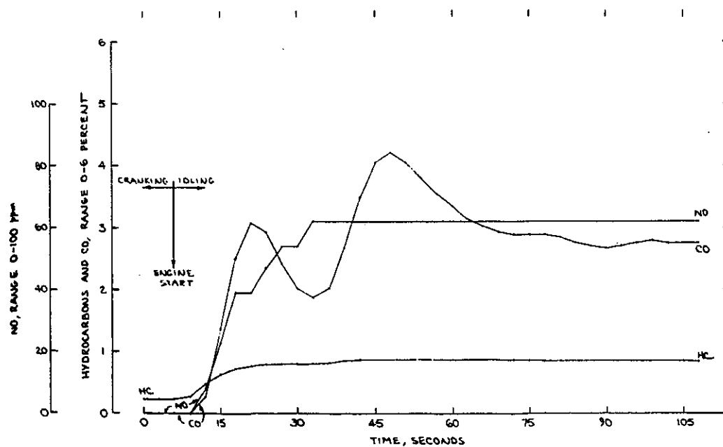
FIGURE C-21. COLD START AND IDLE FOR BRIGGS & STRATTON 9290B ENGINE, 5/4/71 (RUN CS2)
