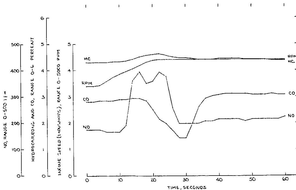
FIGURE C-17. TRANSITION BETWEEN 3400 RPM (FULL LOAD) AND 4400 RPM (FULL LOAD) FOR THE TECUMSEH AHS20 TYPE 1448 ENGINE (RUN T6P) — CONSTANT THROTTLE, DECREASING LOAD
