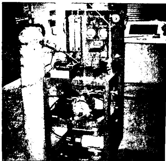
Figure 7. Experimental Dilution-Type Particulate Sampler
