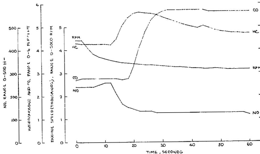
FIGURE C-18. TRANSITION BETWEEN 4500 RPM (FULL LOAD) AND 3200 RPM (NO LOAD) FOR THE TECUMSEH AH520 TYPE 1448 ENGINE (RUN 77A) — THROTTLE CLOSING, LOAD DECREASING
