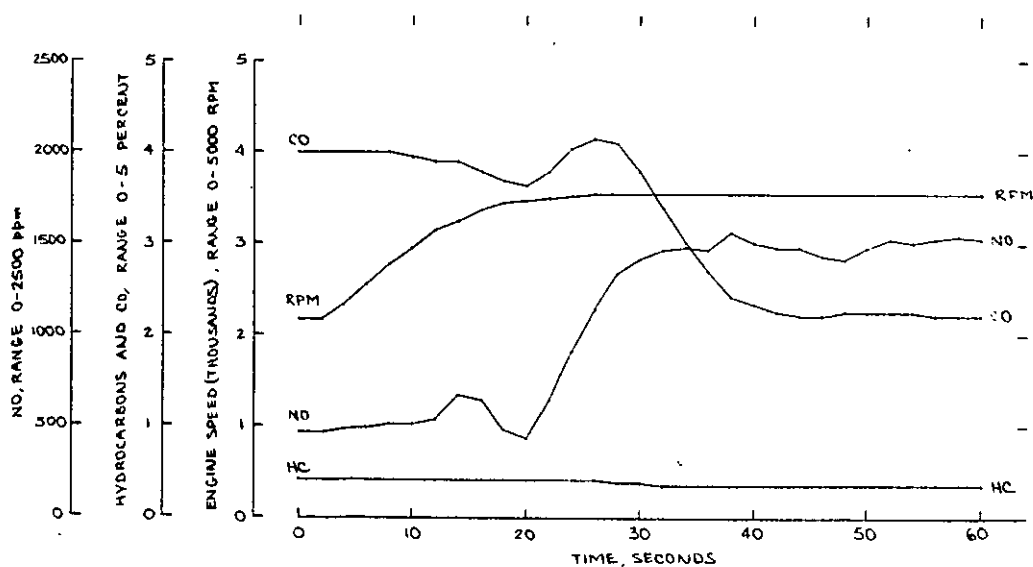
FIGURE C-6. TRANSITION BETWEEN 2200 RPM (PARTY LOAD) AND 3600 RPM (FULL LOAD) FOR THE BRIGGS & STRATTON 100202 ENGINE (RUN T6A) — CONSTANT LOAD, THROTTLE BEING OPENED
