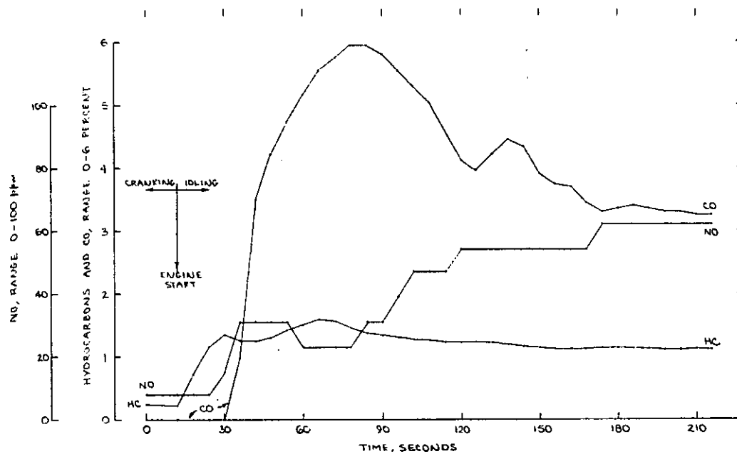
FIGURE C-20. COLD START AND IDLE FOR BRIGGS & STRATTON 9290B ENGINE, 4/30/71 (RUN CS1)
