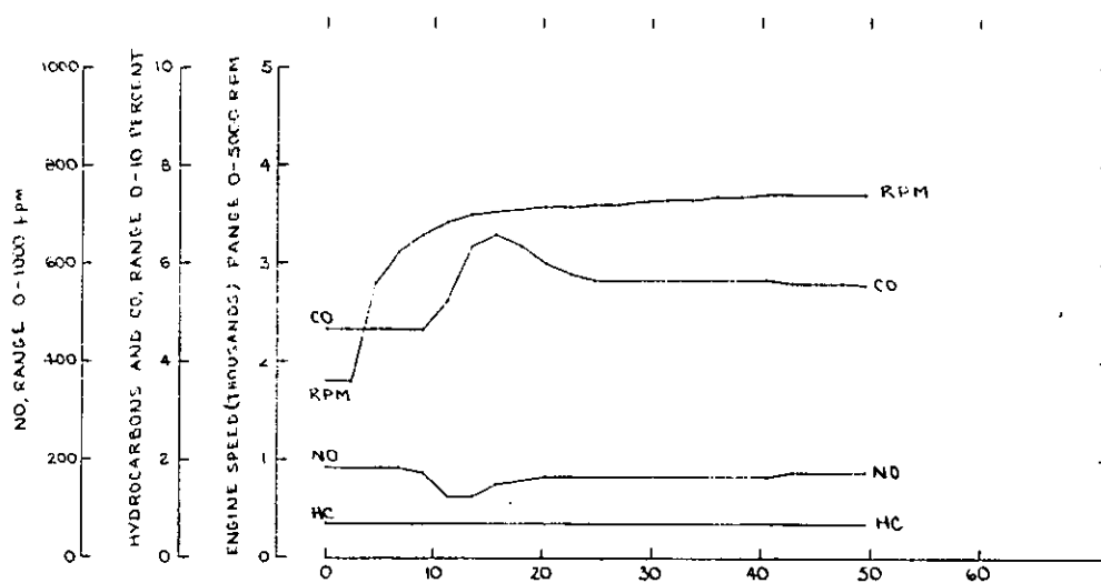
FIGURE C-13. TRANSITION BETWEEN 1800 RPM (PART LOAD) AND 3700 RPM (FULL LOAD) FOR THE KOHLER K4B2 ENGINE (RUN T9A) — CONSTANT LOAD, THROTTLE BEING OPENED
