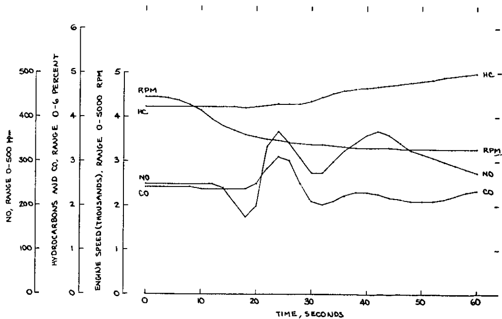
FIGURE C-15. TRANSITION BETWEEN 4500 RPM (FULL LOAD) AND 3300 RPM (FULL LOAD) FOR THE TECUMSEH AH520 TYPE 1448 ENGINE (RUN T2D) — CONSTANT THROTTLE, LOAD INCREASING
