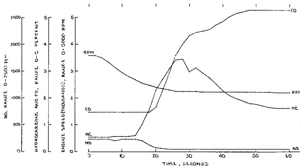
FIGURE C-1. TRANSITION BETWEEN 3600 RPM (NO LOAD) AND 2200 RPM (NO LOAD) FOR THE BRIGGS & STRATTON 100202 ENGINE (RUN T1A) — CONSTANT LOAD, THROTTLE CLOSING
