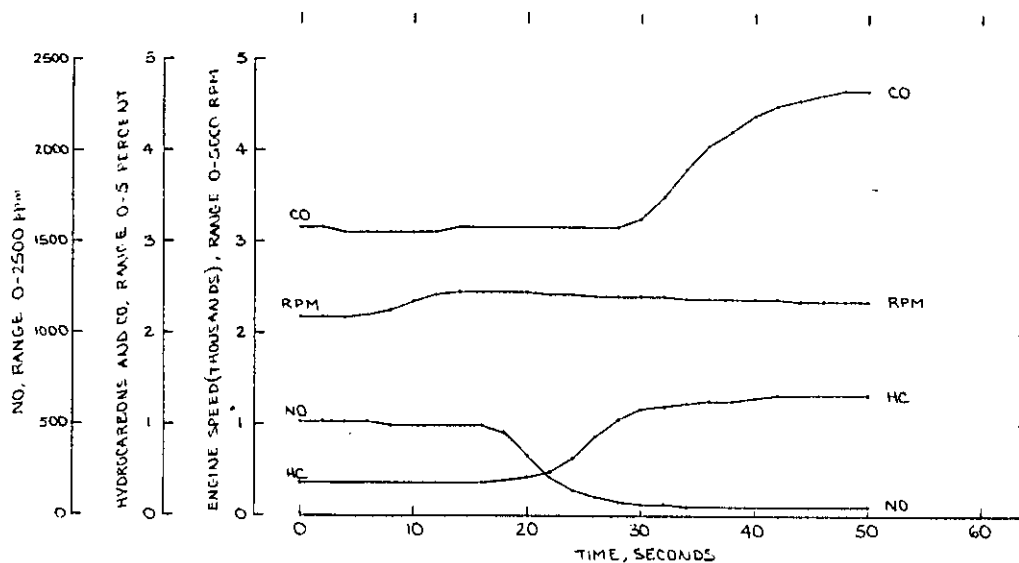
FIGURE C-5. TRANSITION BETWEEN 2200 RPM (HALF LOAD) AND 2350 RPM (NO LOAD) FOR THE BRIGGS & STRATTON 100202 ENGINE (RUN T3A) — CONSTANT THROTTLE, DECREASING LOAD (GOVERNOR CONTROLLED ENGINE SPEED DURING THIS TRANSIENT CONDITION)
