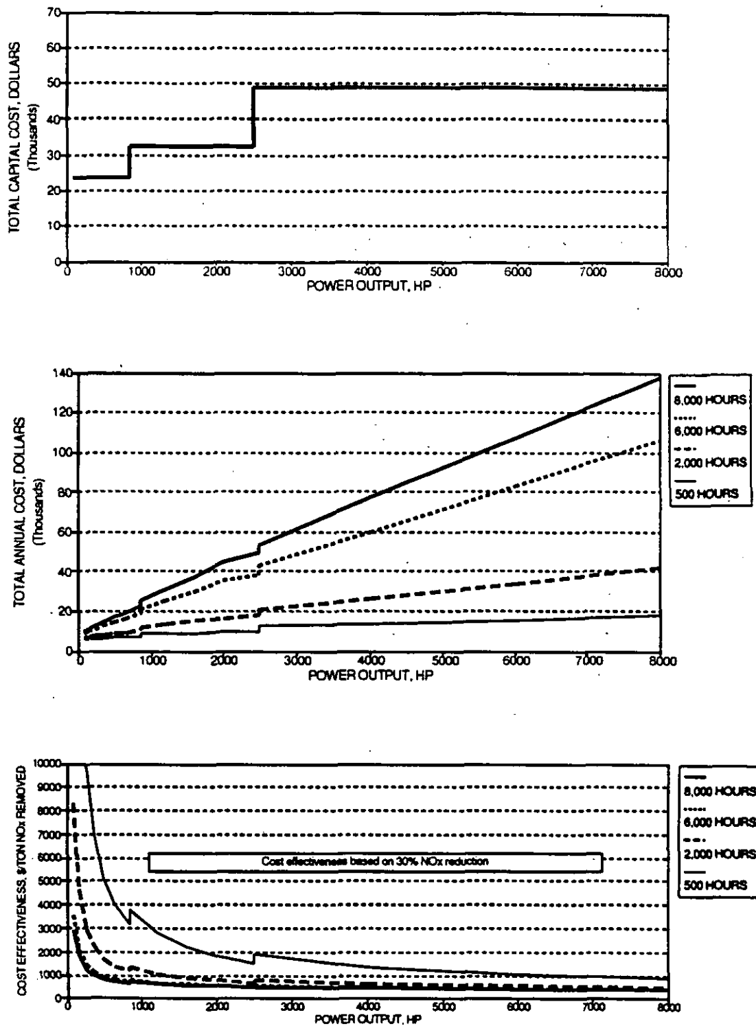
Figure 6-3. Total capital and annual costs and cost effectiveness for A/F adjustment and ignition timing retard in rich-burn engines, based on installation of automatic A/F adjustment system and controls and an electronic ignition system.
