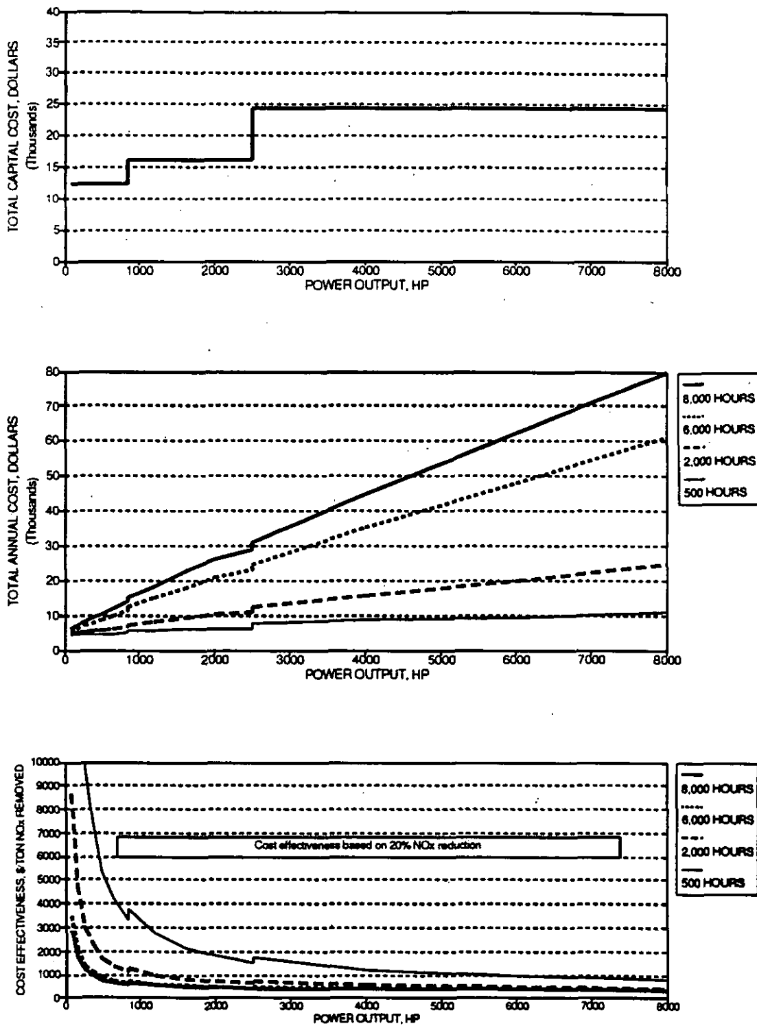
Figure 6-2. Total capital and annual costs and cost effectiveness for ignition timing retard in rich-burn engines, based on installation of an electronic ignition system.
