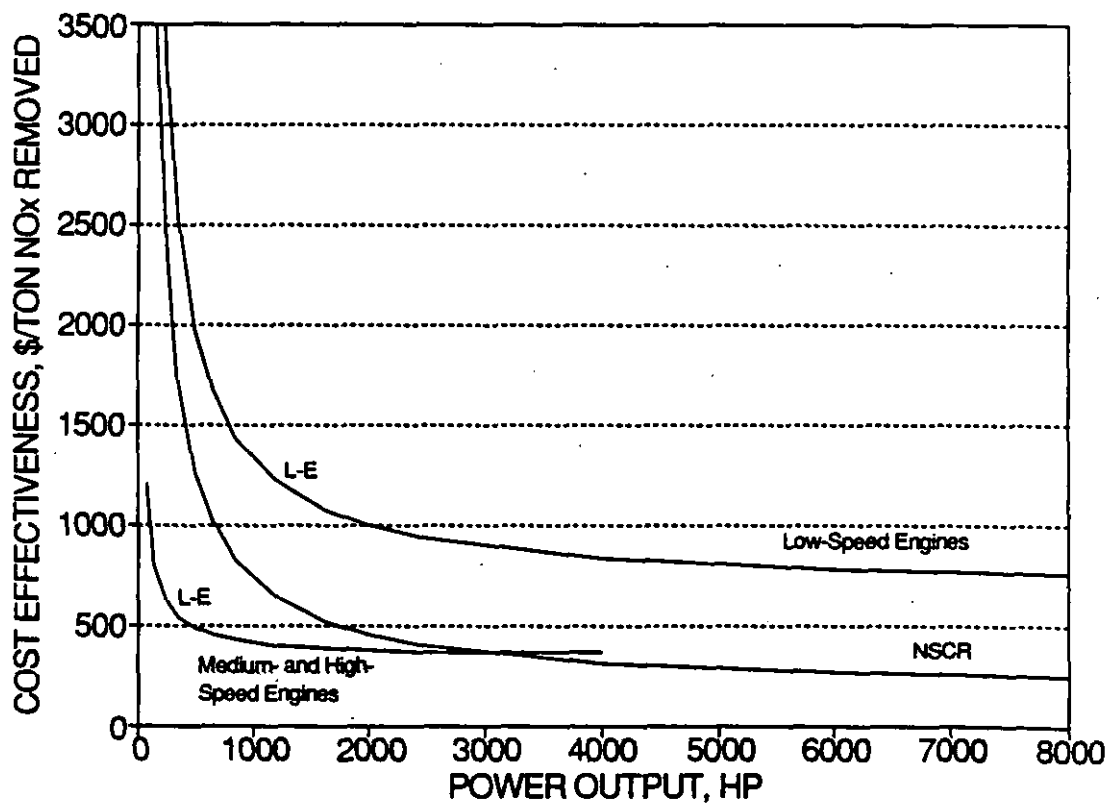
Figure 2-3. Cost effectiveness for NO x control techniques applied to rich-burn engines (8,000 hr/yr).
