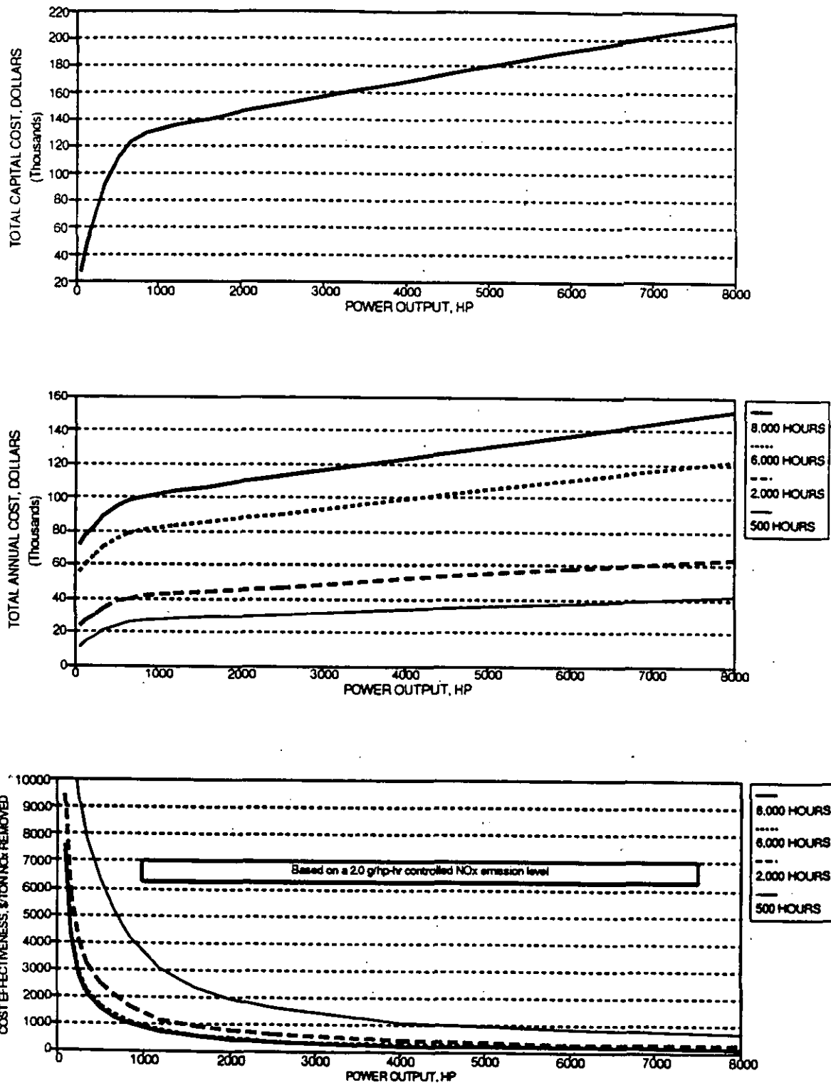
Figure 6-6. Total capital and annual costs and cost effectiveness for PSC® in rich-burn engines, with turbocharger installation or modification.
