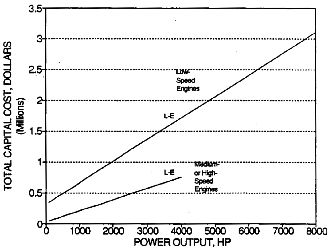
Figure 2-1. Total capital costs for NO x control techniques applied to rich-burn SI engines.
