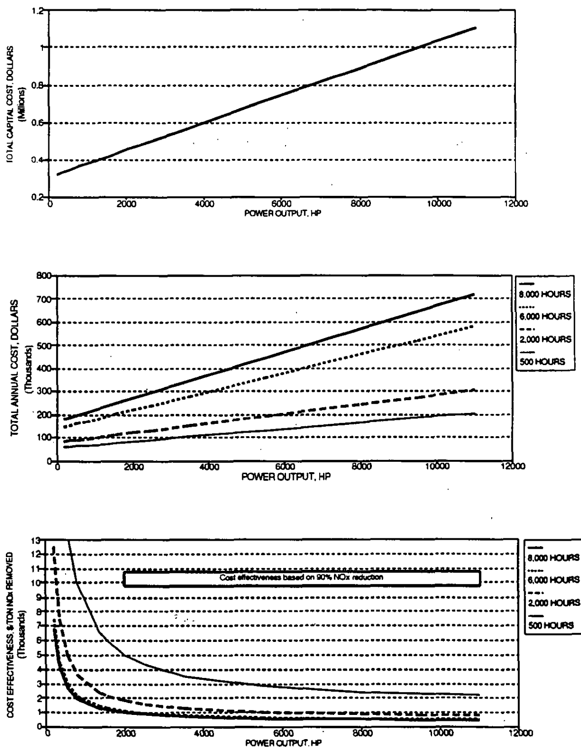
Figure 6-16. Total capital and annual costs and cost effectiveness for selective catalytic reduction for lean-burn SI engines, including a continuous emission monitoring system.
