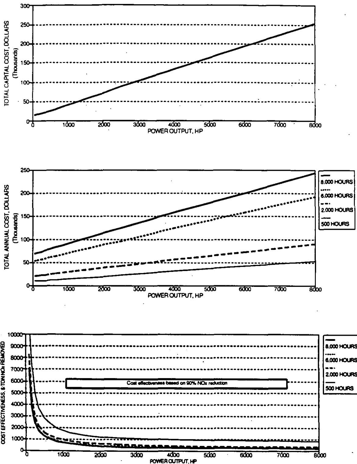
Figure 6-7. Total capital and annual costs and cost effectiveness for nonselective catalytic reduction for rich-burn engines.
