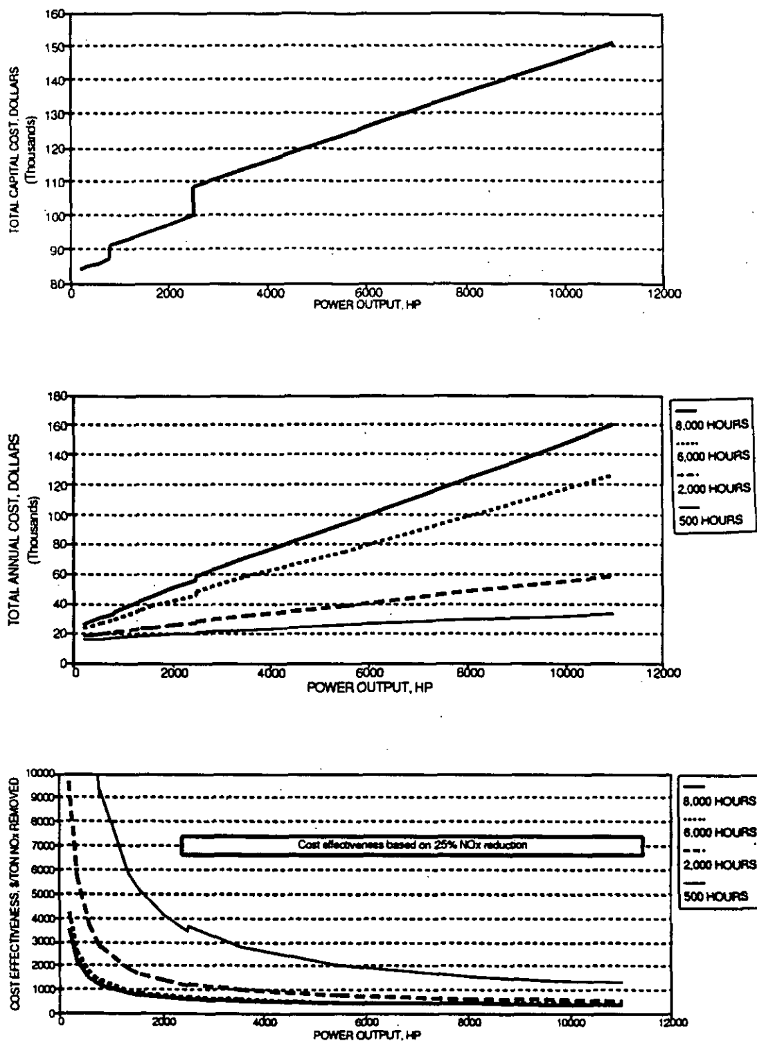
Figure 6-14. Total capital and annual costs and cost effectiveness for A/F adjustment and ignition timing retard in lean-burn SI engines, based on addition of a new turbocharger and an electronic ignition system.
