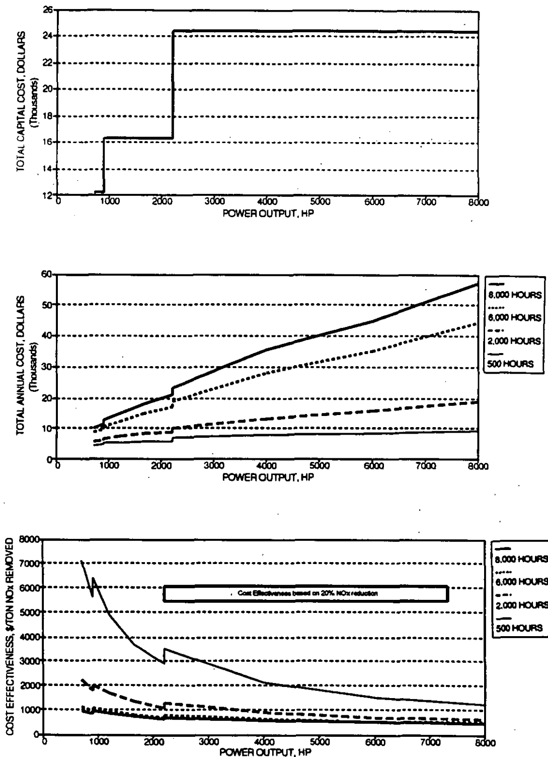
Figure 6-18. Total capital and annual costs and cost effectiveness for injection timing retard in dual-fuel engines, based on installation of an electronic ignition system.
