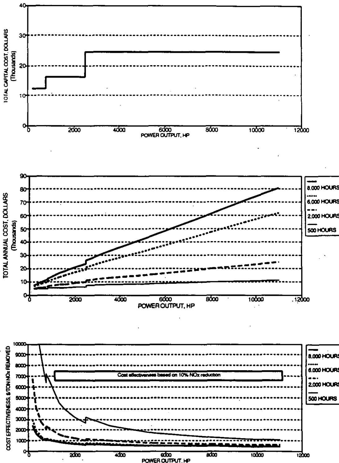
Figure 6-13. Total capital and annual costs and cost effectiveness for ignition timing retard in lean-burn SI engines, based on installation of an electronic ignition system.
