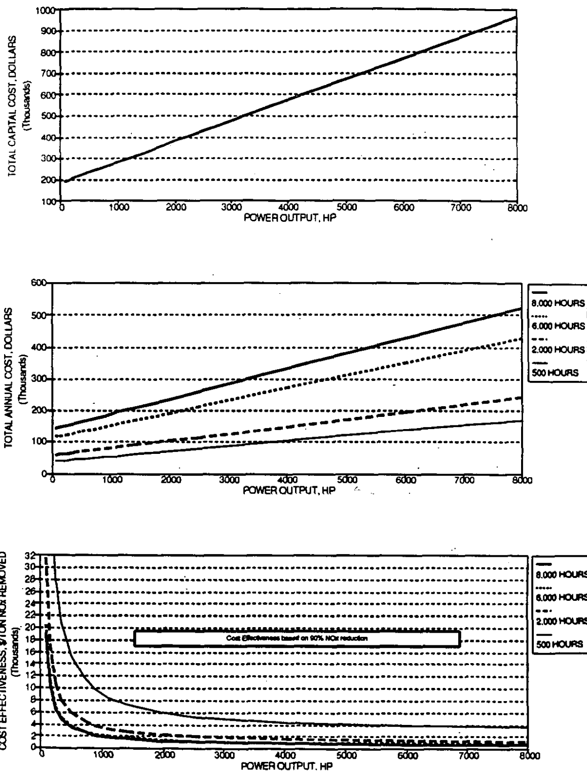
Figure 6-20. Total capital and annual costs and cost effectiveness for selective catalytic reduction for diesel engines, including a continuous emission monitoring system.
