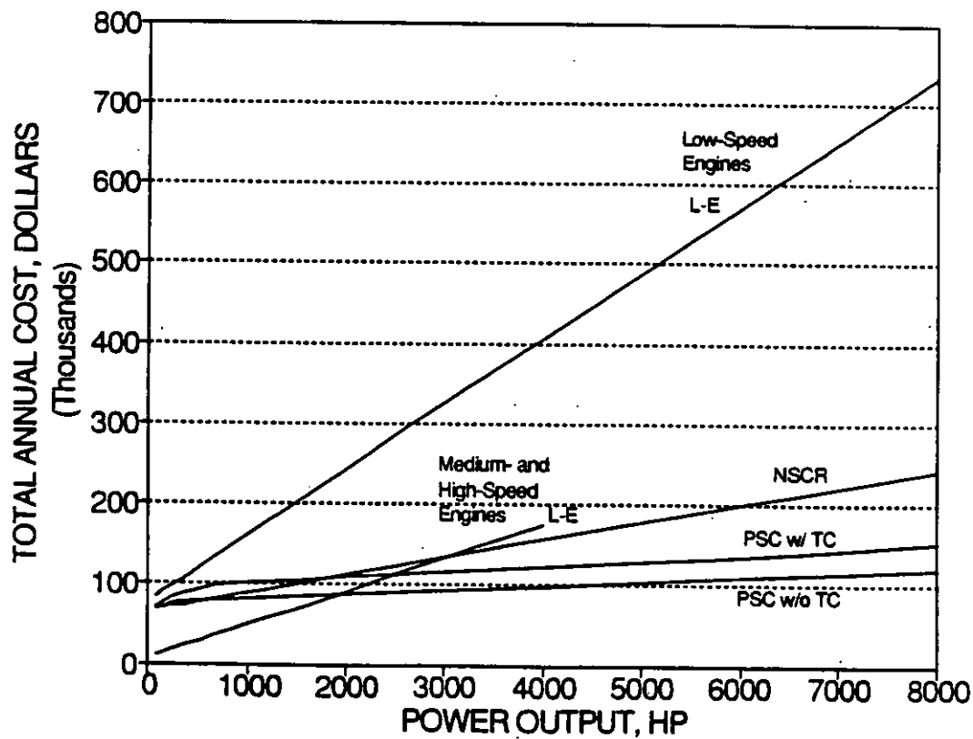
Figure 2-2. Total annual costs for NO x control techniques applied to rich-burn SI engines (8,000 hr/yr).
