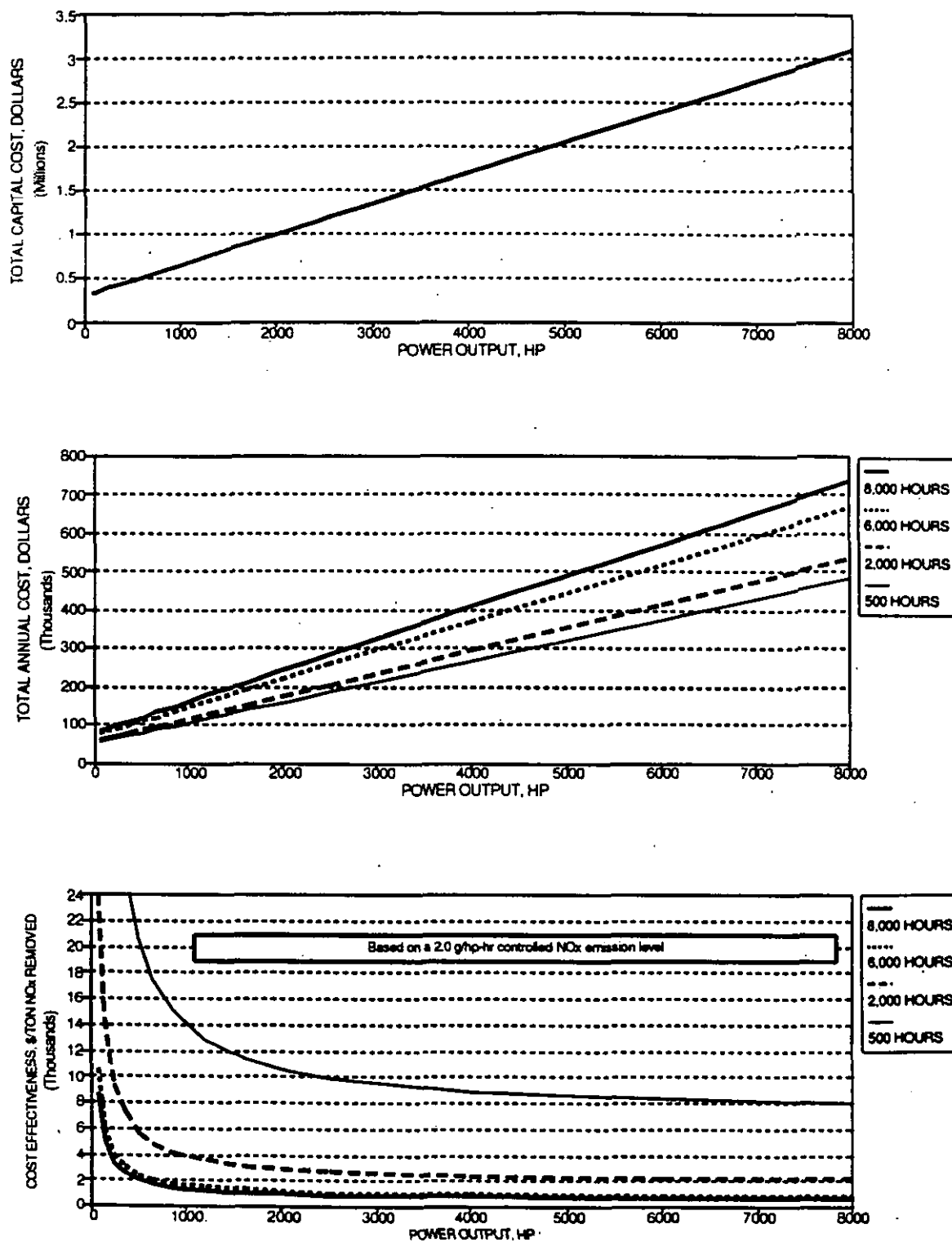
Figure 6-11. Total capital and annual costs and cost effectiveness for retrofit to low-emission combustion for low-speed engines.
