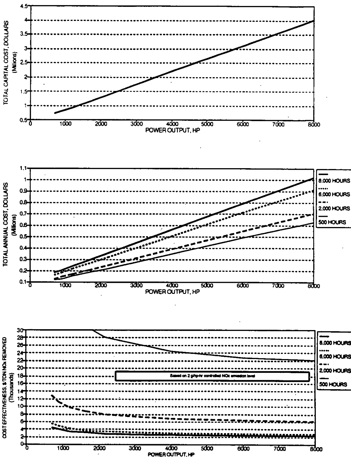
Figure 6-22. Total capital and annual costs and cost effectiveness for retrofit to low-emission combustion for dual-fuel engines.
