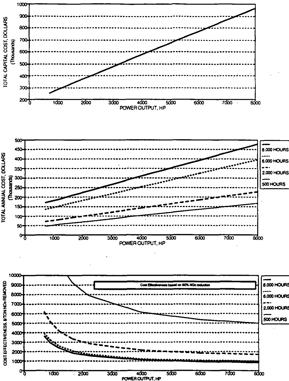
Figure 6-21. Total capital and annual costs and cost effectiveness for selective catalytic reduction for dual-fuel engines, including a continuous emission monitoring system.
