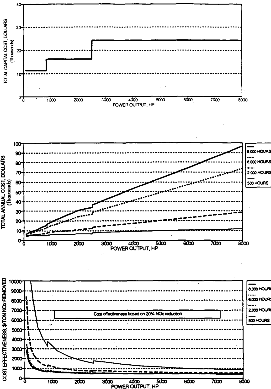
Figure 6-1. Total capital and annual costs and cost effectiveness for A/F adjustment in rich-burn engines, based on installation of an automatic A/F adjustment system and controls.
