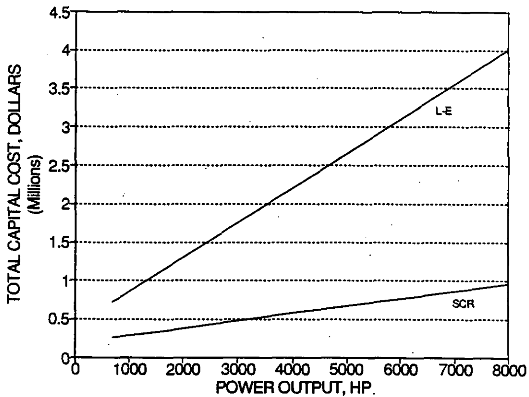
Figure 2-10. Total capital costs for NO x control techniques applied to dual-fuel engines.
