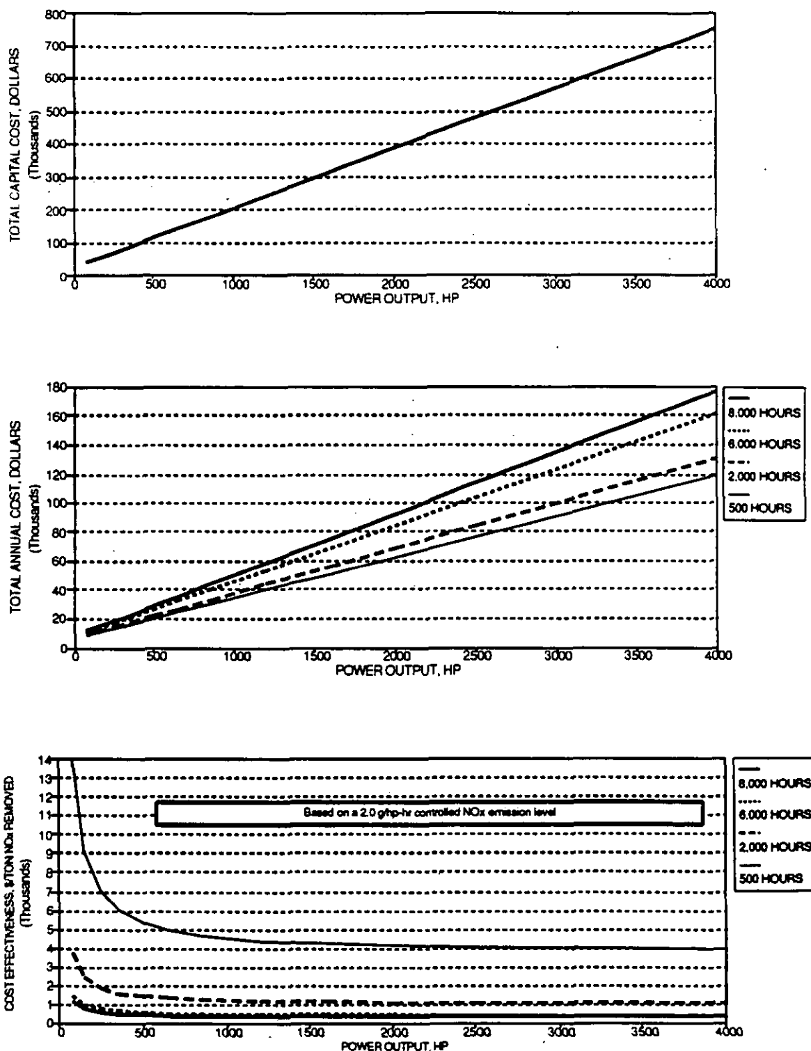
Figure 6-10. Total capital and annual costs and cost effectiveness for retrofit to low-emission combustion for medium-speed engines.
