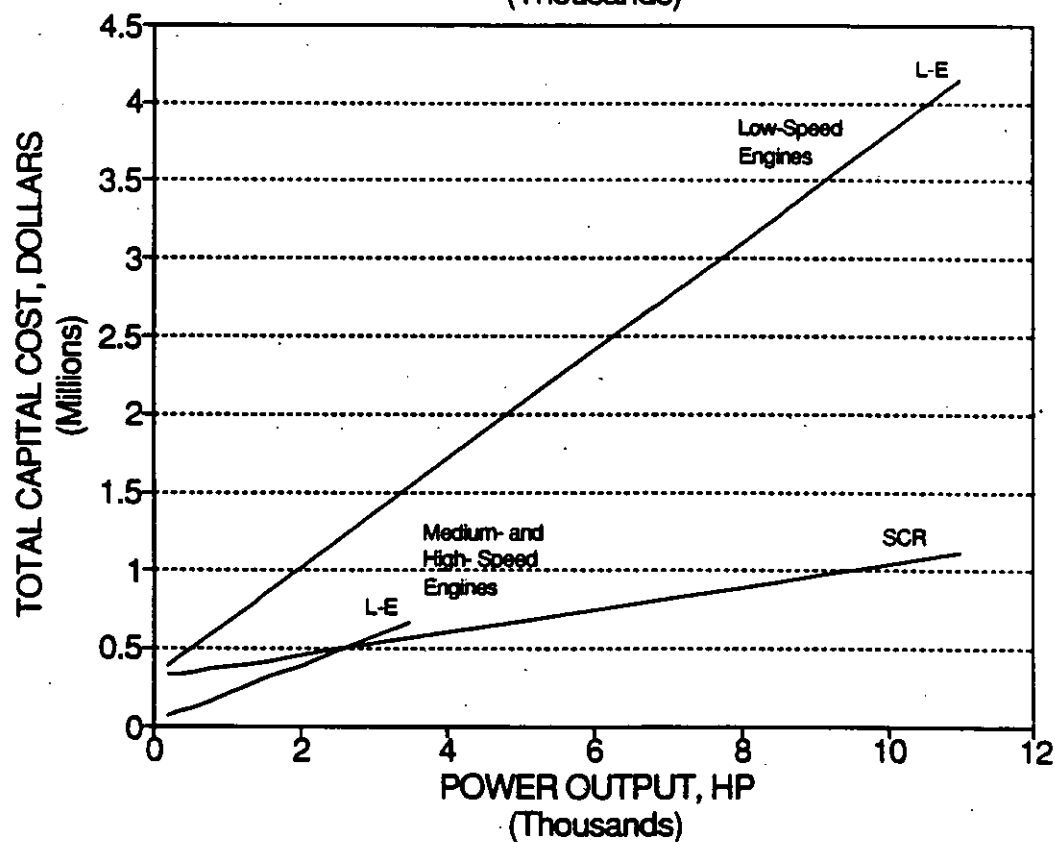
Figure 2-4. Total capital costs for NO x control techniques applied to lean-burn SI engines.
