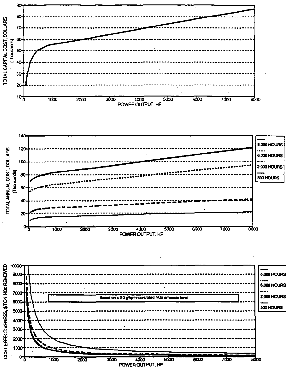
Figure 6-5. Total capital and annual costs and cost effectiveness for PSC ® in rich-burn engines, without turbocharger installation or modification.
