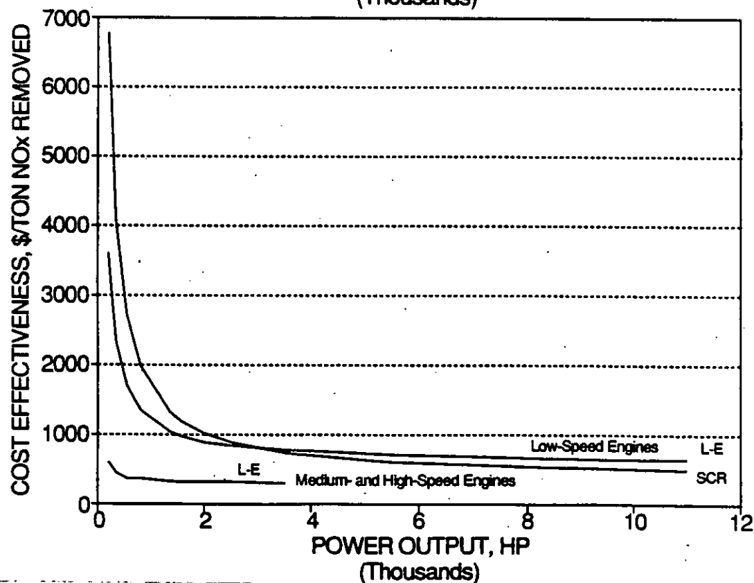
Figure 2-6. Cost effectiveness for NO x control techniques applied to lean-burn SI engines (8,000 hr/yr).
