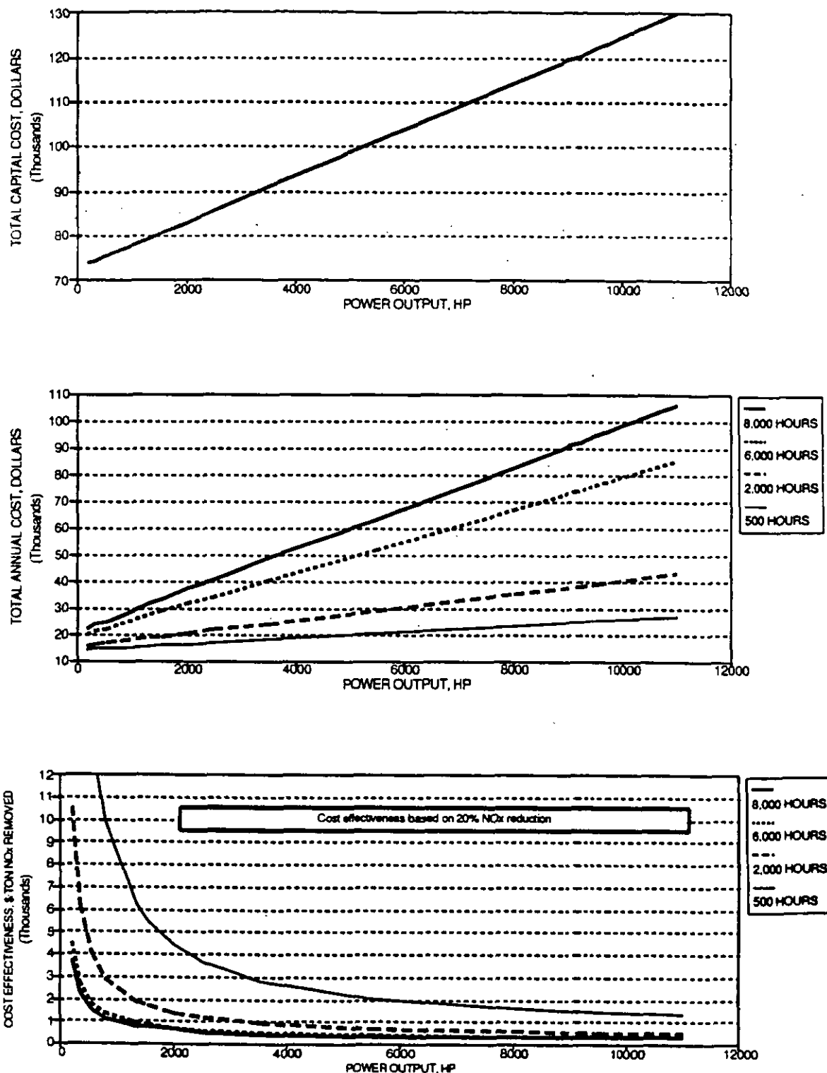
Figure 6-12. Total capital and annual costs and cost effectiveness for A/F adjustment in lean-burn engines, based on the addition of a new turbocharger to the existing engine.
