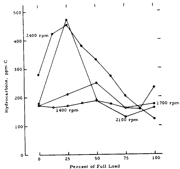
FIGURE A-6. HYDROCARBON EMISSIONS FROM A MERCEDES-BENZ OM636 ENGINE AS A FUNCTION OF LOAD AT FOUR SPEEDS
