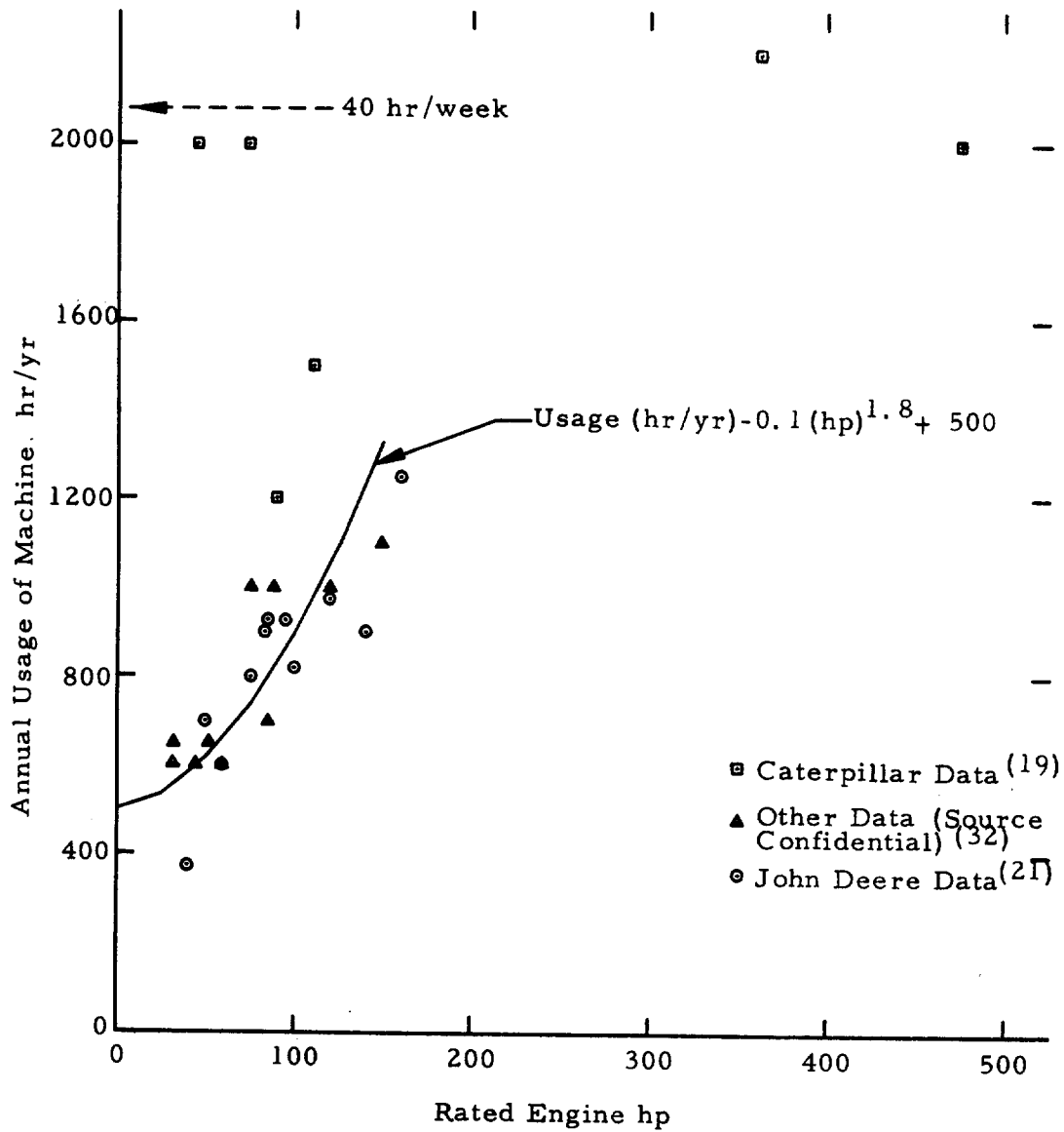
FIGURE 23. USAGE AS A FUNCTION OF RATED ENGINE HP FOR VARIOUS CATEGORIES OF CONSTRUCTION EQUIPMENT
