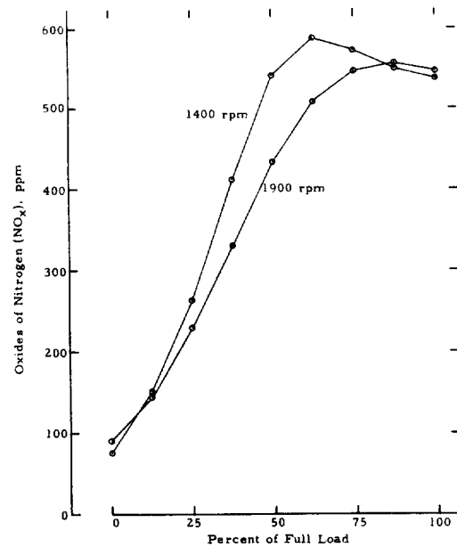
FIGURE A-18. OXIDES OF NITROGEN EMISSIONS FROM A CATERPILLAR D6C ENGINE AS A FUNCTION OF LOAD AT TWO SPEEDS
