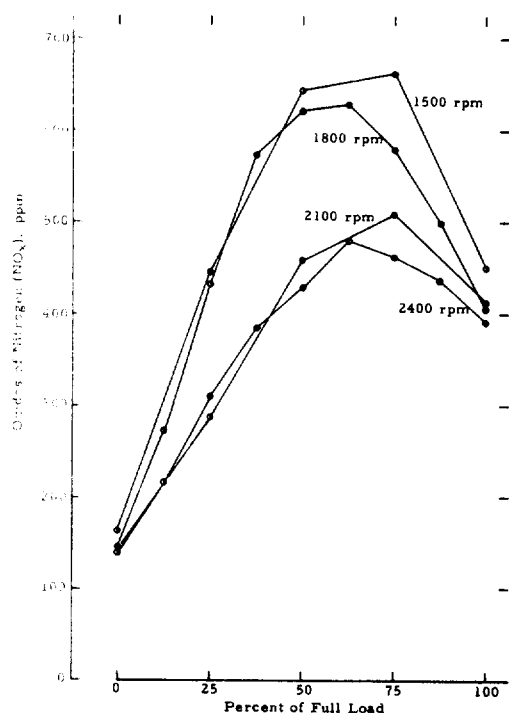
FIGURE A-23. OXIDES OF NITROGEN EMISSIONS FROM AN ONAN 6JBA ENGINE AS A FUNCTION OF LOAD AT FOUR SPEEDS
