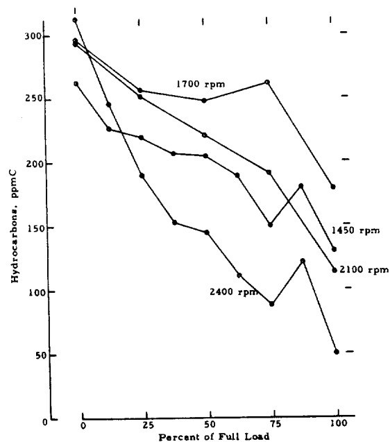
FIGURE A-8. HYDROCARBON EMISSIONS FROM A PERKINS 4.236 ENGINE AS A FUNCTION OF LOAD AT FOUR SPEEDS
