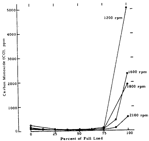
FIGURE A-11. CARBON MONOXIDE EMISSIONS FROM A DETROIT DIESEL 6V-71 ENGINE AS A FUNCTION OF LOAD AT FOUR SPEEDS
