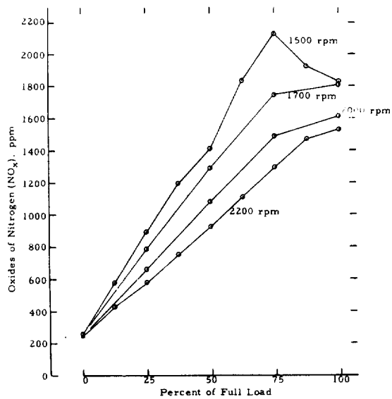
FIGURE A-17. OXIDES OF NITROGEN EMISSIONS FROM AN ALLIS-CHALMERS 3500 ENGINE AS A FUNCTION OF LOAD AT FOUR SPEEDS
