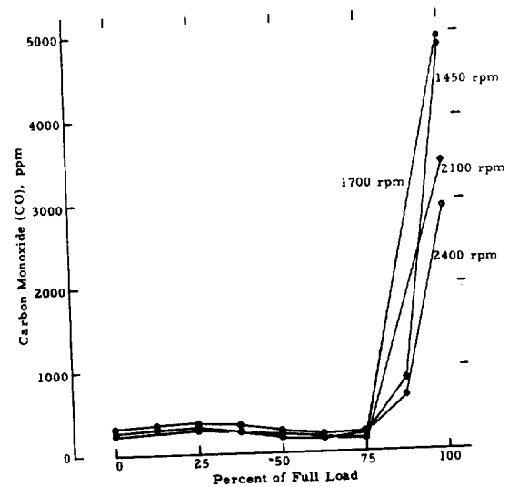
FIGURE A-16. CARBON MONOXIDE EMISSIONS FROM A PERKINS 4.236 ENGINE AS A FUNCTION OF LOAD AT FOUR SPEEDS
