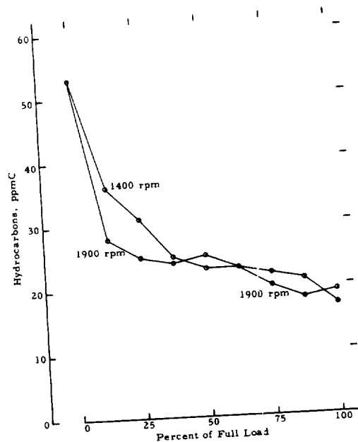
FIGURE A-2. HYDROCARBON EMISSIONS FROM A CATERPILLAR D6C ENGINE AS A FUNCTION OF LOAD AT TWO SPEEDS
