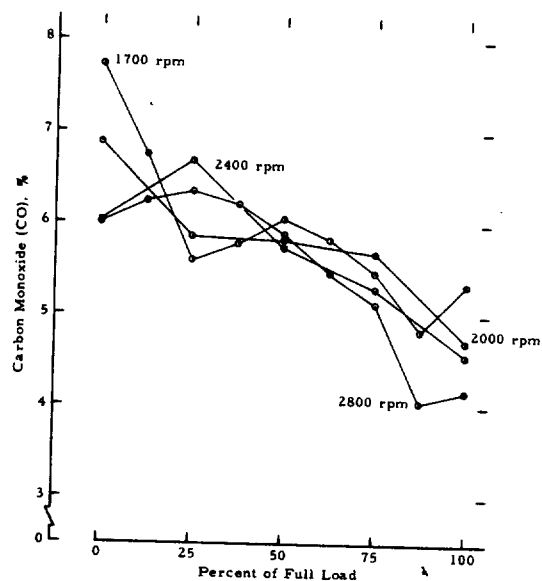
FIGURE E-8. CARBON MONOXIDE EMISSIONS FROM A WISCONSIN V4D ENGINE AS A FUNCTION OF LOAD AT FOUR SPEEDS
