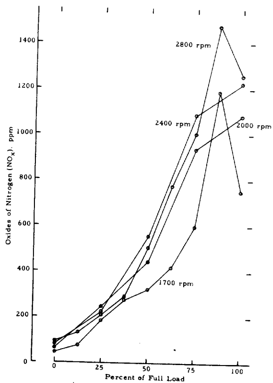
FIGURE E-12. OXIDES OF NITROGEN EMISSIONS FROM A WISCONSIN V44D ENGINE AS A FUNCTION OF LOAD AT FOUR SPEEDS
