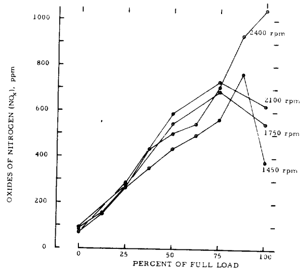
FIGURE E-10. OXIDES OF NITROGEN EMISSIONS FROM A HERCULES G-2300 ENGINE AS A FUNCTION OF LOAD AT FOUR SPEEDS
