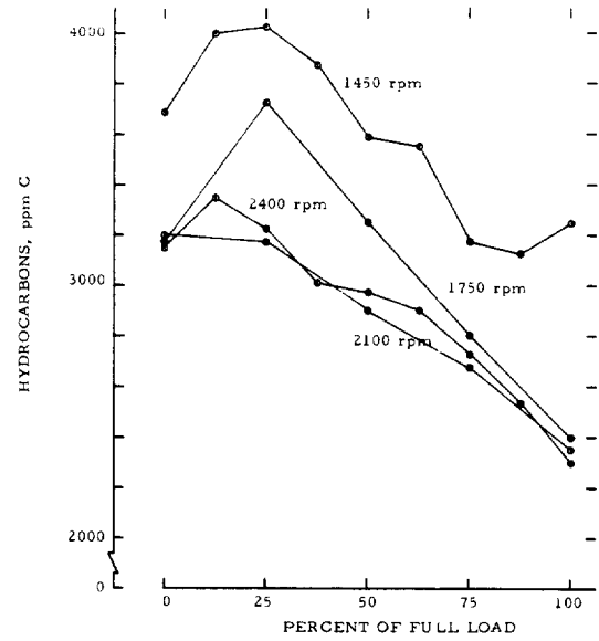
FIGURE E-2. HYDROCARBON EMISSIONS FROM A HERCULES G-2300 ENGINE AS A FUNCTION OF LOAD AT FOUR SPEEDS
