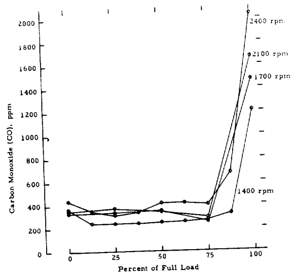
FIGURE A-14. CARBON MONOXIDE EMISSIONS FROM A MERCEDES-BENZ OM636 ENGINE AS A FUNCTION OF LOAD AT FOUR SPEEDS
