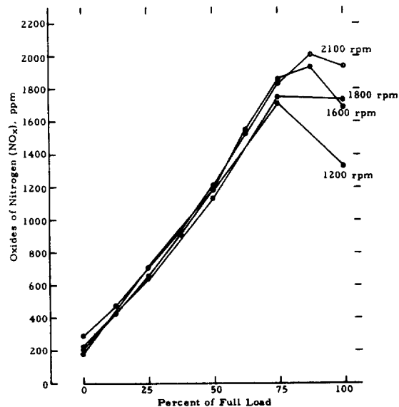
FIGURE A-19. OXIDES OF NITROGEN EMISSIONS FROM A DETROIT DIESEL 6V-71 ENGINE AS A FUNCTION OF LOAD AT FOUR SPEEDS
