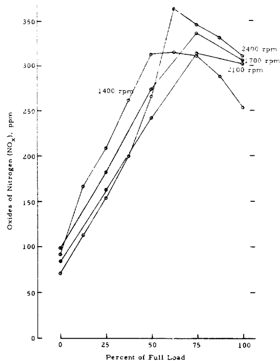
FIGURE A-22. OXIDES OF NITROGEN EMISSIONS FROM A MERCEDES-BENZ OM636 ENGINE AS A FUNCTION OF LOAD AT FOUR SPEEDS
