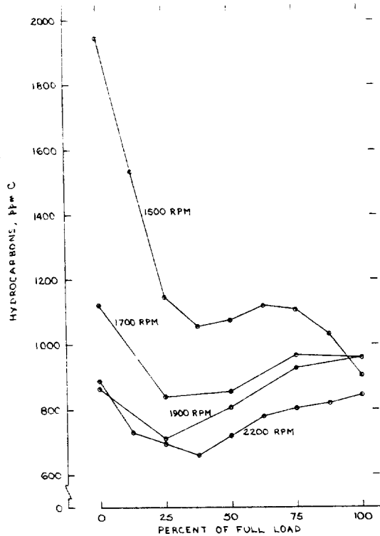
FIGURE A-5. HYDROCARBON EMISSIONS FROM A JOHN DEERE 6404 ENGINE AS A FUNCTION OF LOAD AT FOUR SPEEDS
