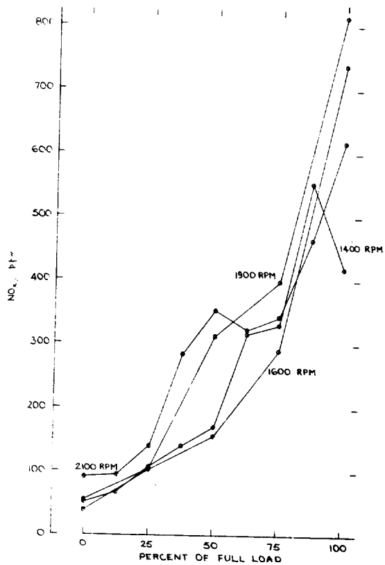
FIGURE E-11. OXIDES OF NITROGEN EMISSIONS FROM A J.I. CASE 159 G ENGINE AS A FUNCTION OF LOAD AT FOUR SPEEDS
