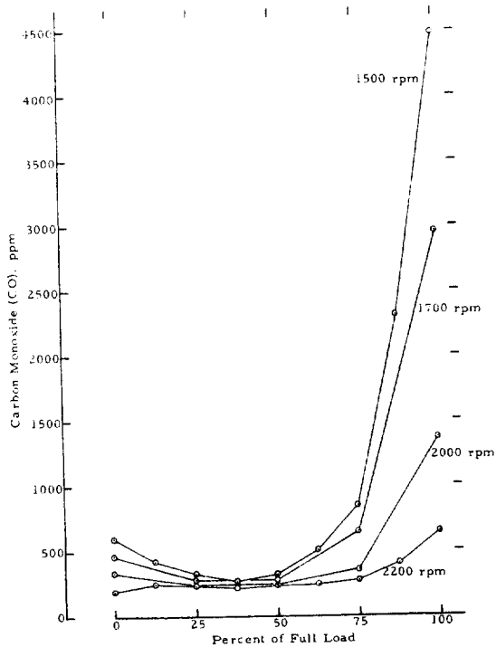
FIGURE A-9. CARBON MONOXIDE EMISSIONS FROM AN ALLIS-CHALMERS 3500 ENGINE AS A FUNCTION OF LOAD AT FOUR SPEEDS
