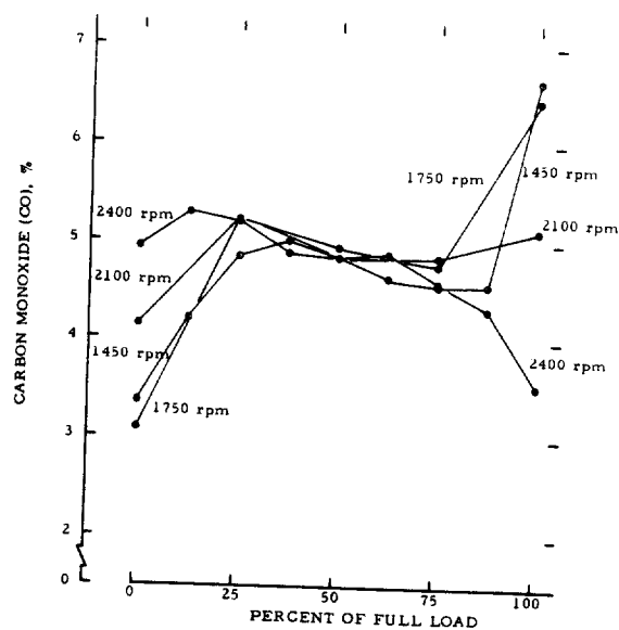
FIGURE E-6. CARBON MONOXIDE EMISSIONS FROM A HERCULES G-2300 ENGINE AS A FUNCTION OF LOAD AT FOUR SPEEDS
