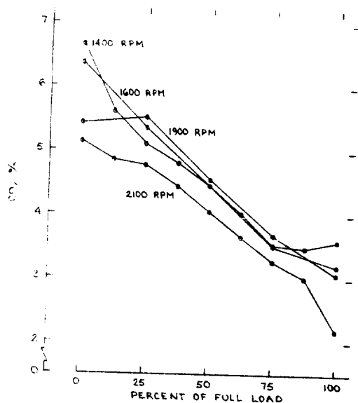
FIGURE E-5. CARBON MONOXIDE EMISSIONS FROM A FORD G-5000 ENGINE AS A FUNCTION OF LOAD AT FOUR SPEEDS
