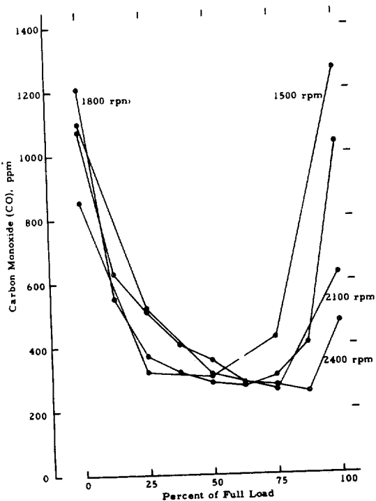
FIGURE A-15. CARBON MONOXIDE EMISSIONS FROM AN ONAN DJBA ENGINE AS A FUNCTION OF LOAD AT FOUR SPEEDS
