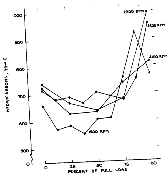
FIGURE A-4. HYDROCARBON EMISSIONS FROM AN INTERNATIONAL HARVESTER D407 ENGINE AS A FUNCTION OF LOAD AT FOUR SPEEDS
