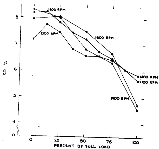
FIGURE E-7. CARBON MONOXIDE EMISSIONS FROM A J.I. CASE 159 G ENGINE AS A FUNCTION OF LOAD AT FOUR SPEEDS
