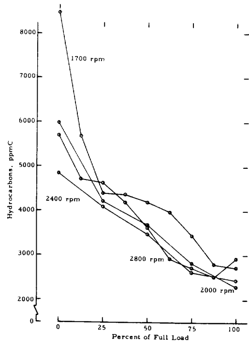
FIGURE E-4. HYDROCARBON EMISSIONS FROM A WISCONSIN VH4D ENGINE AS A FUNCTION OF LOAD AT FOUR SPEEDS
