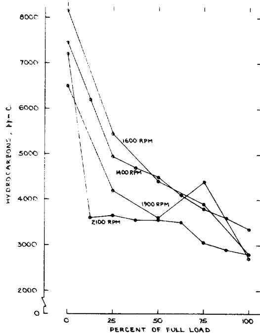
FIGURE E-3. HYDROCARBON EMISSIONS FROM A J.I. CASE 159G ENGINE AS A FUNCTION OF LOAD AT FOUR SPEEDS
