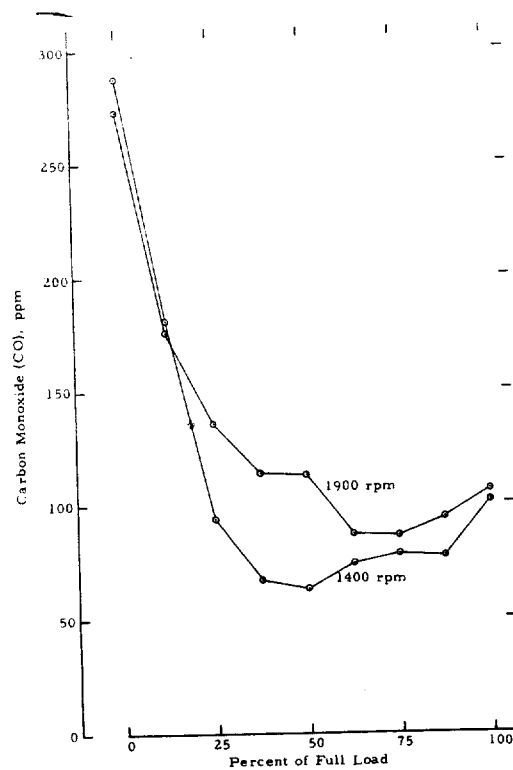
FIGURE A-10. CARBON MONOXIDE EMISSIONS FROM A CATERPILLAR D6C ENGINE AS A FUNCTION OF LOAD AT TWO SPEEDS
