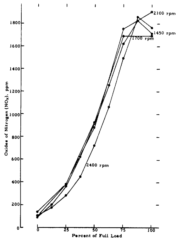
FIGURE A-24. OXIDES OF NITROGEN EMISSIONS FROM A PERKINS 4.236 ENGINE AS A FUNCTION OF LOAD AT FOUR SPEEDS
