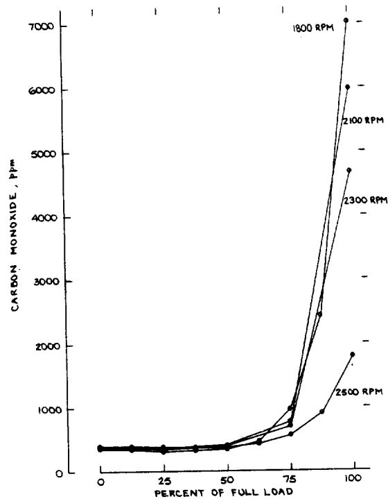
FIGURE A-12. CARBON MONOXIDE EMISSIONS FROM AN INTERNATIONAL HARVESTER D407 ENGINE AS A FUNCTION OF LOAD AT FOUR SPEEDS
