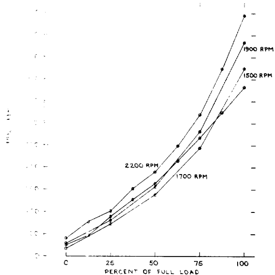
FIGURE A-21. OXIDES OF NITROGEN EMISSIONS FROM A JOHN DEERE 6404 ENGINE AS A FUNCTION OF LOAD AT FOUR SPEEDS
