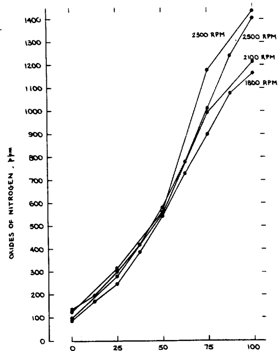
FIGURE A-20. OXIDES OF NITROGEN EMISSIONS FROM AN INTERNATIONAL HARVESTER D407 ENGINE AS A FUNCTION OF LOAD AT FOUR SPEEDS
