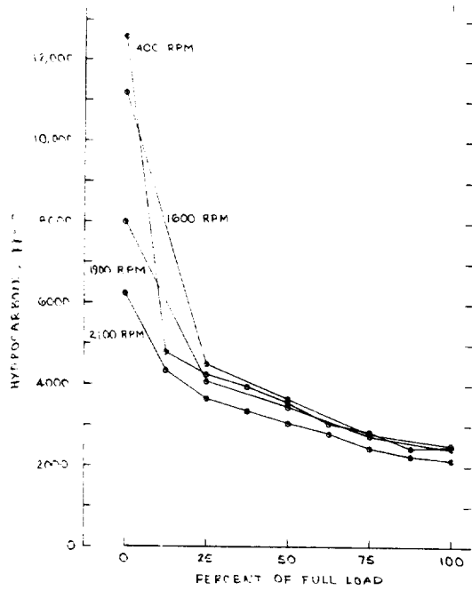
FIGURE E-1. HYDROCARBON EMISSIONS FROM A FORD G-5000 ENGINE AS A FUNCTION OF LOAD AT FOUR SPEEDS
