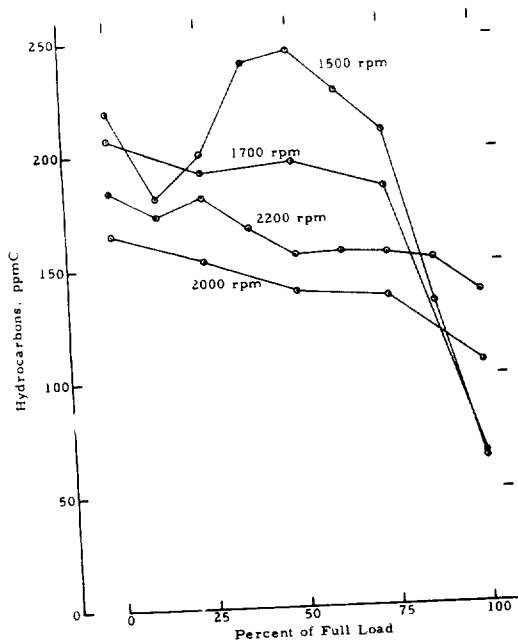
FIGURE A-1. HYDROCARBON EMISSIONS FROM AN ALLIS-CHALMERS 3500 ENGINE AS A FUNCTION OF LOAD AT FOUR SPEEDS
