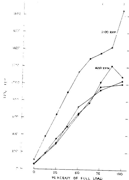
FIGURE E-9. OXIDES OF NITROGEN EMISSIONS FROM A FORD 9500 V8 ENGINE AS A FUNCTION OF LOAD AT FOUR SPEEDS
