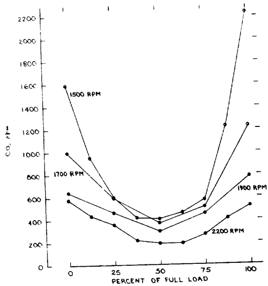
FIGURE A-13. CARBON MONOXIDE EMISSIONS FROM A JOHN DEERE 6404 ENGINE AS A FUNCTION OF LOAD AT FOUR SPEEDS
