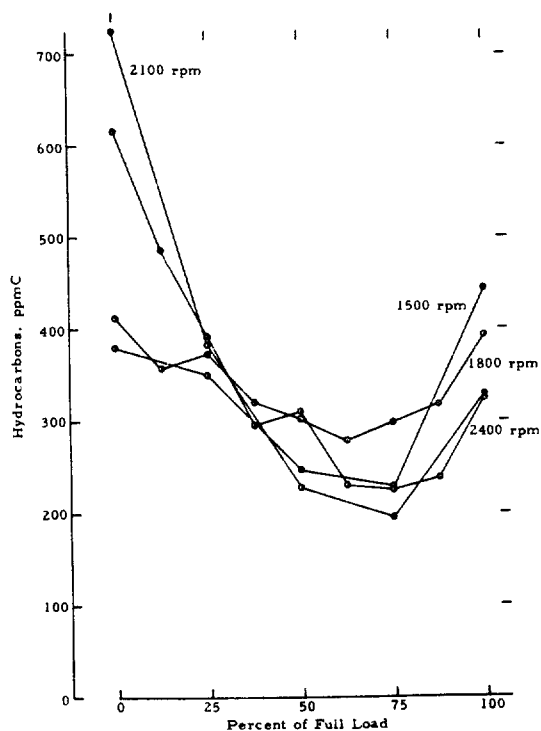
FIGURE A-7. HYDROCARBON EMISSIONS FROM AN ONAN DJBA ENGINE AS A FUNCTION OF LOAD AT FOUR SPEEDS
