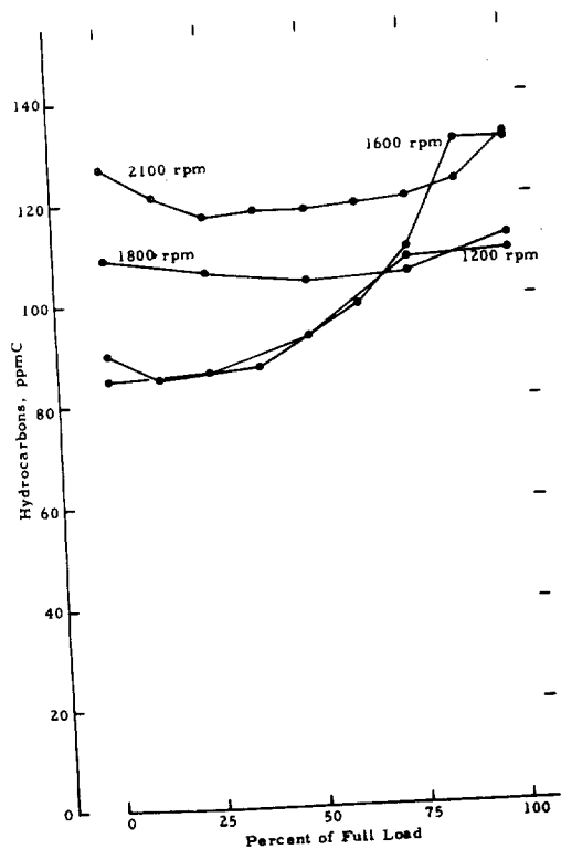
FIGURE A-3. HYDROCARBON EMISSIONS FROM A DETROIT DIESEL 6V-71 ENGINE AS A FUNCTION OF LOAD AT FOUR SPEEDS
