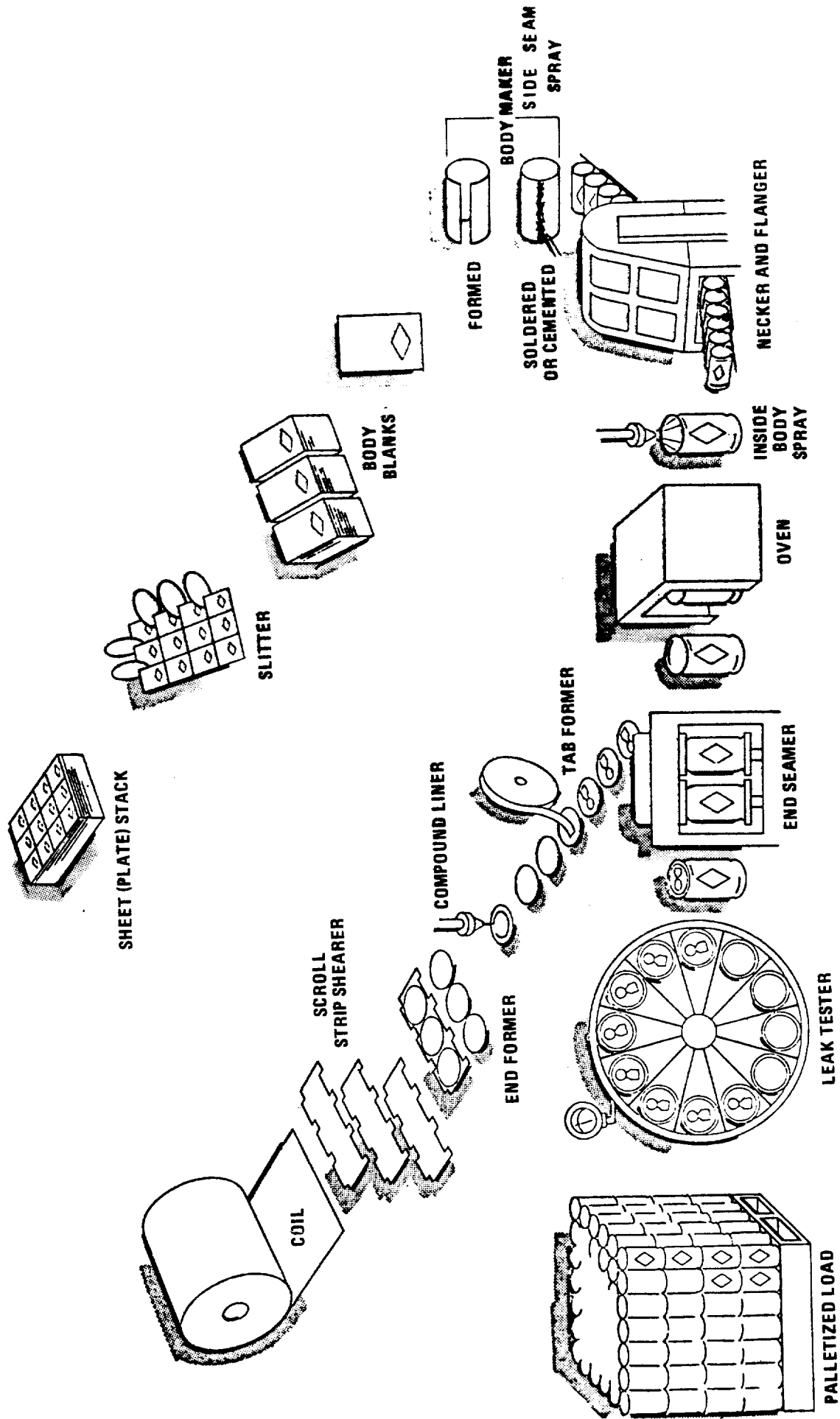
Figure 2-4. Can end, and three-piece beer and beverage can fabricating operation.
