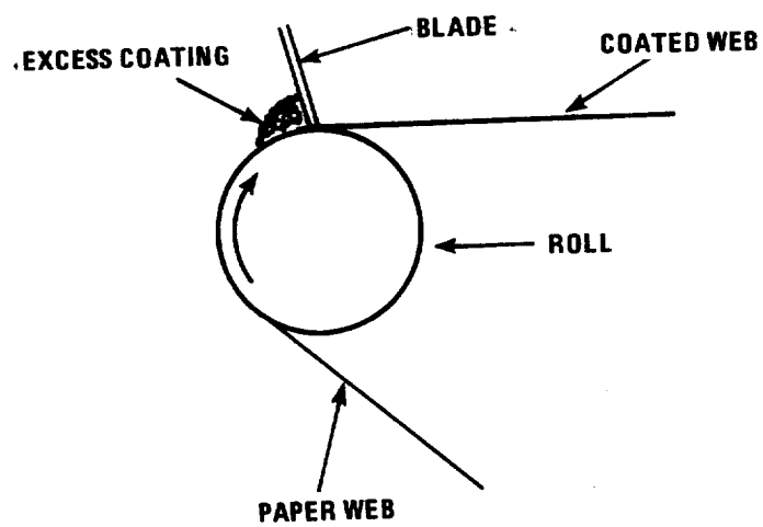
Figure 5-2. Knife coating of paper.
