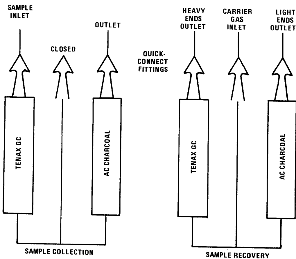
Figure 5-2. Schematic diagram of universal collector. 8
