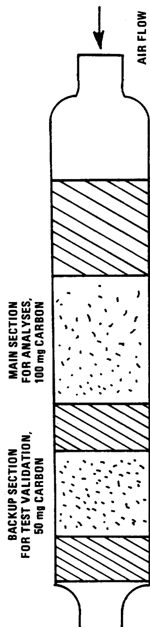
Figure 5-1. Carbon-filled tube employed to trap solvent vapors. 7
