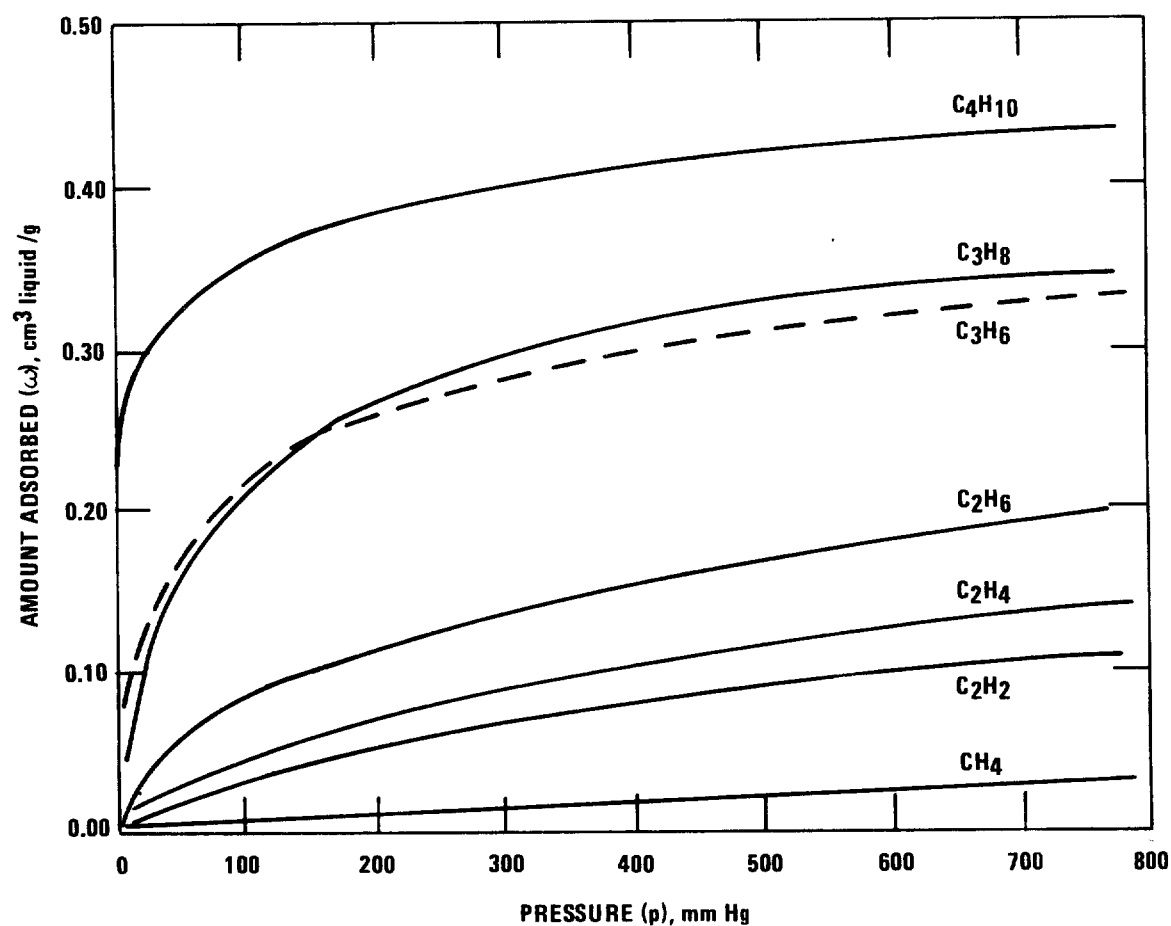
Figure 3-1. Adsorption isotherms of hydrocarbon vapors (amount adsorbed, \omega , at pressure, p , on type Columbia L carbon at 100°F, liquid volume of \omega at boiling temperature). 1
