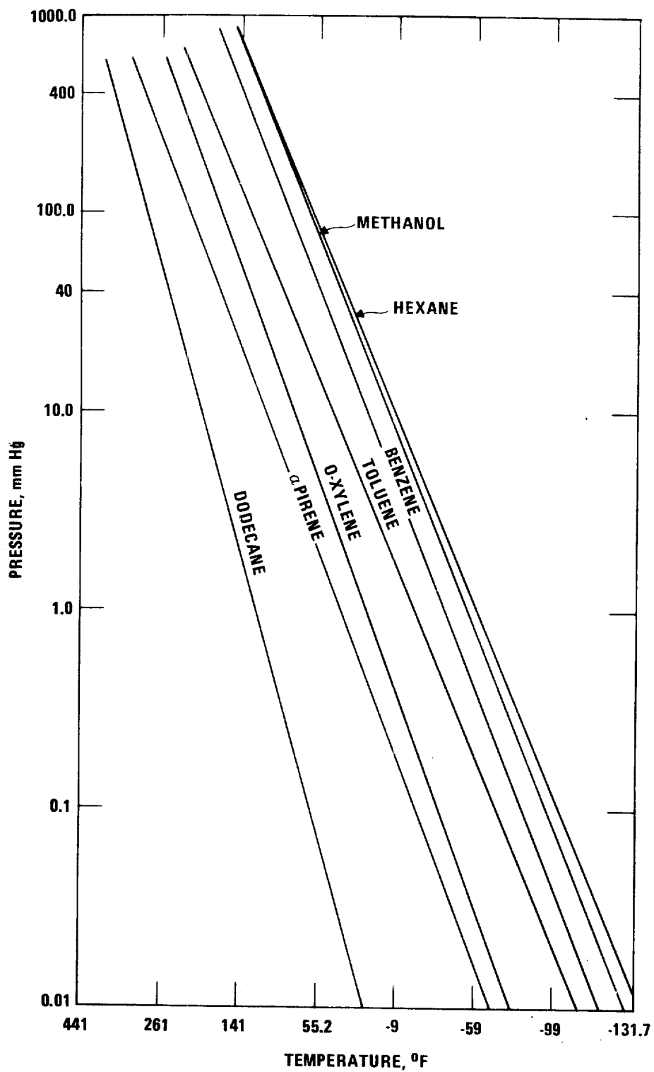
Figure 3-17. Vapor pressures of organic solvents versus temperature.
