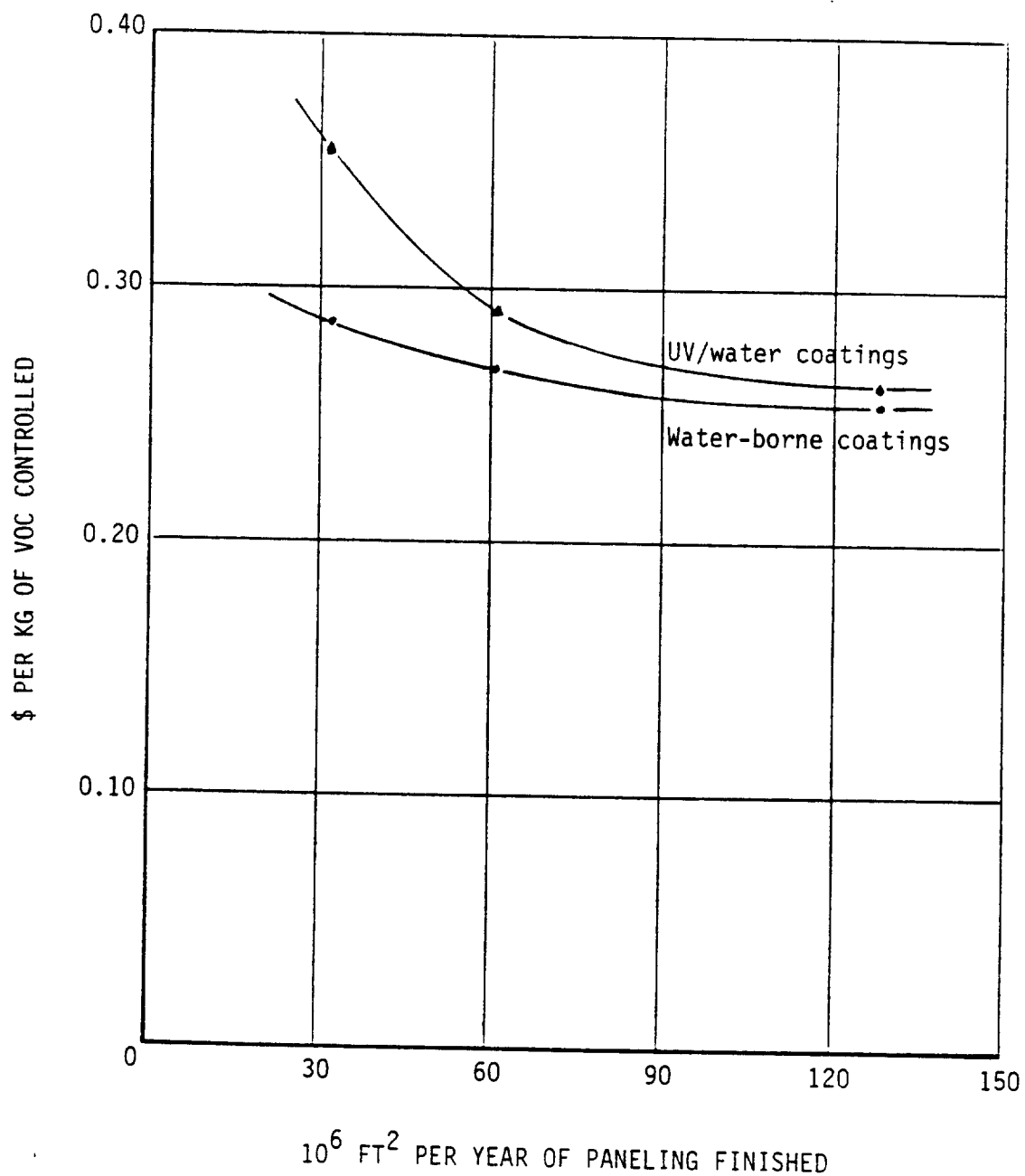
Figure 3-1. Cost Effectiveness for VOC Control at Existing Printed Panel Coating Plants
