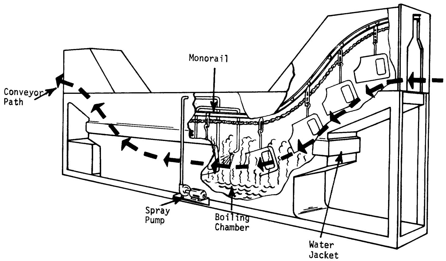
Figure 2-11 MONORAIL CONVEYORIZED DEGREASER
