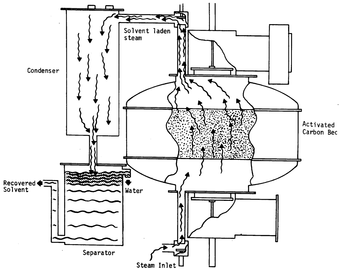
Figure 3-4 DESORPTION CYCLE
