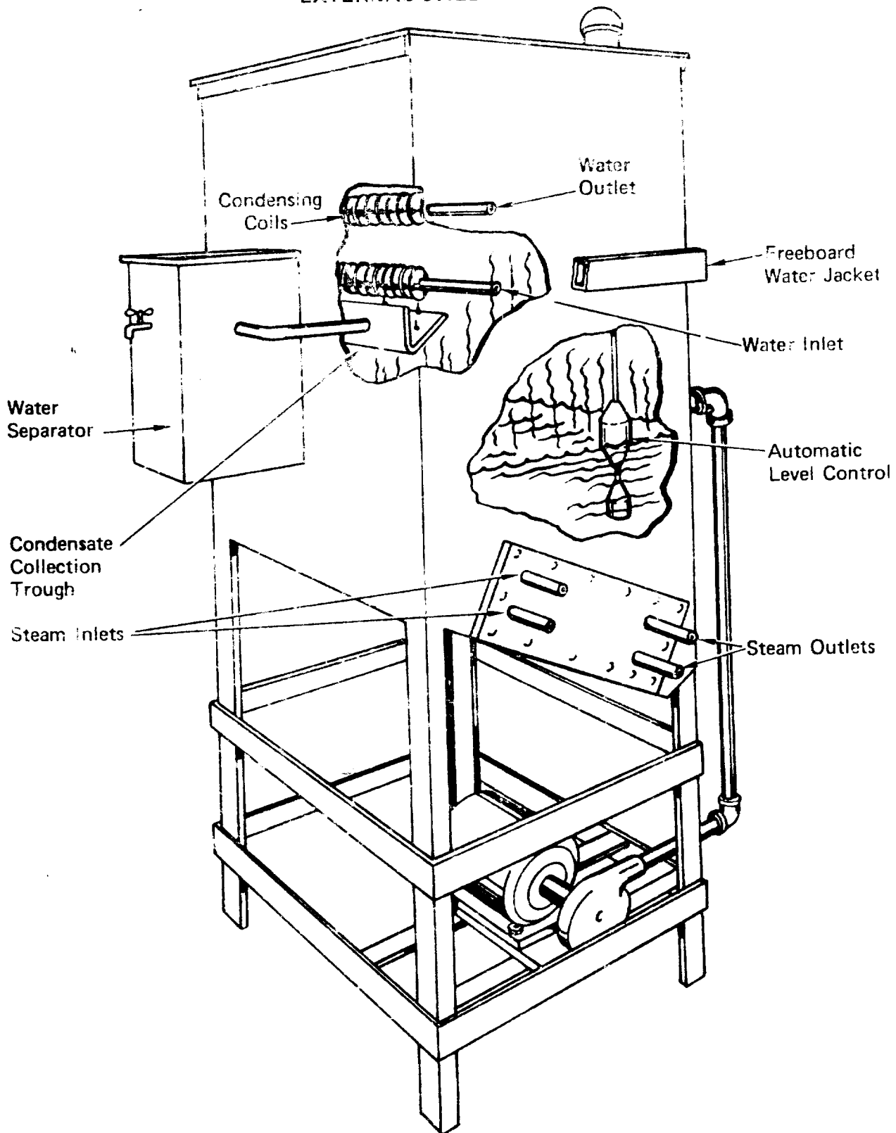
Figure 3-7 EXTERNAL STILL
