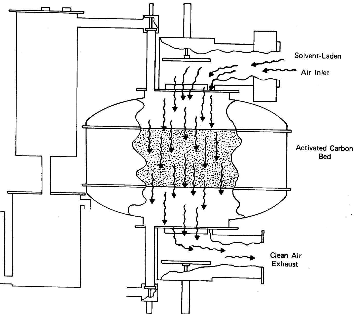
Figure 3-3 ADSORPTION CYCLE
