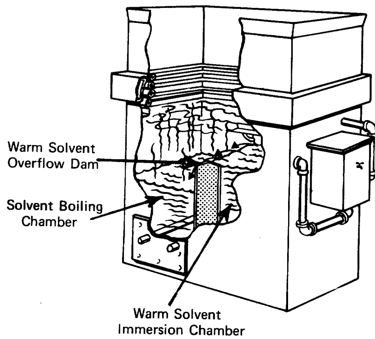
Figure 2-7 TWO COMPARTMENT DEGREASER
