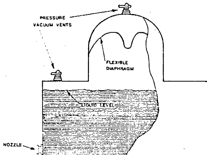
FIGURE 4.3-7. FLEXIBLE DIAPHRAGM TANK (INTEGRAL UNIT)
