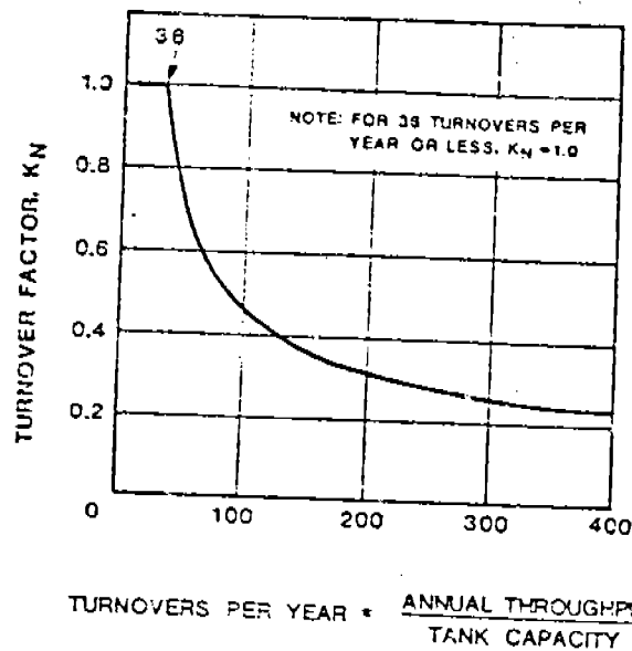
FIGURE 4.3-11. TURNOVER FACTOR ( K_N ) FOR FIXED ROOF TANKS
