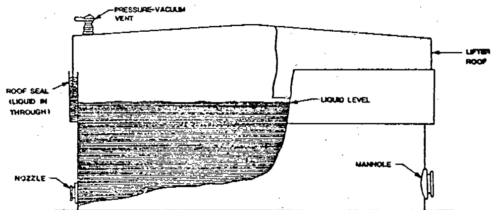
FIGURE 4.3-6. LIFTER ROOF STORAGE TANK (WET SEAL)
