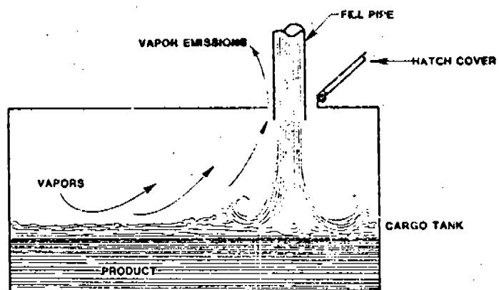
FIGURE 4.4-2 SPLASH LOADING METHOD
