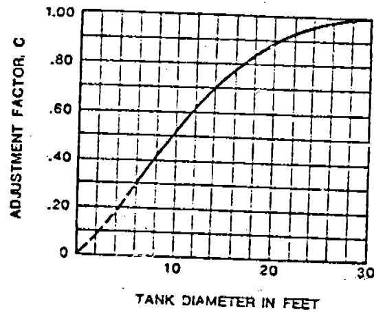
FIGURE 4.3-10. ADJUSTMENT FACTOR (C) FOR SMALL DIAMETER TANKS
