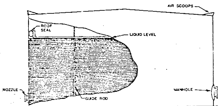
FIGURE 4.3-5. COVERED FLOATING ROOF STORAGE TANK
