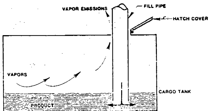
FIGURE 4.4-2 SPLASH LOADING METHOD
