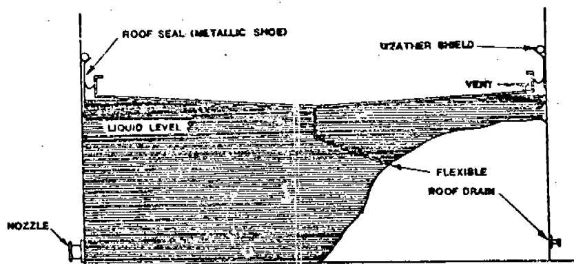
FIGURE 4.3-3. PAN-TYPE FLOATING ROOF STORAGE TANK (METALLIC SEALS)
