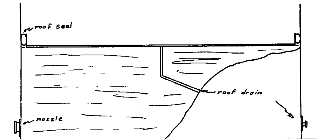
FIGURE 2.2-2 - PAN-TYPE FLOATING ROOF TANK
