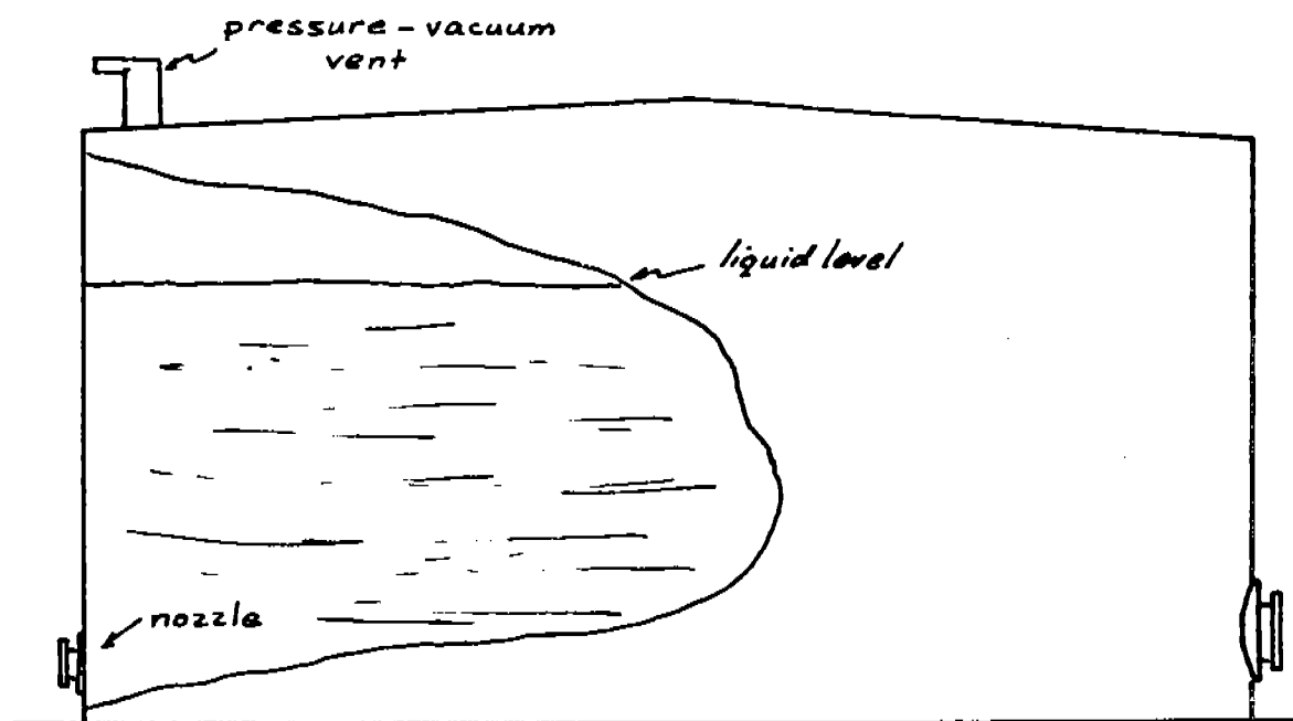
FIGURE 2.2-1 - STANDARD FIXED CONE ROOF TANKS
