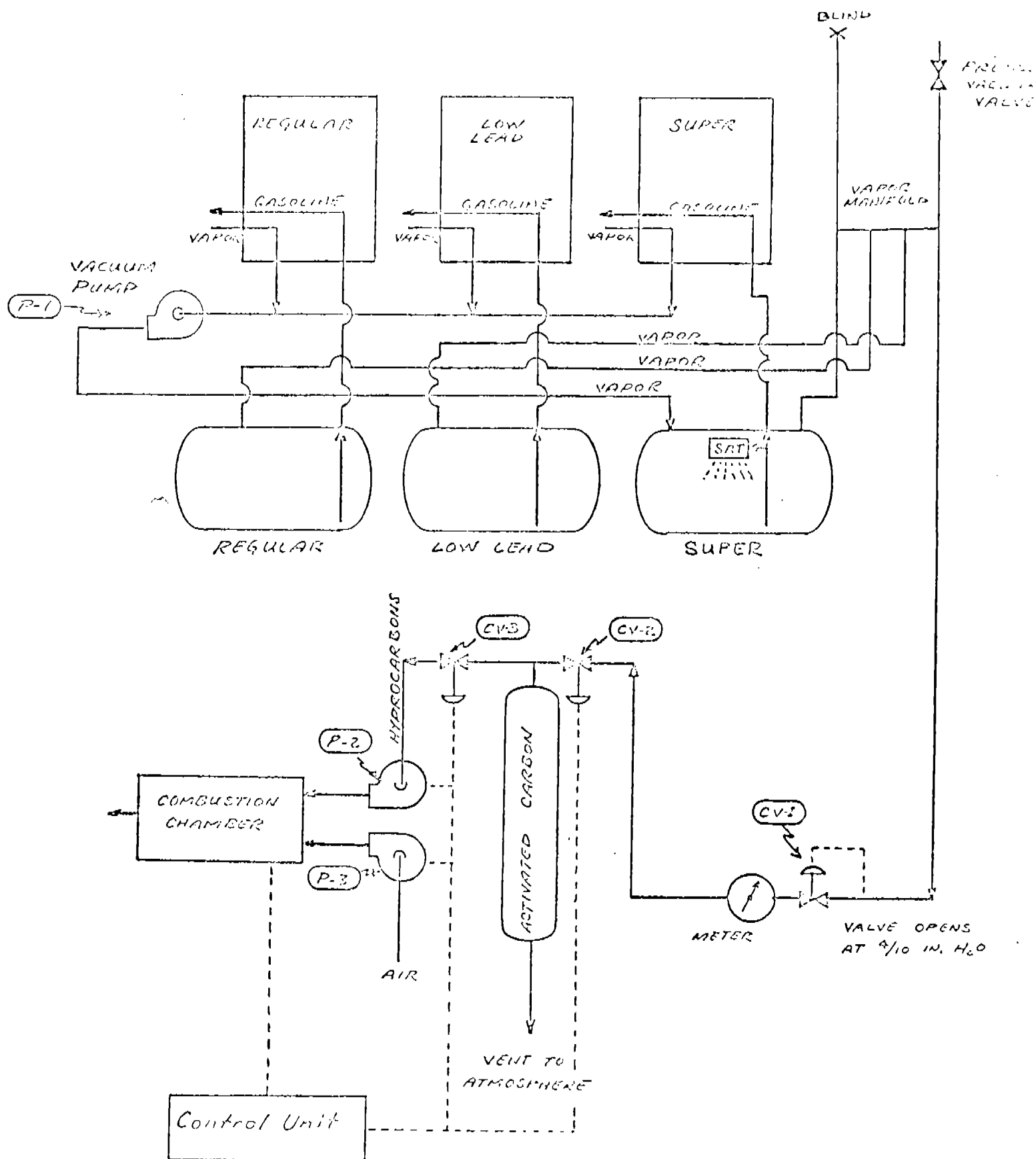
FIGURE 2.2-28. SCHEMATIC DIAGRAM OF A THERMAL OXIDATION UNIT
