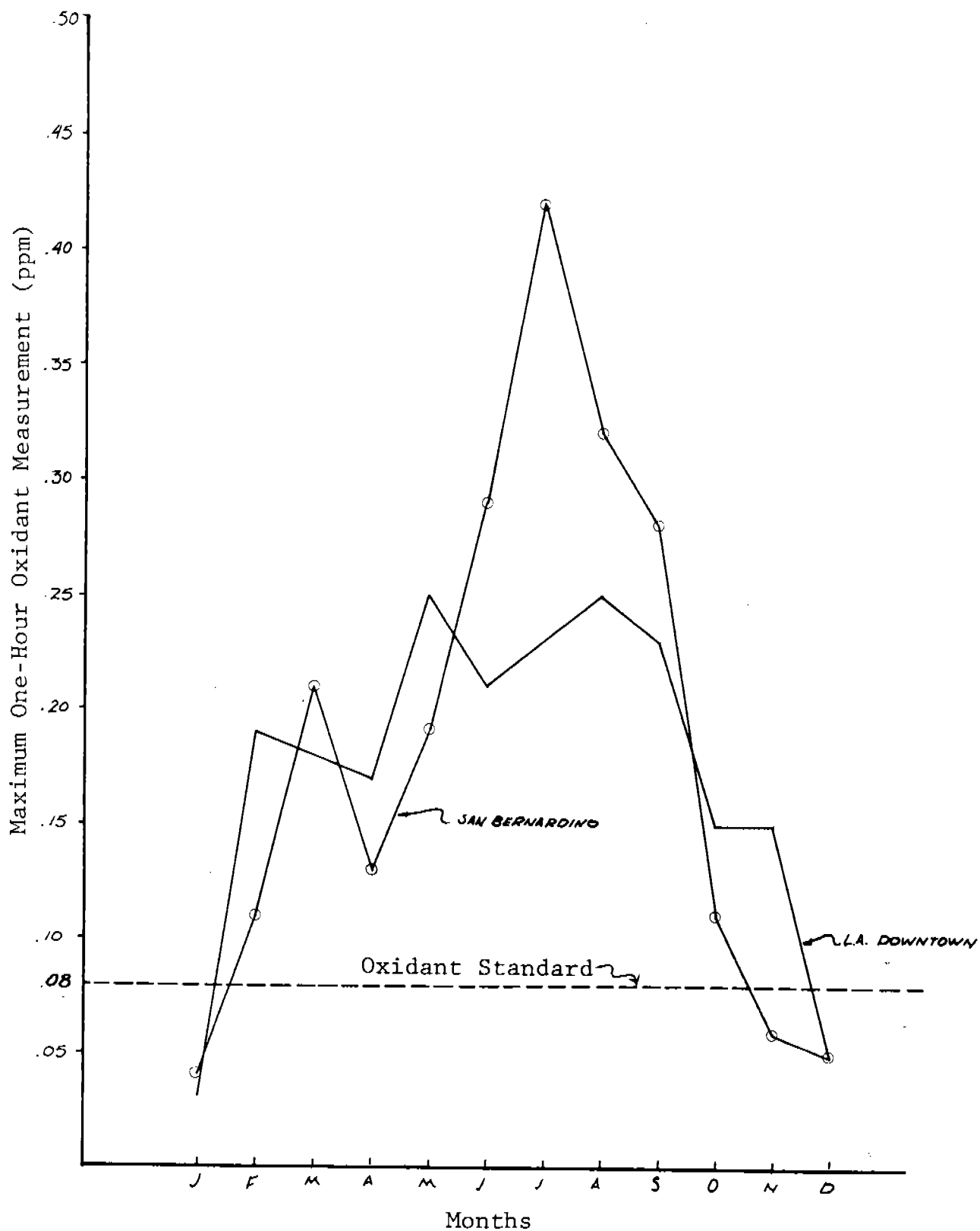
FIGURE 2.1-4 - MONTHLY OXIDANT MAXIMA, LOSS ANGELES AND SAN BERNADINO, CALIFORNIA - 1972
