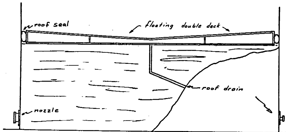
FIGURE 2.2-4 - DOUBLE DECK FLOATING ROOF
