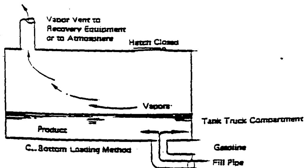
Figure 4-1. Gasoline Tank Truck Loading Methods
