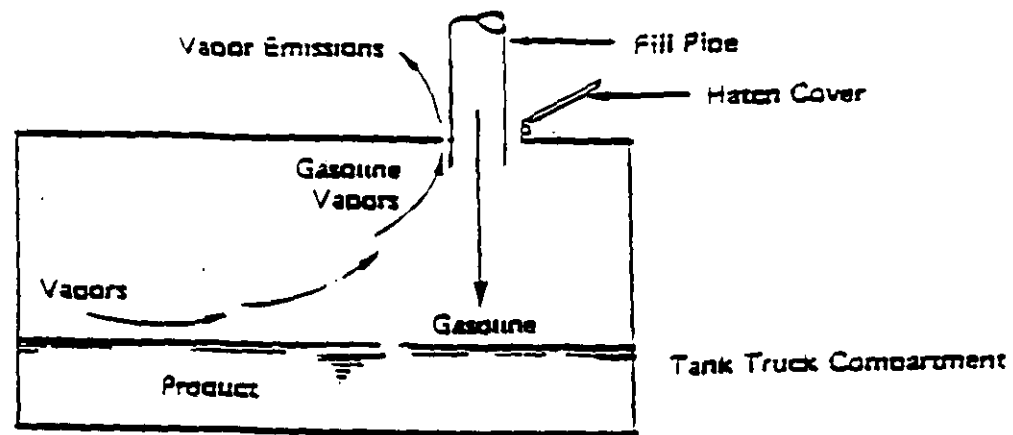
A. Top Splash Loading Method
