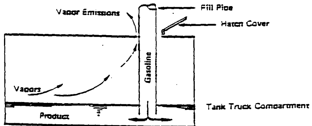
B. Top Submerged Method
