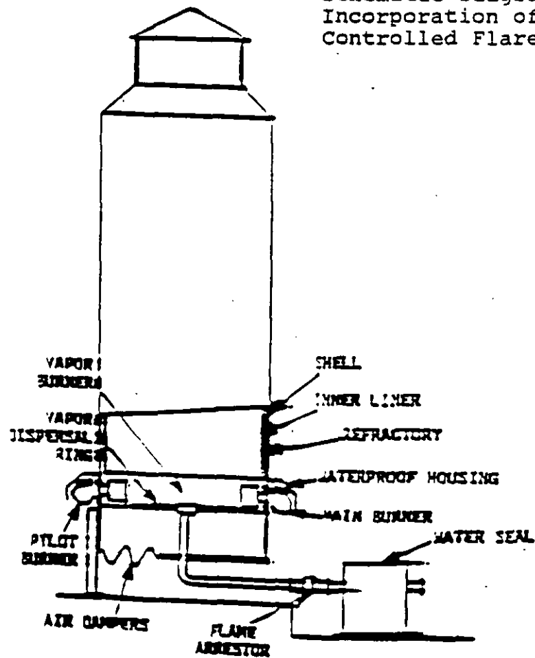
Figure 4-6. A Typical Temperature Controlled Flare and Simplified Flow Diagram (Diagram Courtesy of the John Zink Company)
