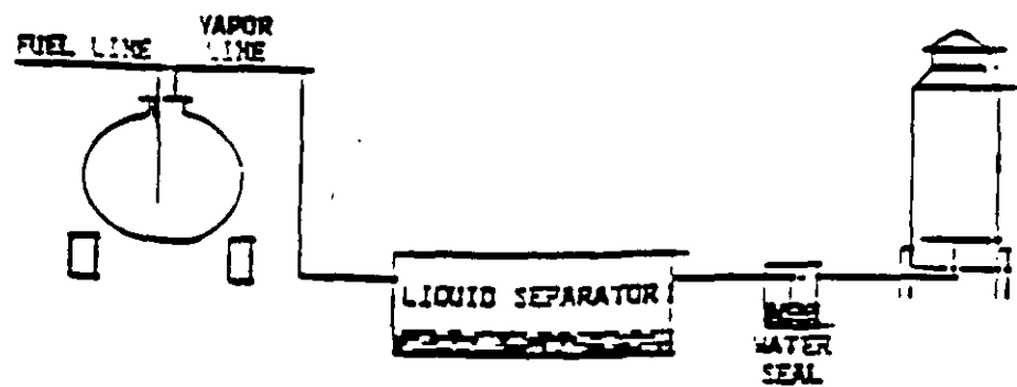
Schematic Diagram Showing Incorporation of Temperature Controlled Flare
