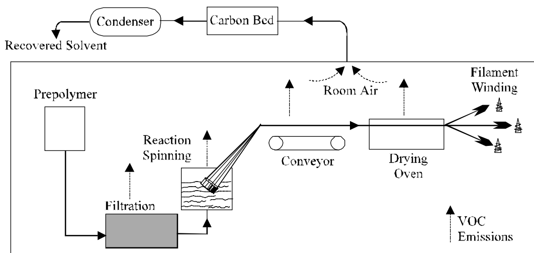
Figure 6.9-13. Spandex reaction spinning.
