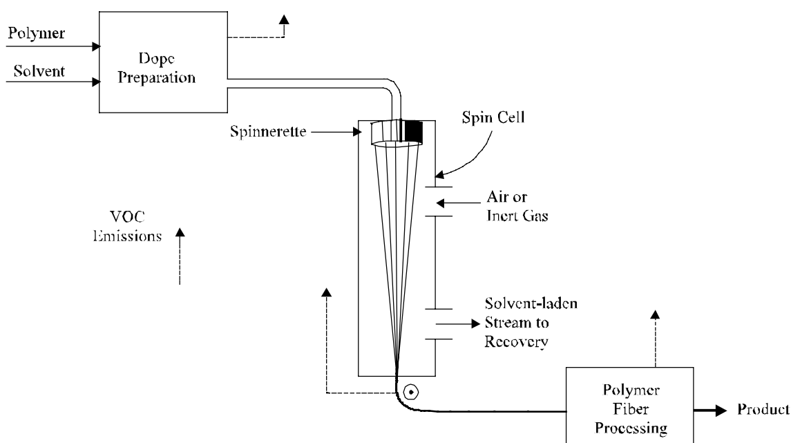
Figure 6.9-3. Dry spinning.
