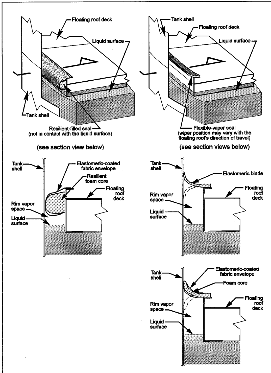
Figure 2-8. Vapor mounted primary seals. 11
