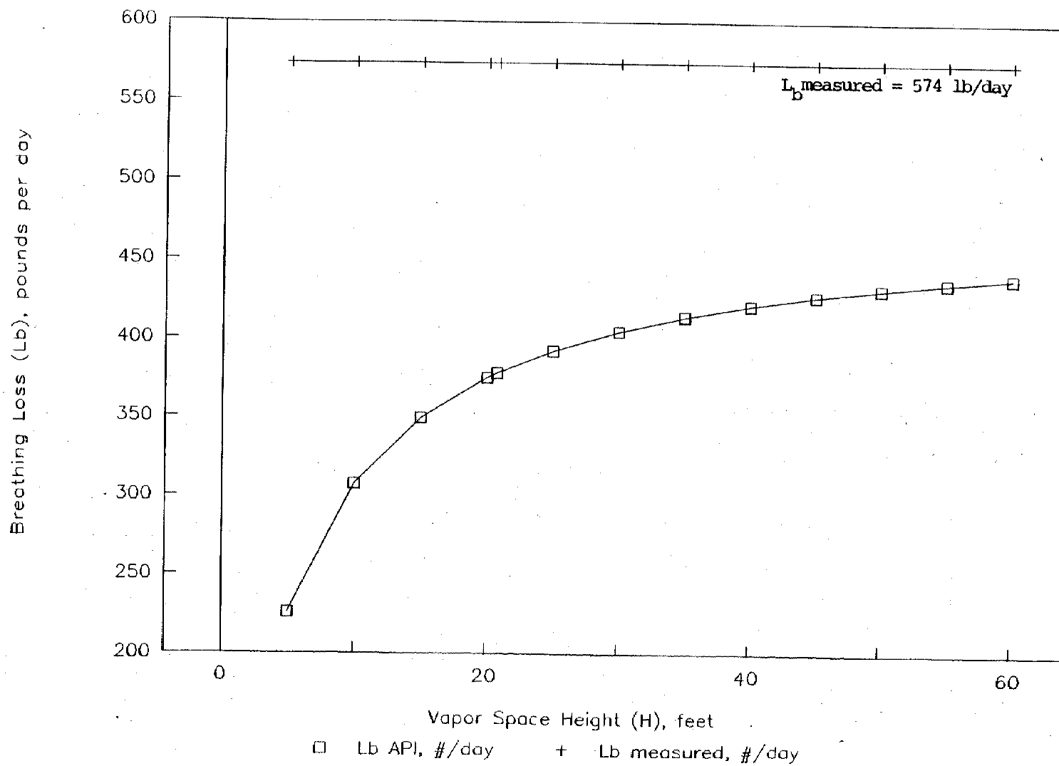
Figure 4-6. Sensitivity of Equation 4-2 to changes in the vapor space outage ( H_{VO} ).
