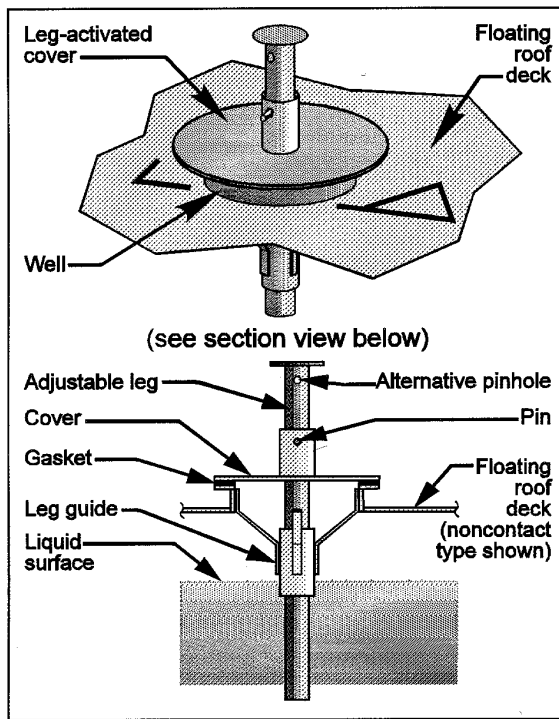
Vacuum Breaker
