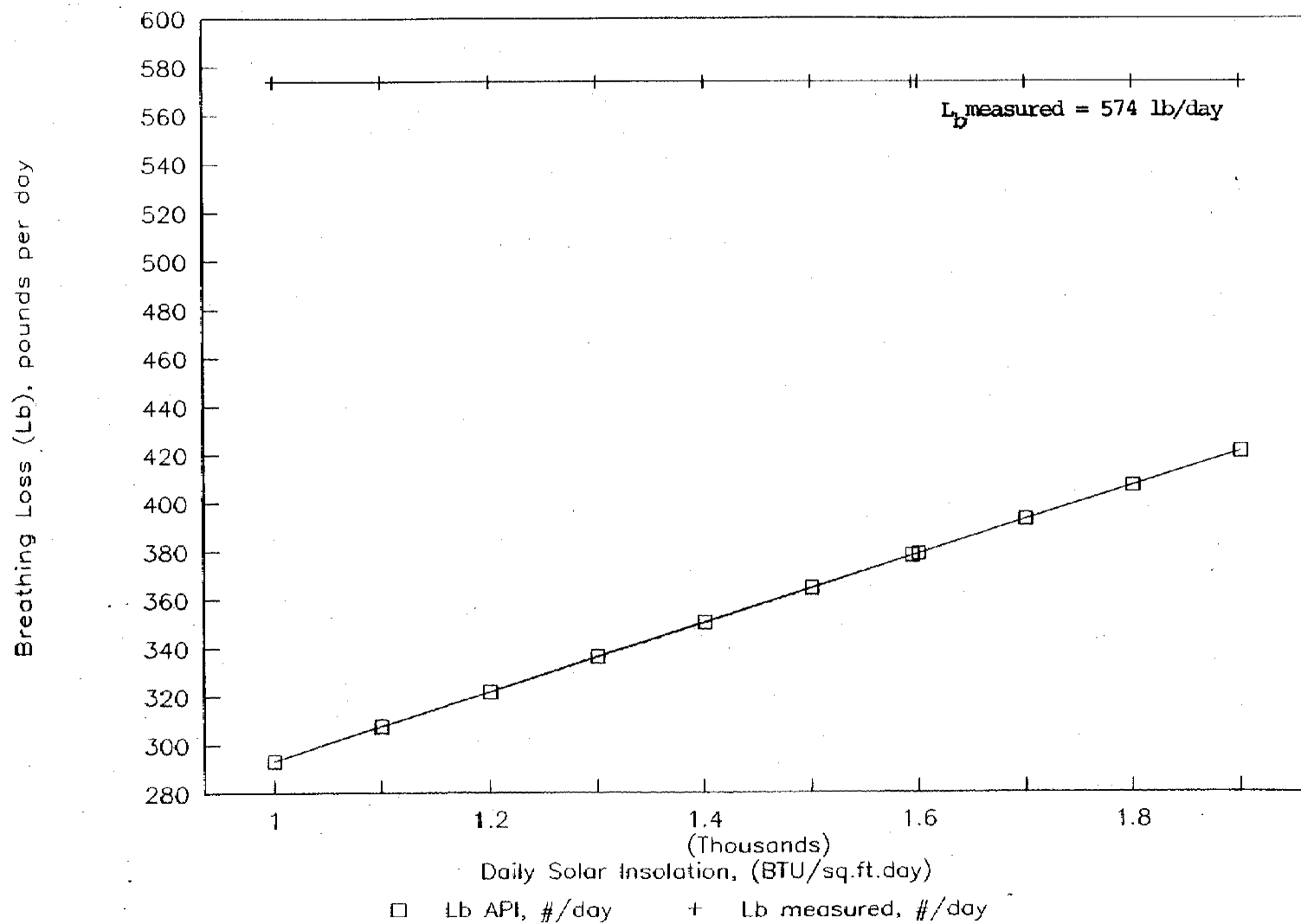
Figure 4-10. Sensitivity of Equation 4-2 to changes in the solar absorptance ( \alpha ).
