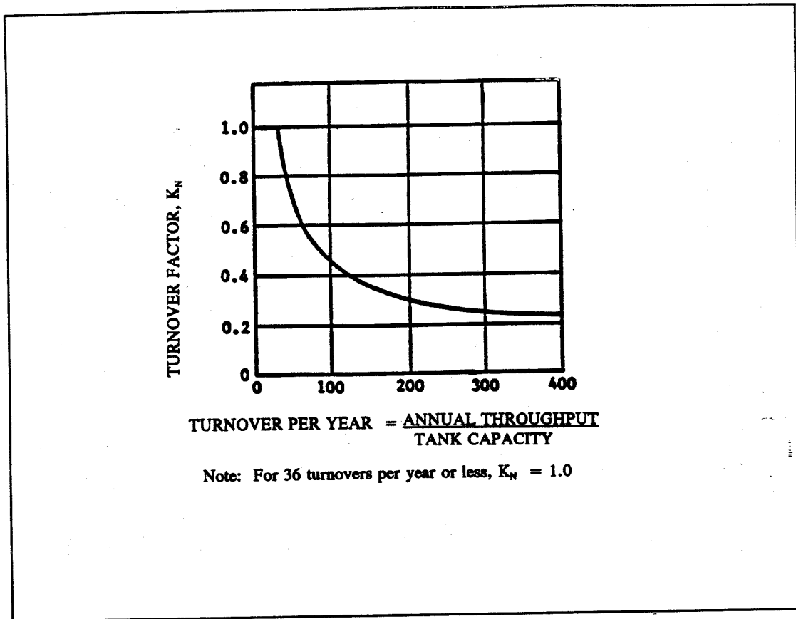
Figure 3-10. Turnover factor ( K_N ) for fixed roof tanks. 1
