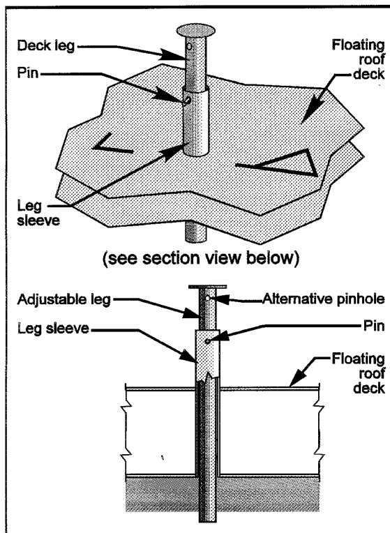
Deck Leg
