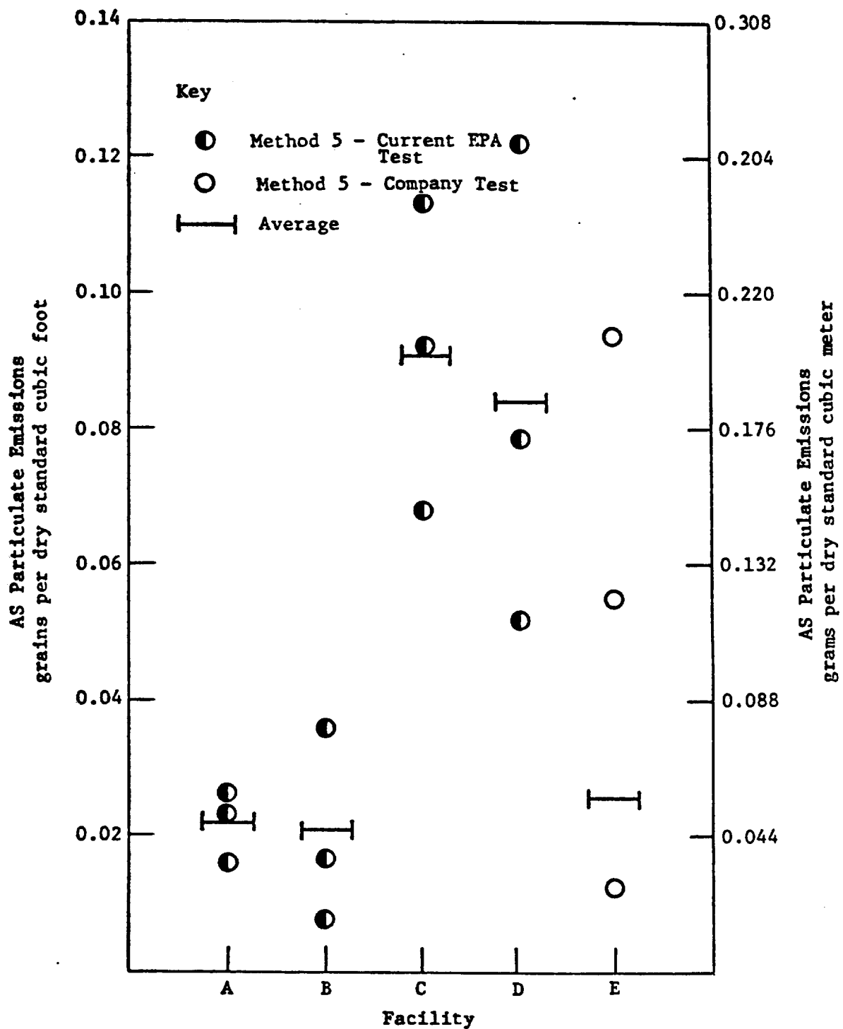
FIGURE C-1 CONTROLLED AS PARTICULATE EMISSIONS FROM EPA EMISSION TESTS—CALCULATED GRAIN LOADINGS
