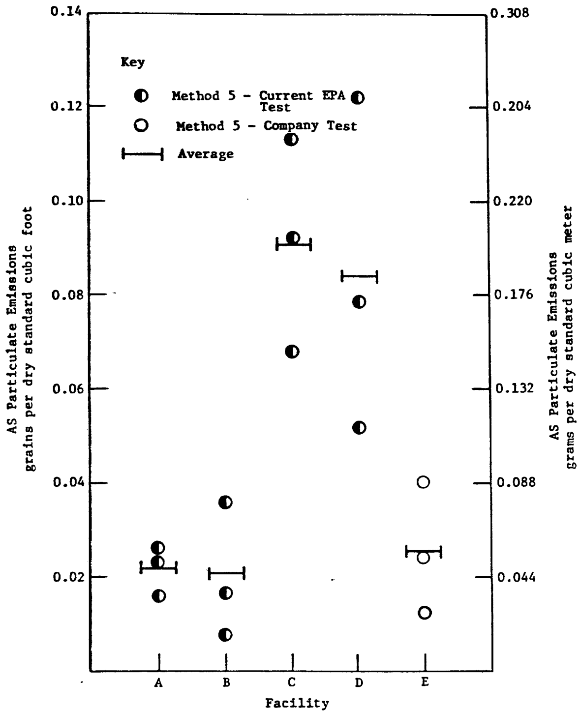
FIGURE 4-4 CONTROLLED AS PARTICULATE EMISSIONS FROM EPA EMISSION TESTS—CALCULATED GRAIN LOADINGS
