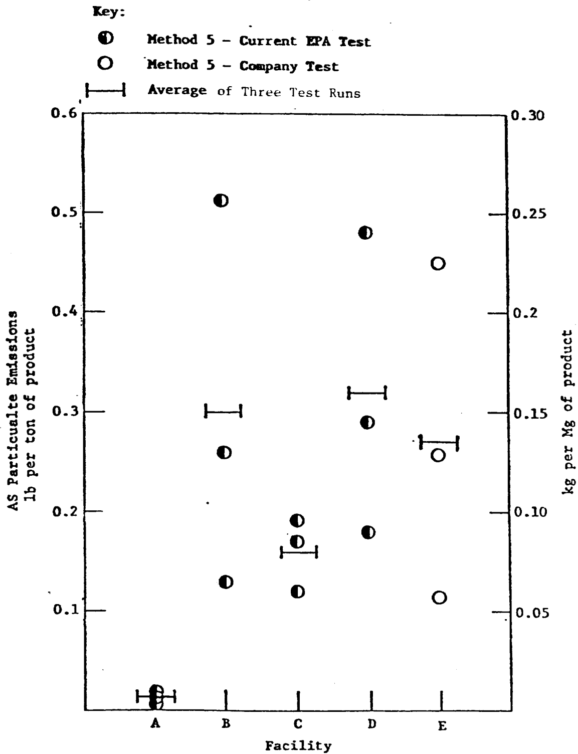
FIGURE 1 CONTROLLED AS PARTICULATE EMISSIONS FROM EPA EMISSION TESTS—CALCULATED MASS EMISSION RATES
