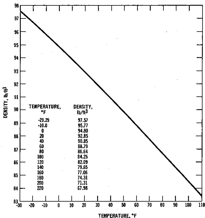
Figure C-1. Density of liquid chlorine. 33
