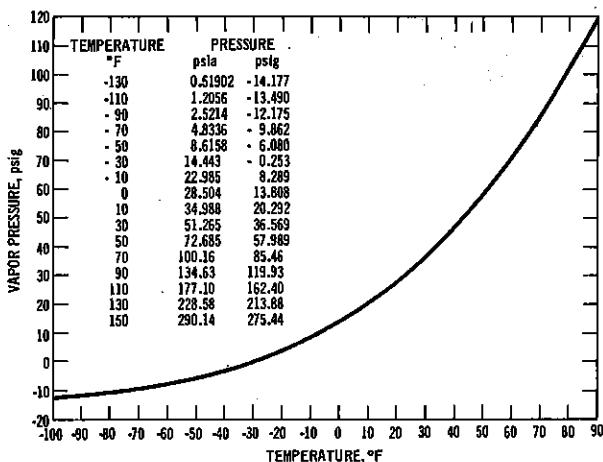
Figure C-4. Vapor pressure of liquid chlorine. 35
