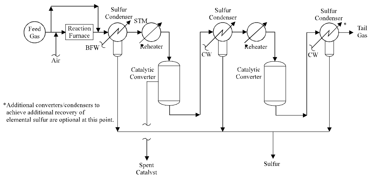
Figure 8.13-1. Typical Claus sulfur recovery unit. CW = Cooling water. STM = Steam. BFW = Boiler feed water.
