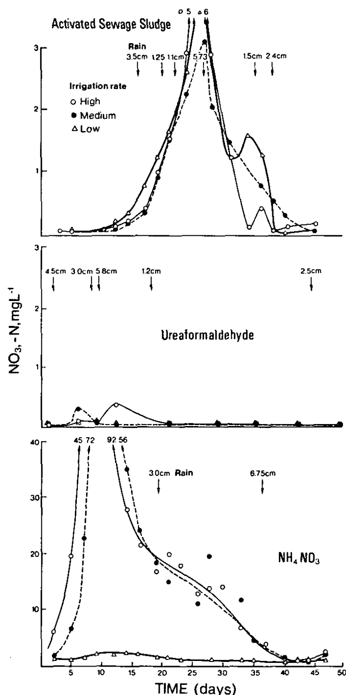
Fig. 5. Leachate concentration of NO 3 -N as a function of N source and irrigation (low, medium, high): Milorganite applied on 17 Oct. 1973 at a rate of 146 kg N ha -1 , ureaformaldehyde applied on 6 June 1973 at a rate of 244 kg N ha -1 ; NH 4 NO 3 applied on 16 Feb. 1973 at a rate of 163 kg N ha -1 (with permission from Brown et al., 1977).
