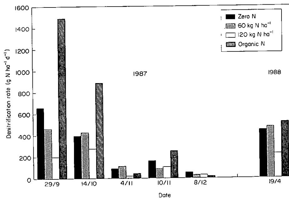
Fig. 7. Denitrification flux measured by core incubation, Glencorse Mains, 1987-88.
