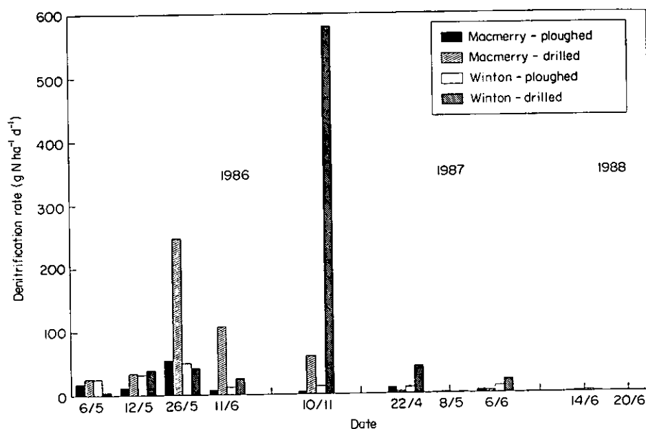
Fig. 6. Denitrification flux measured by core incubation, South Road, 1986-88.
