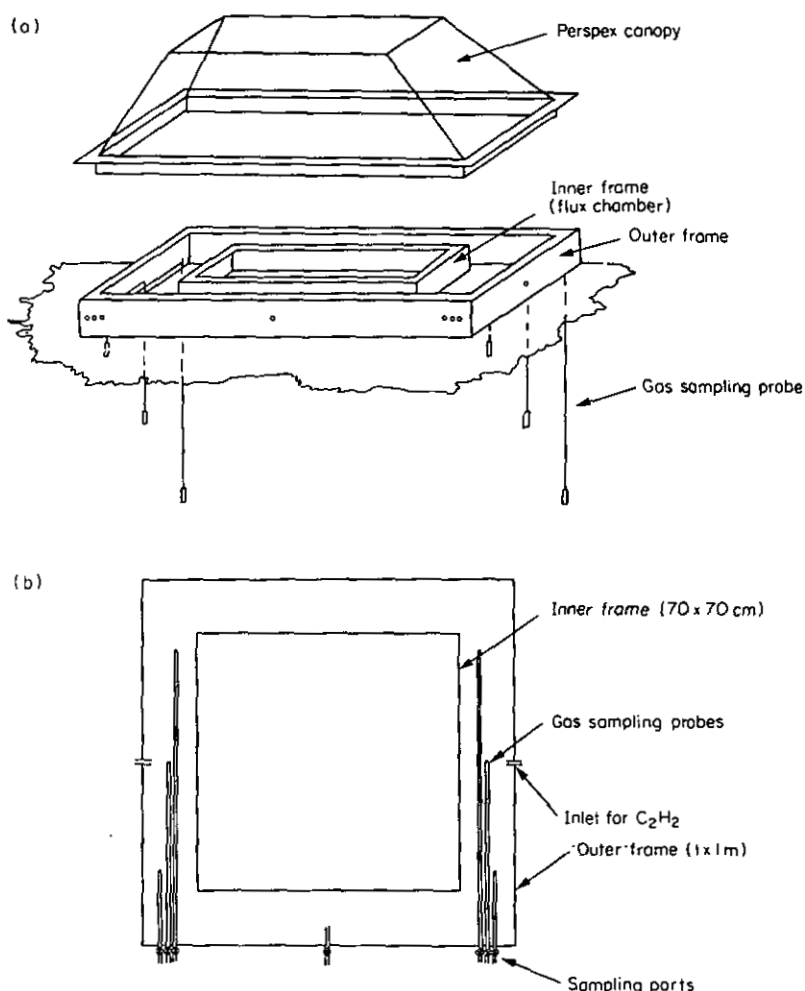
Fig. 1. Apparatus for field application of acetylene and measurement of gaseous emissions from soil: (a) 'exploded' view showing perspex canopy for covering soil and crop during application of acetylene; (b) plan view showing location of gas sampling probes in guard area between frames.
