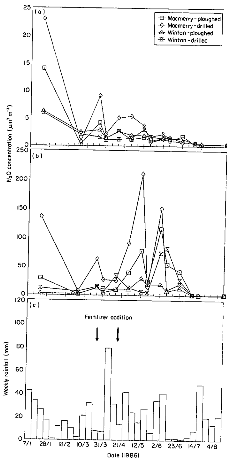
Fig. 2. N 2 O concentrations recorded in soil atmosphere, South Road, 1986: (a) 5 cm depth; (b) 20 cm depth; (c) weekly precipitation.
