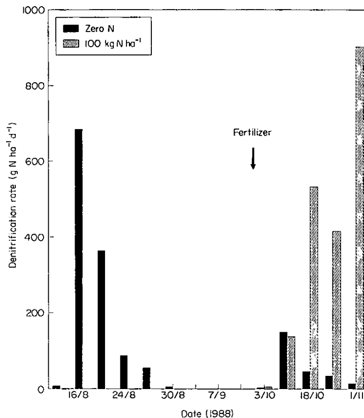
Fig. 5. Surface denitrification flux, measured using acetylene inhibition, Croft Field, 1988.
