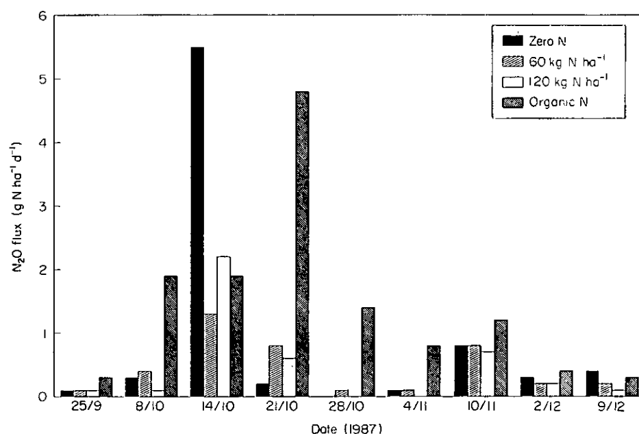
Fig. 3. Surface N 2 O flux measured using closed chambers, Glencorse Mains, autumn 1987.
