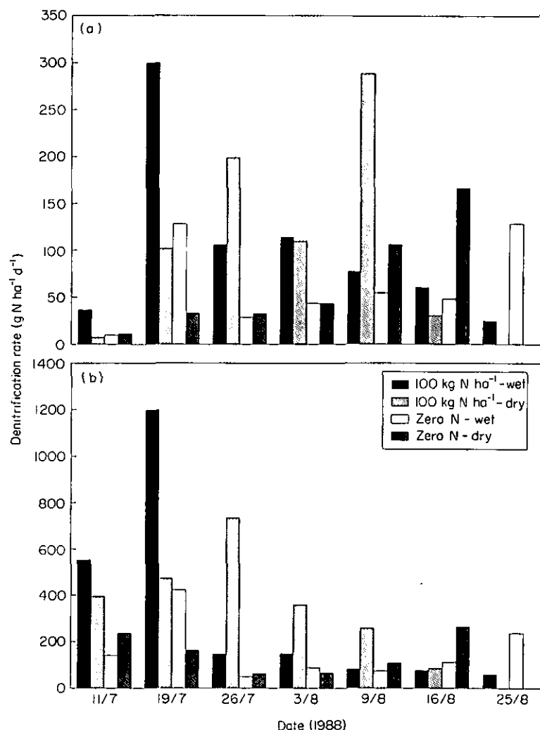
Fig. 8. Denitrification flux measured by core incubation, South Road, Winton soil, summer 1988: (a) cores incubated at atmospheric oxygen concentration; (b) cores incubated at decreased oxygen concentrations (3–12% by volume).
