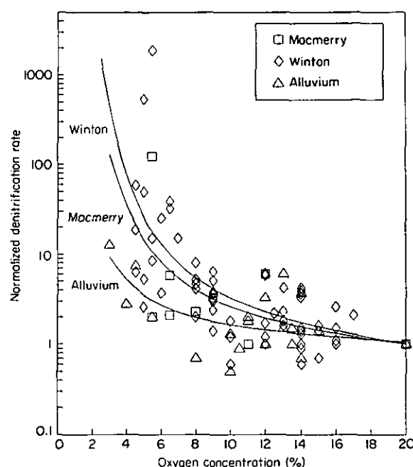
Fig. 9. Relationship between oxygen concentration in incubation vessel and measured denitrification rate, South Road and Croft Field, 1988.
