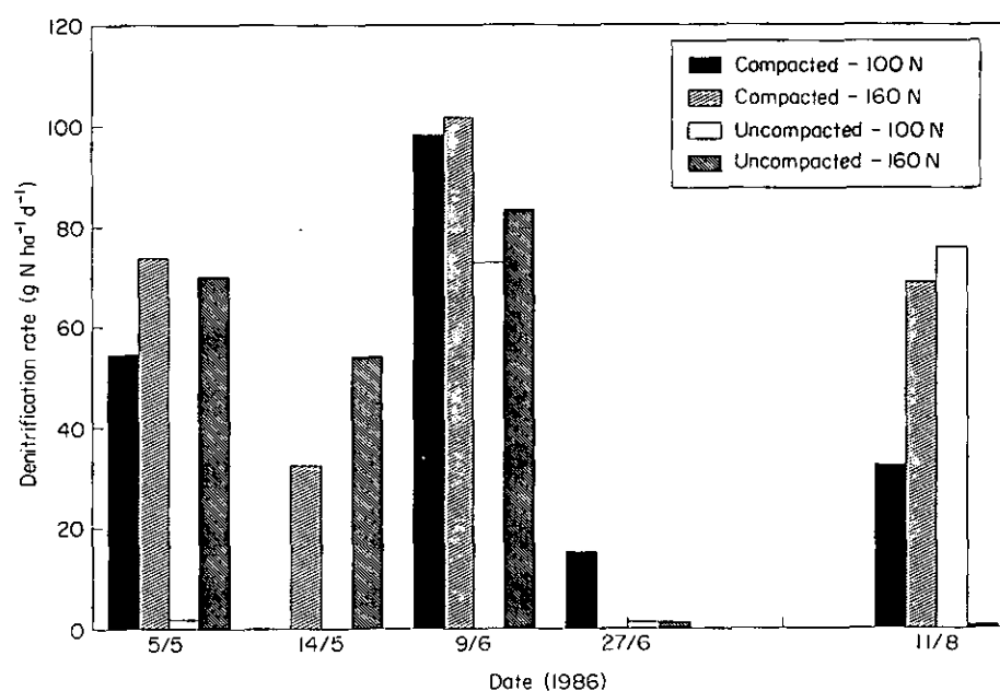
Fig. 4. Surface denitrification flux measured using acetylene inhibition, Bush House, 1986.
