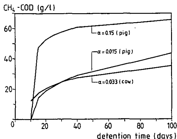
Fig. 1. Predicted methane production as a function of the detention time at digestion of 'fresh' cow manure ( S_{p0} = 44 \text{ g COD l}^{-1} , S_{m0} = 5 \text{ g COD l}^{-1} , \text{NH}_4^+ \text{-N} = 3.5 \text{ g l}^{-1} ) and fresh pig manure ( S_{p0} = 65 \text{ g COD l}^{-1} , S_{m0} = 5 \text{ g COD l}^{-1} , \text{NH}_4^+ \text{-N} = 5 \text{ g l}^{-1} ) in CSTR-systems. The total influent COD for both pig and cow manure is 100 \text{ g l}^{-1} .
