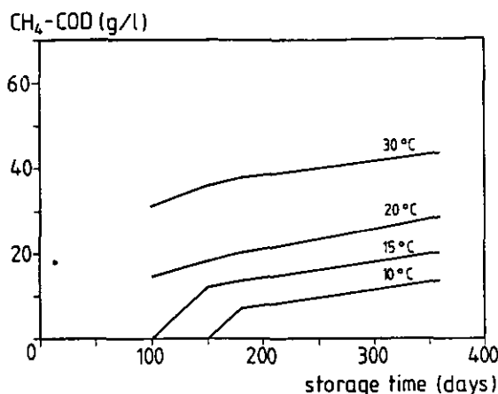
Fig. 3. Predicted total methane production as a function of the storage time at temperatures of 10, 15, 20 en 30^\circ\text{C} , for the digestion of 'fresh' cow manure ( S_{p0} = 44 \text{ g COD l}^{-1} , S_{m0} = 5 \text{ g COD l}^{-1} , \text{NH}_4^+ \text{-N} = 3.5 \text{ g l}^{-1} ) in a fed-batch-system at 15% inoculation.
