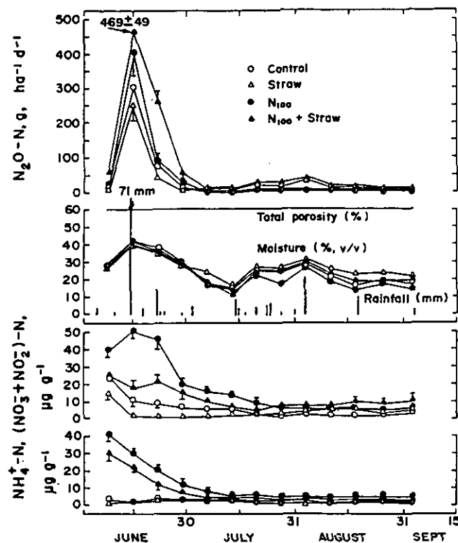
Fig. 1—Gaseous N losses (N 2 O-N), soil moisture, rainfall, (NO 3 - + NO 2 - ) - N and NH 4 + - N of conventional-tilled Elstow clay loam seeded to wheat with various straw and N treatments. Φ indicates standard deviation within three replicates.
