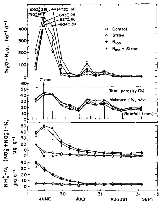
Fig. 2—Gaseous N losses ( \text{N}_2\text{O}-\text{N} ), soil moisture, rainfall, ( \text{NO}_3^- + \text{NO}_2^- - \text{N} and \text{NH}_4^+-\text{N} ) of zero-tilled Elstow clay loam seeded to wheat with various straw and N treatments. \Phi indicates standard deviation within three replicates.
