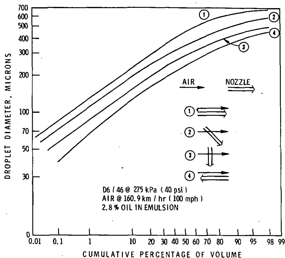
Figure 2. Drop spectra for four nozzle orientations 13
