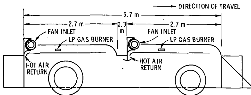
Figure 7. Schematic of 1970 thermal defoliator 60
