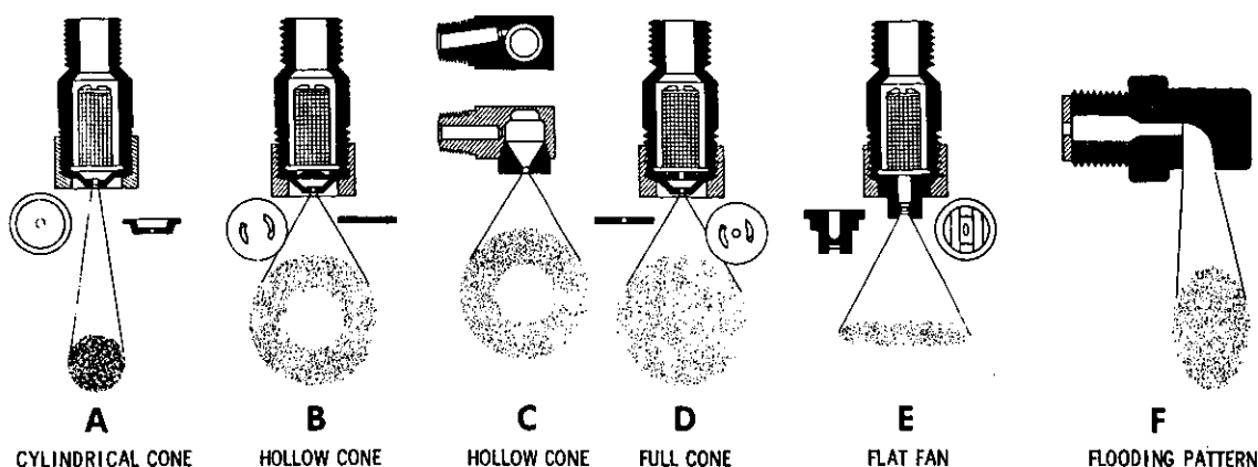
Figure 1. Hydraulic pressure nozzles 6
