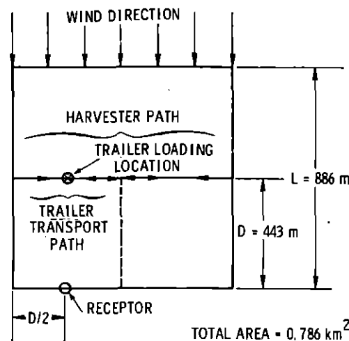
Figure 7. Representative field for calculating cotton harvesting severities
