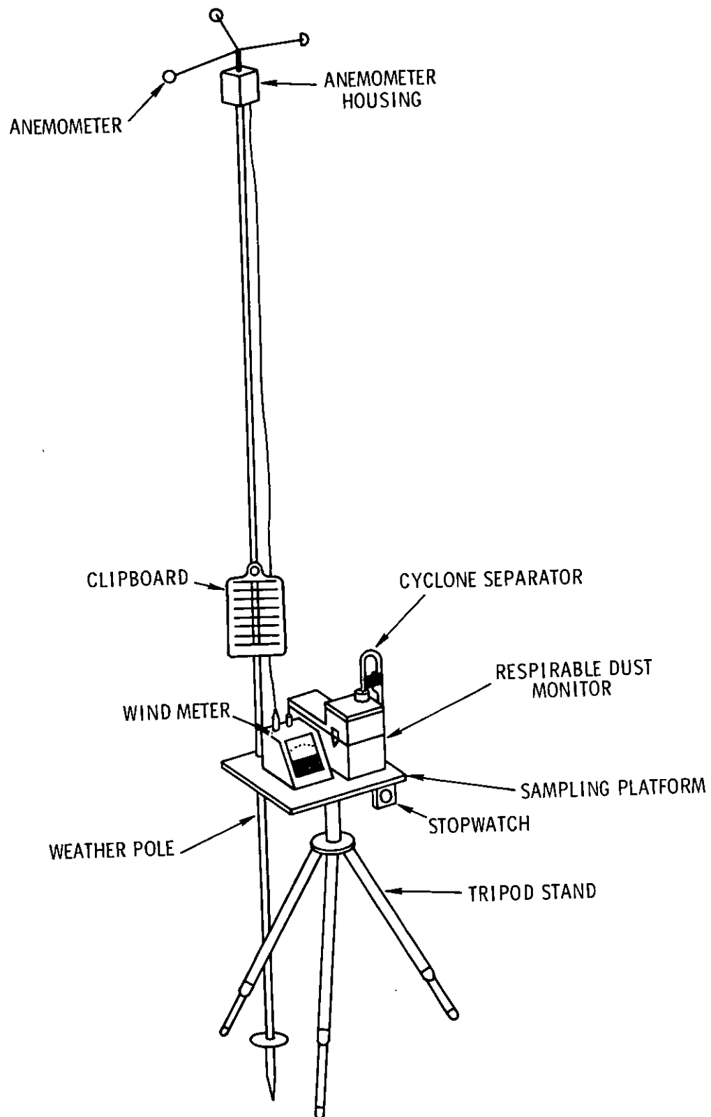
Figure C-2. Sampling apparatus
