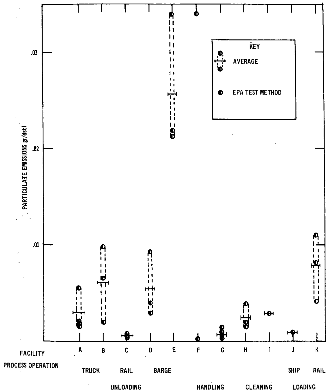
Figure 5-1. Particulate emissions from processes controlled by fabric filters.
