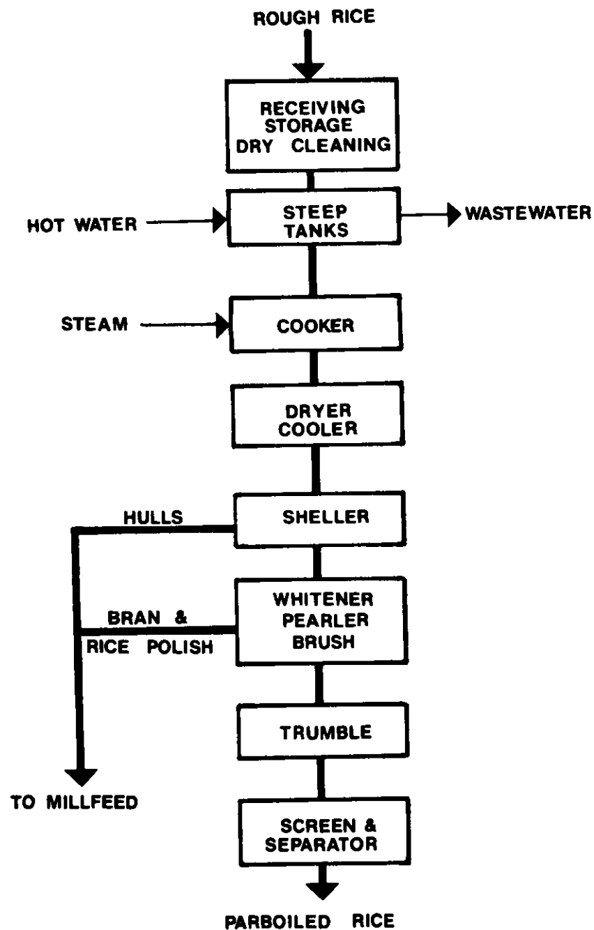
FIGURE 6 THE PARBOILED RICE PROCESS
