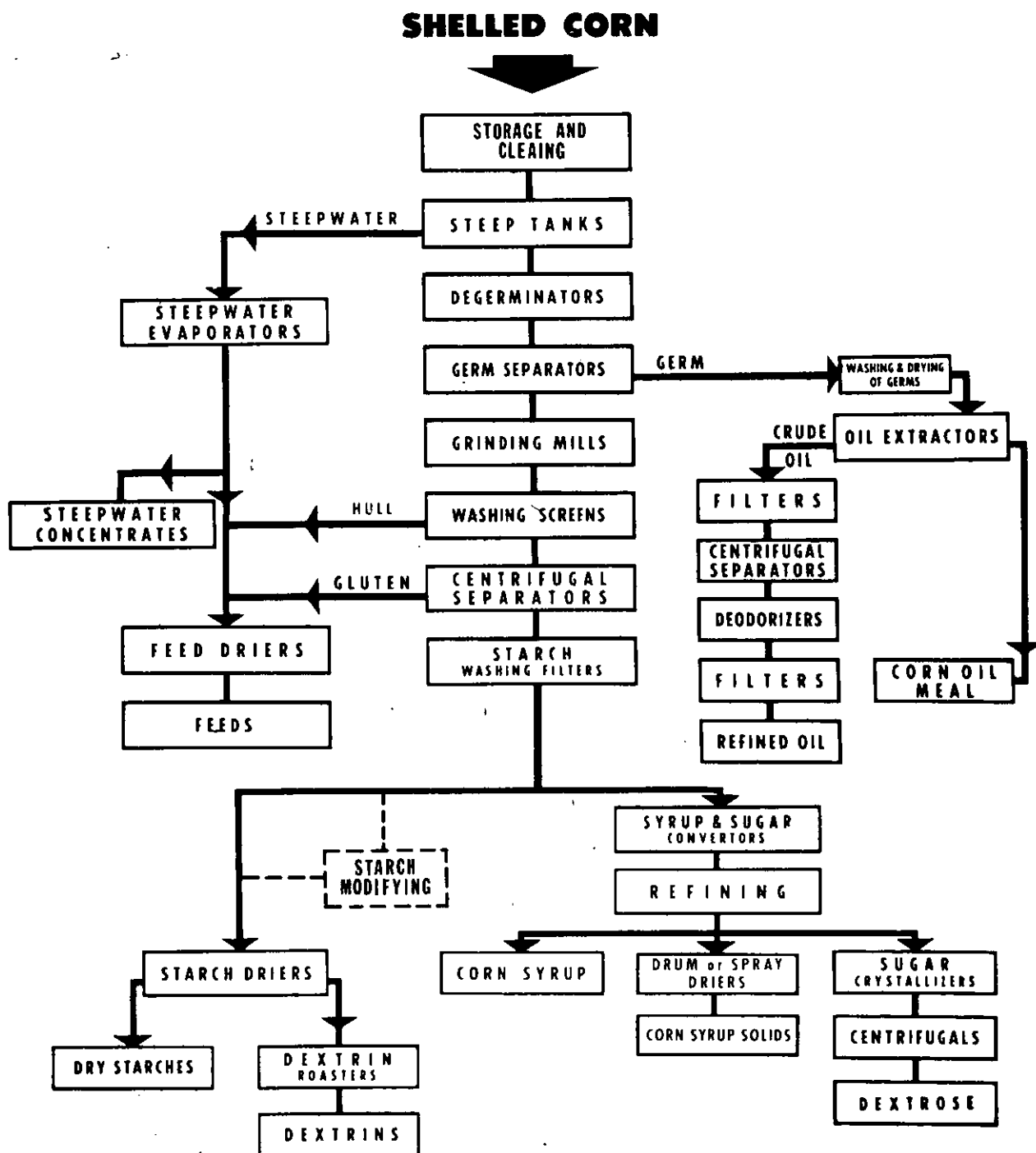
FIGURE 1 THE CORN WET MILLING PROCESS
