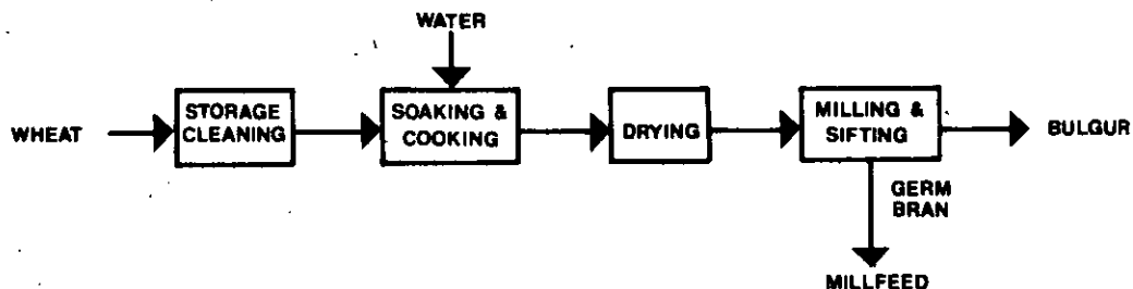
BULGUR PRODUCTION
