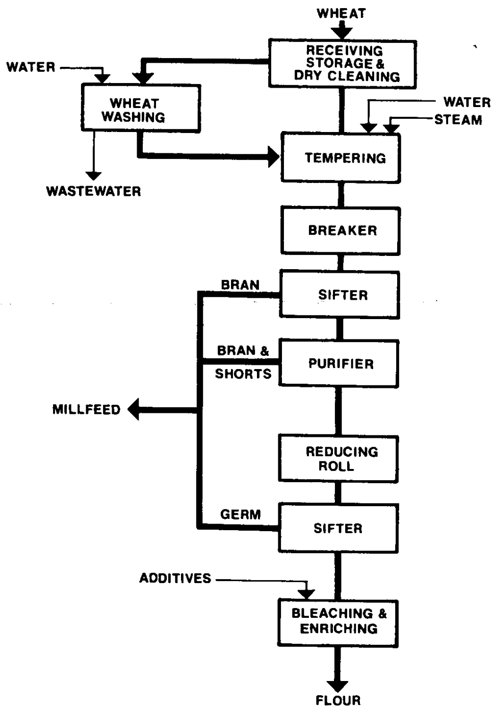
FIGURE 3 THE WHEAT MILLING PROCESS
