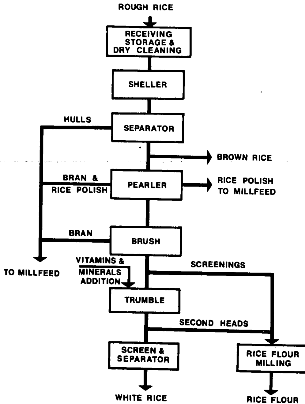
FIGURE 5 THE RICE MILLING PROCESS
