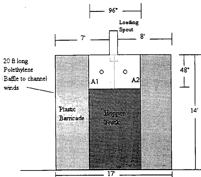
Figure 9. Sampler Deployment for Test Series BE-201 to 202
