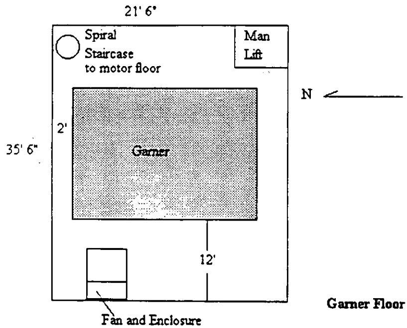
Figure 10. Floor Plans for BF-1 Test Series
