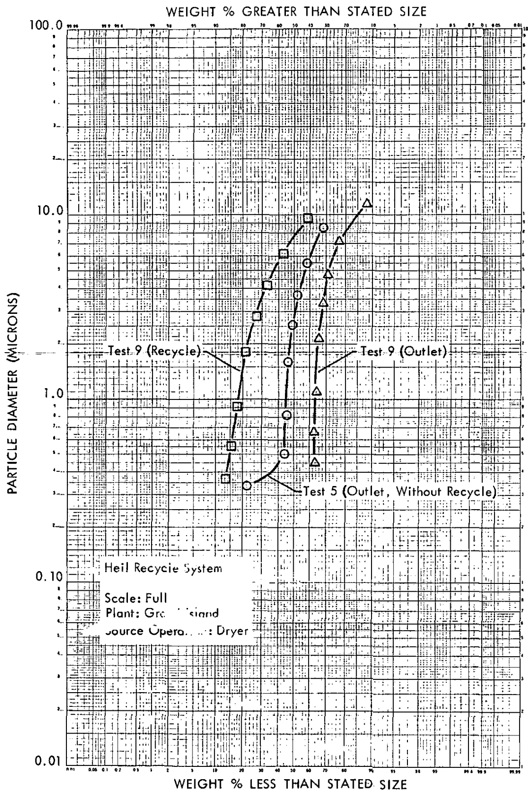
Figure 23 - Particle Size Distributions - Heil Recycle System
