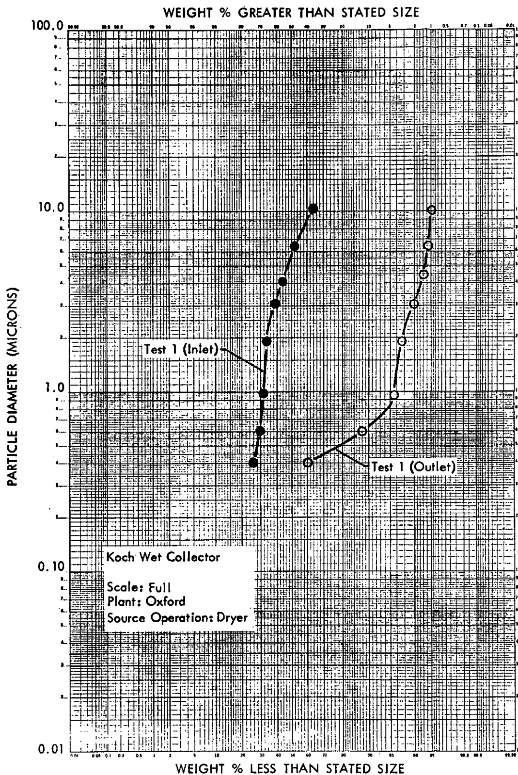
Figure 18 - Particle Size Distributions - Koch Wet Collector (Oxford)
