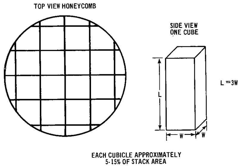
Figure 13. Straightening vanes.
