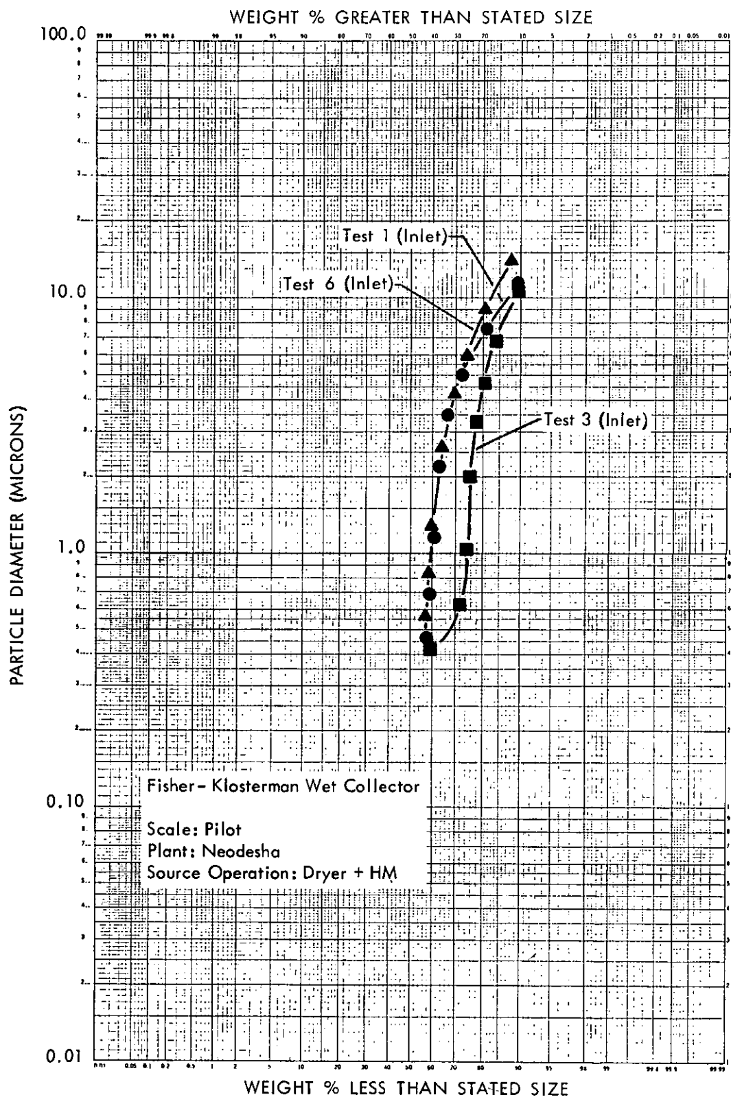
Figure 16- Particle Size Distributions - F/K Wet Collector
