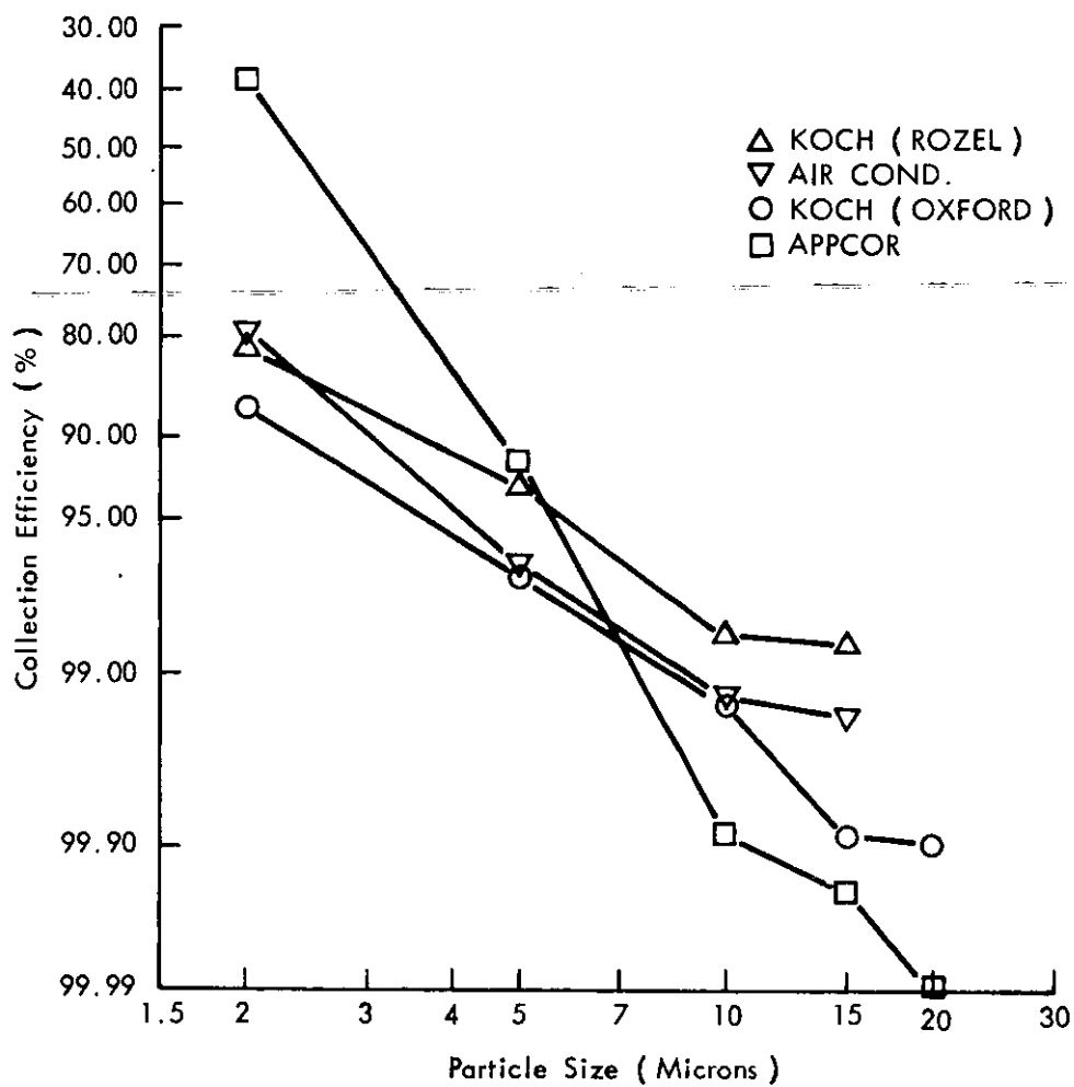
Figure 21 - Fractional Collection Efficiency Curves
