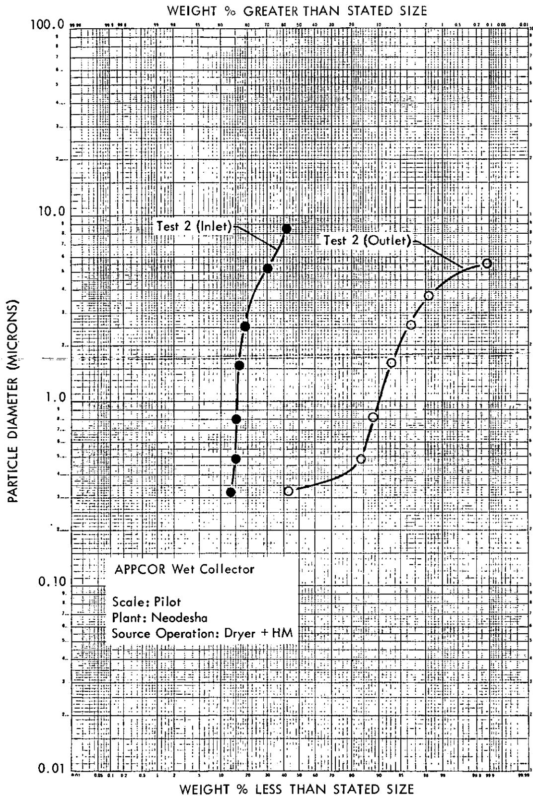
Figure 17 - Particle Size Distributions - APPCOR Wet Collector
