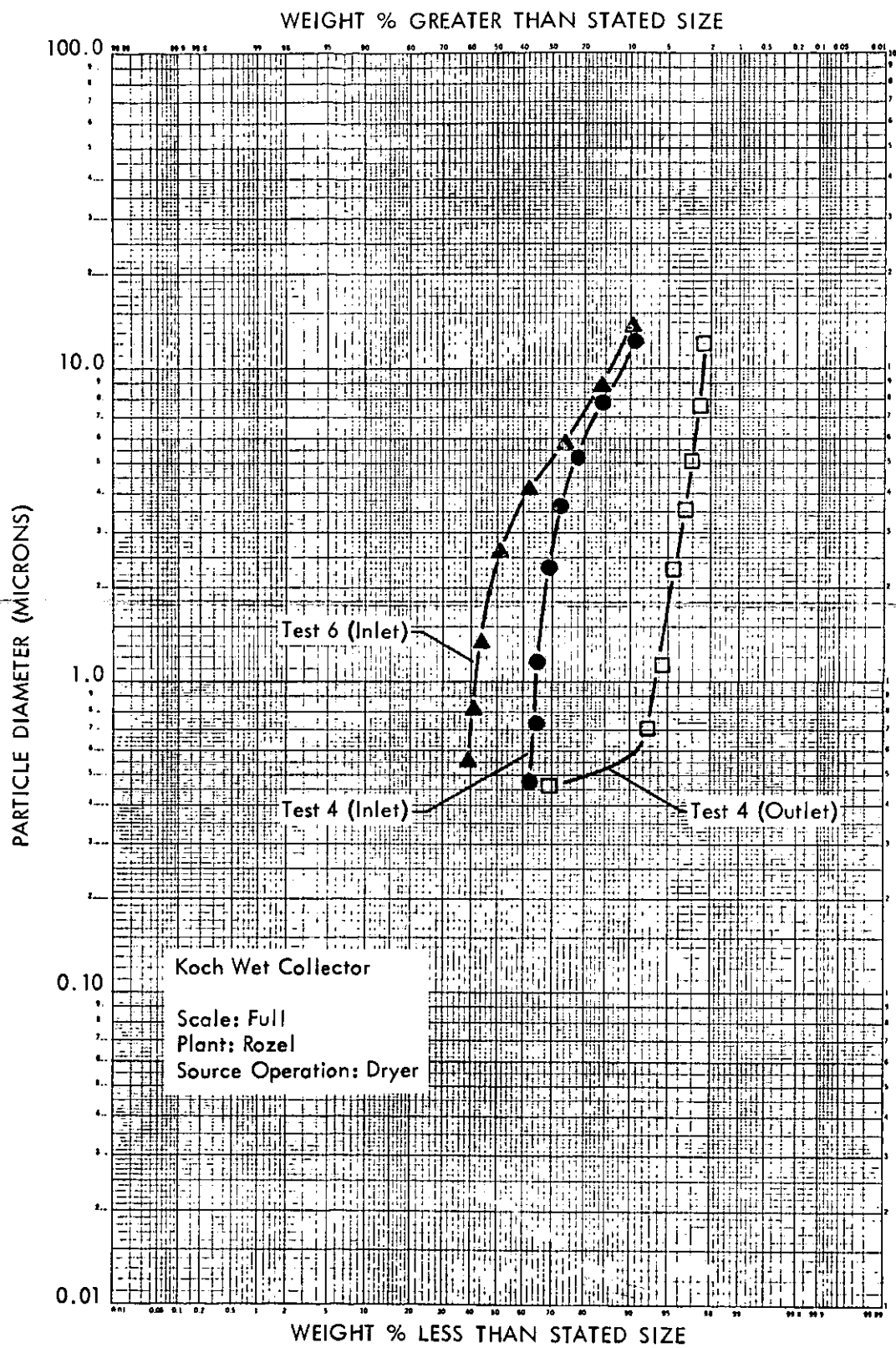
Figure 19 - Particle Size Distributions - Koch Wet Collector (Rozel)
