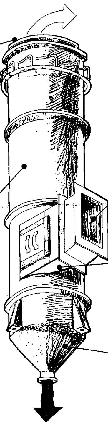
Figure 1 - Fisher-Klosterman Wet Collector (Courtesy of Fisher-Klosterman, Inc.)
