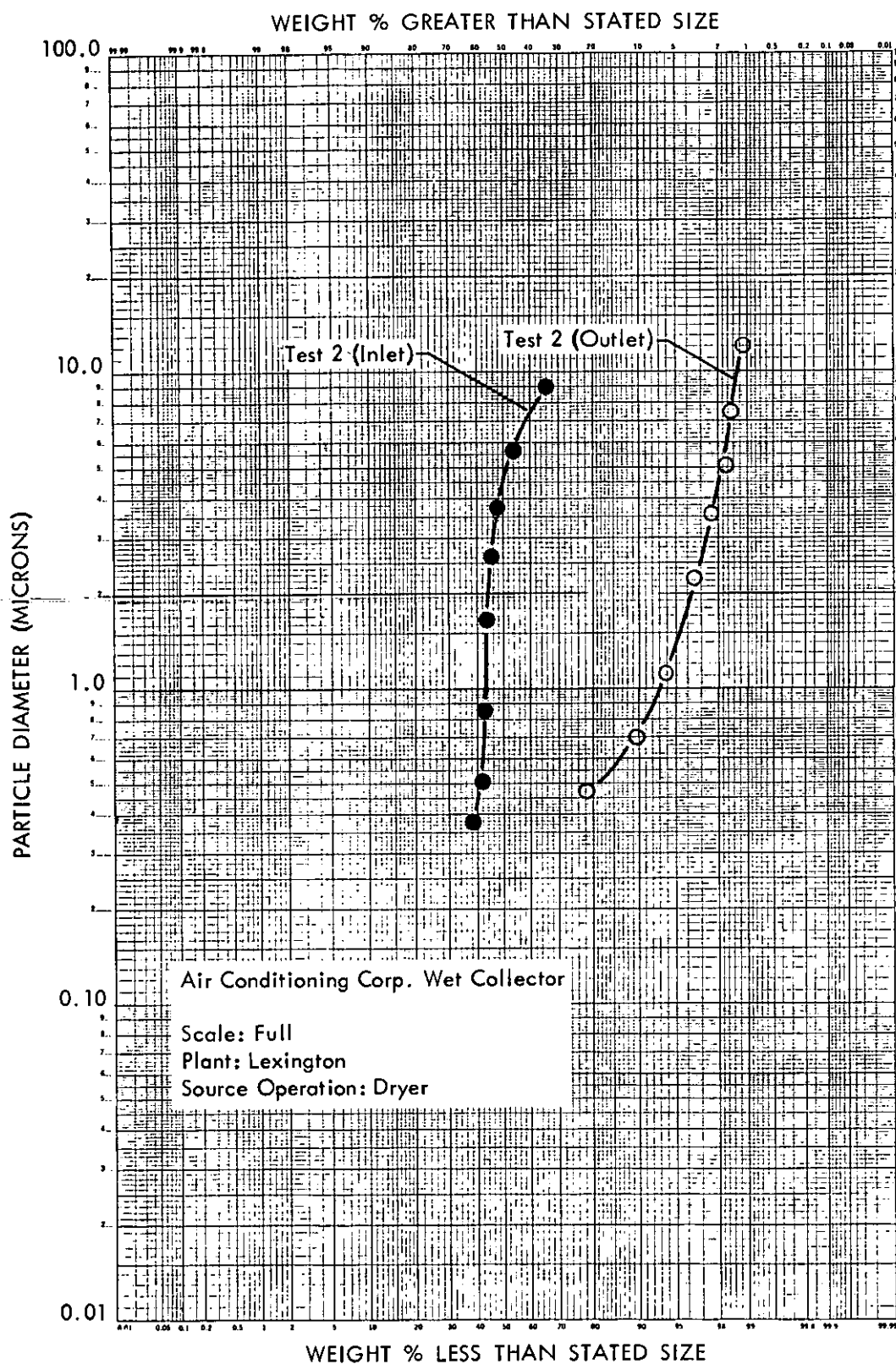
Figure 20 - Particle Size Distributions - ACC Wet Collector
