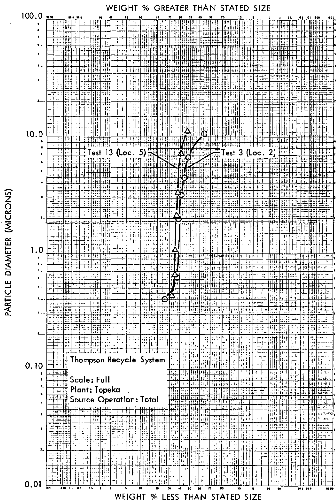
Figure 22 - Particle Size Distributions - Thompson Recycle System
