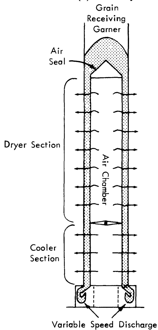
(b) Column Dryer
