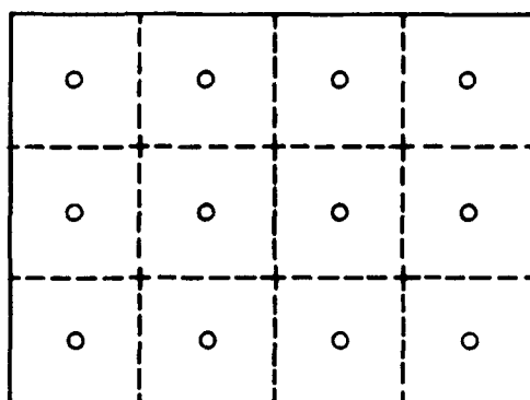
Cross section of rectangular stack divided into 12 equal areas, with traverse points at centroid of each area.
