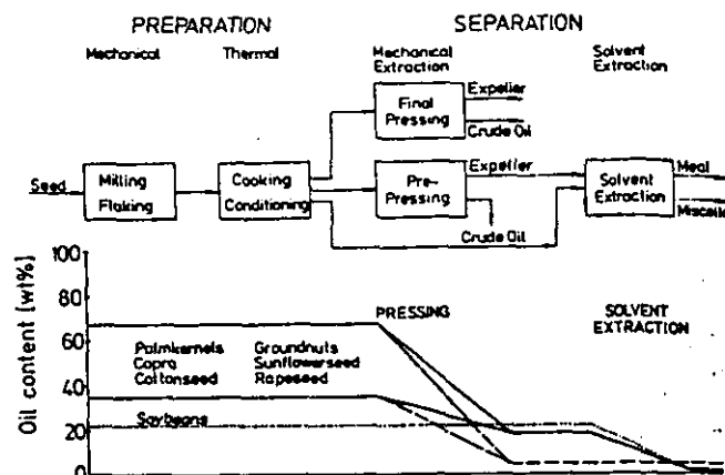
X FIG. 2. Oil recovery processes (29).
