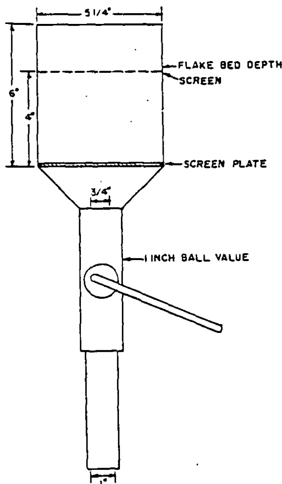
BENCH TEST FILTER FUNNEL
