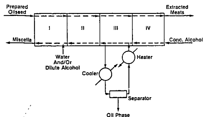
FIG. 5. Four-step alcohol extraction process (38).
