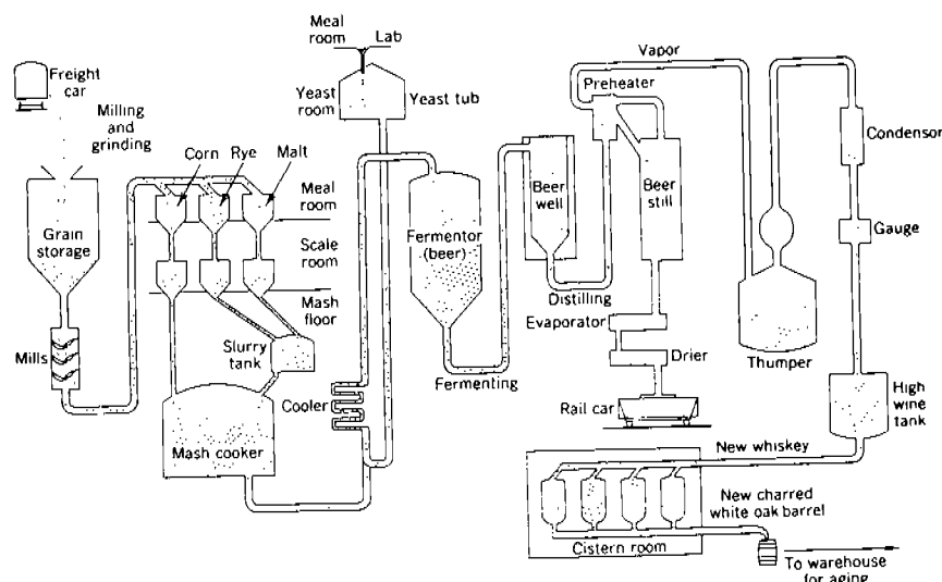
Fig. 4 Distilled beverage plant process flow sheet.
