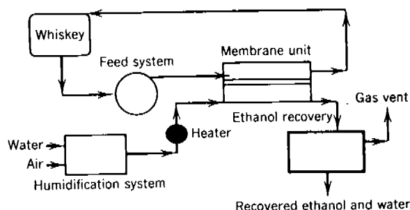
Fig. 5 Alcohol reduction pervaporation system.
