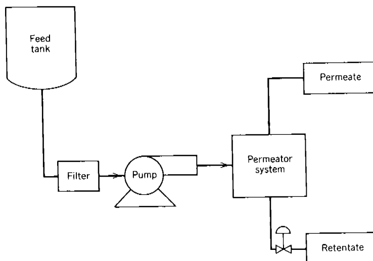
Fig. 6 High pressure reverse osmosis system for alcohol reduction.
