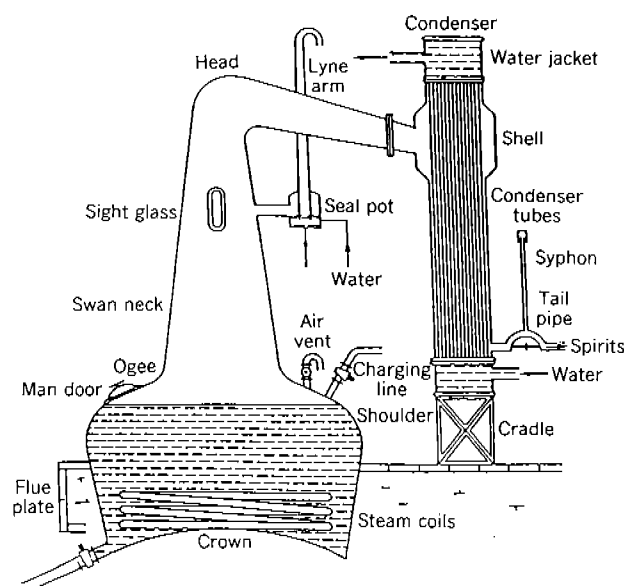
Fig. 1 Pot (batch) still.
