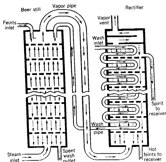
Fig. 2 Coffey continuous still.
