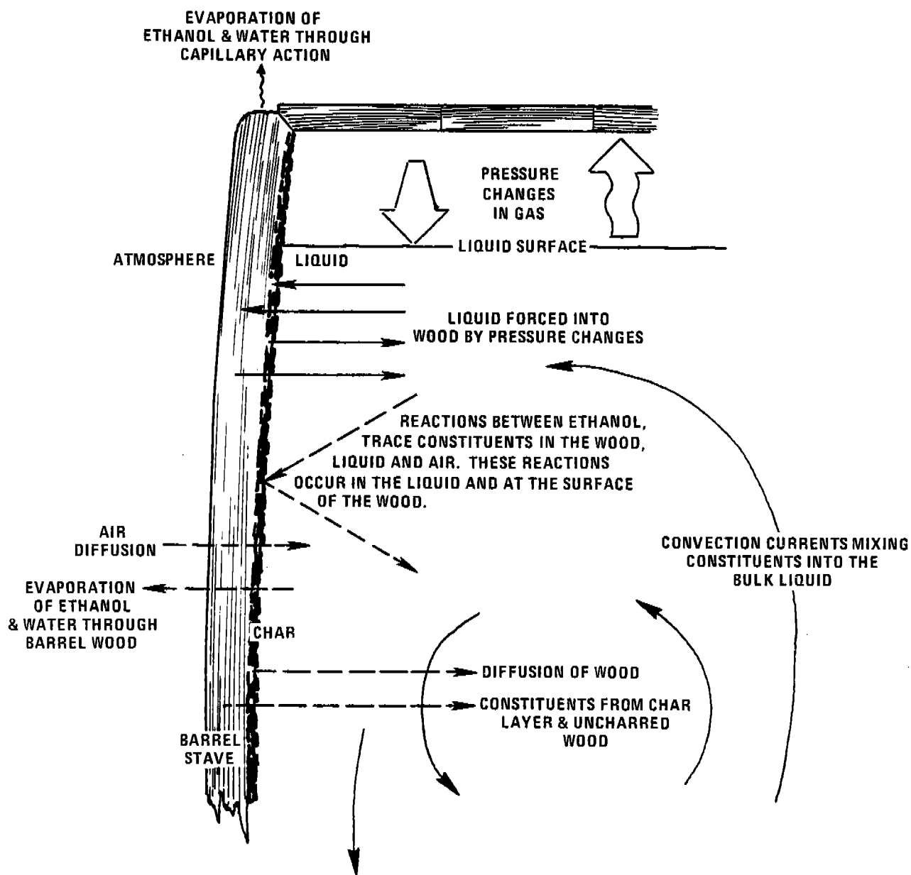
Figure 2-2. Mechanisms of whiskey aging.
