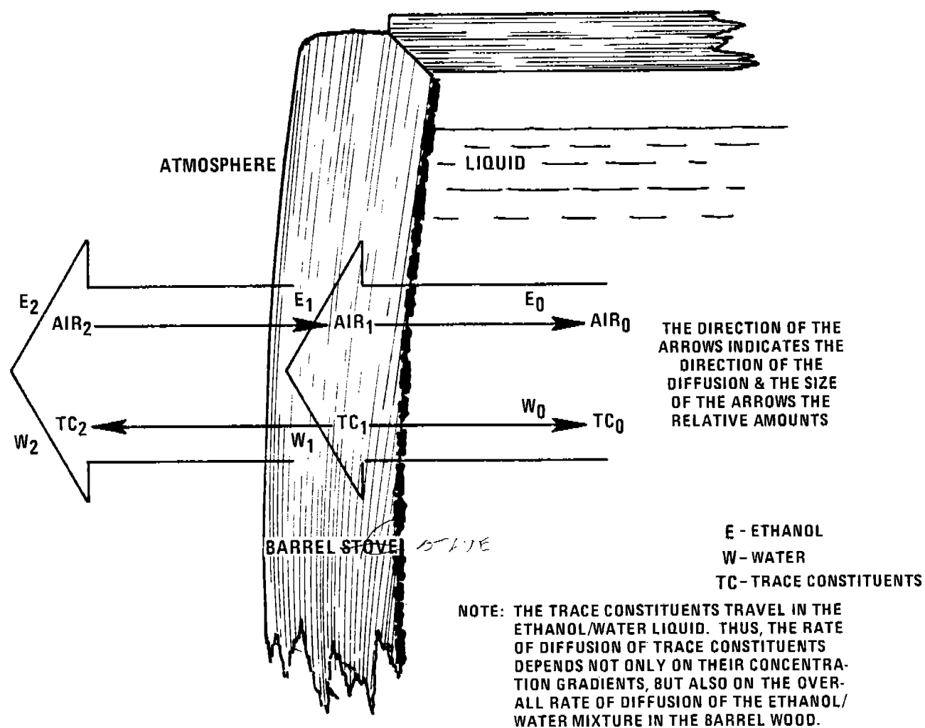
Figure 2-3. Diffusion through barrel staves in whiskey aging.
