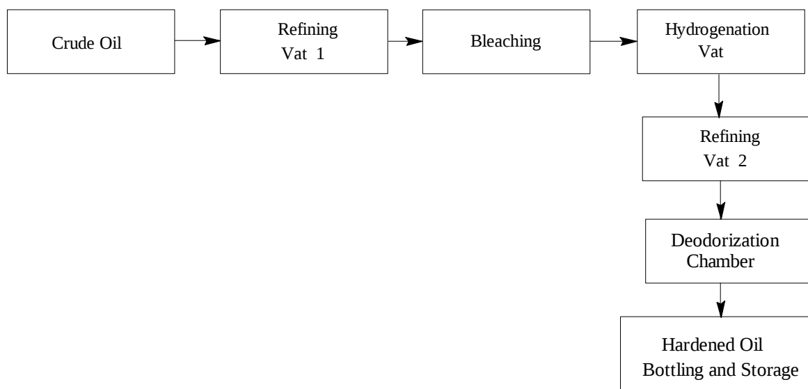
Figure 9.13.1-4. Oil hardening process.
