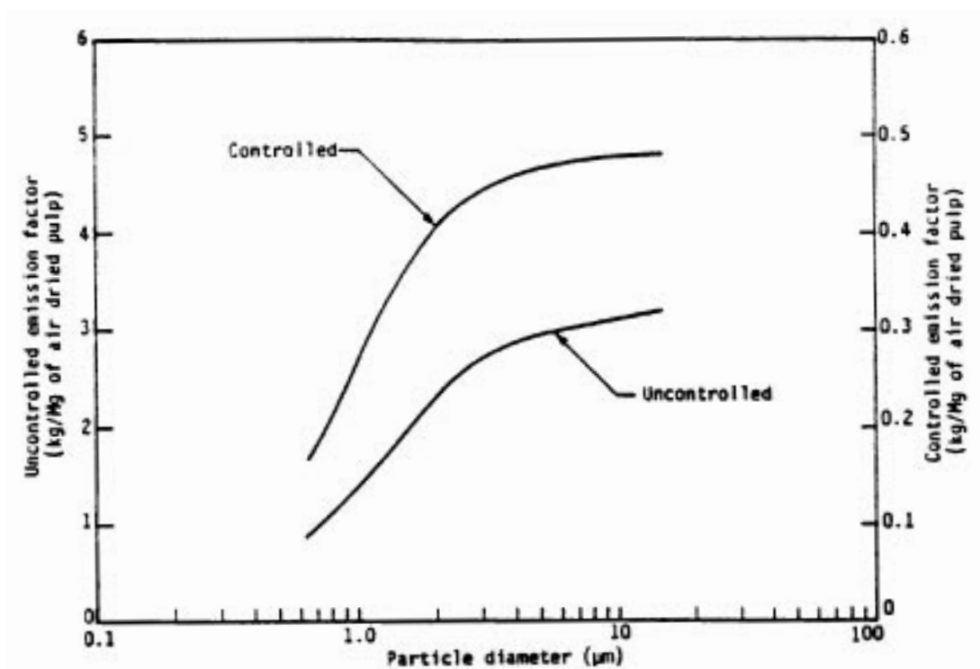
Figure 10.2-6. Cumulative particle size distribution and size-specific emission factors for smelt dissolving tank with packed tower.
