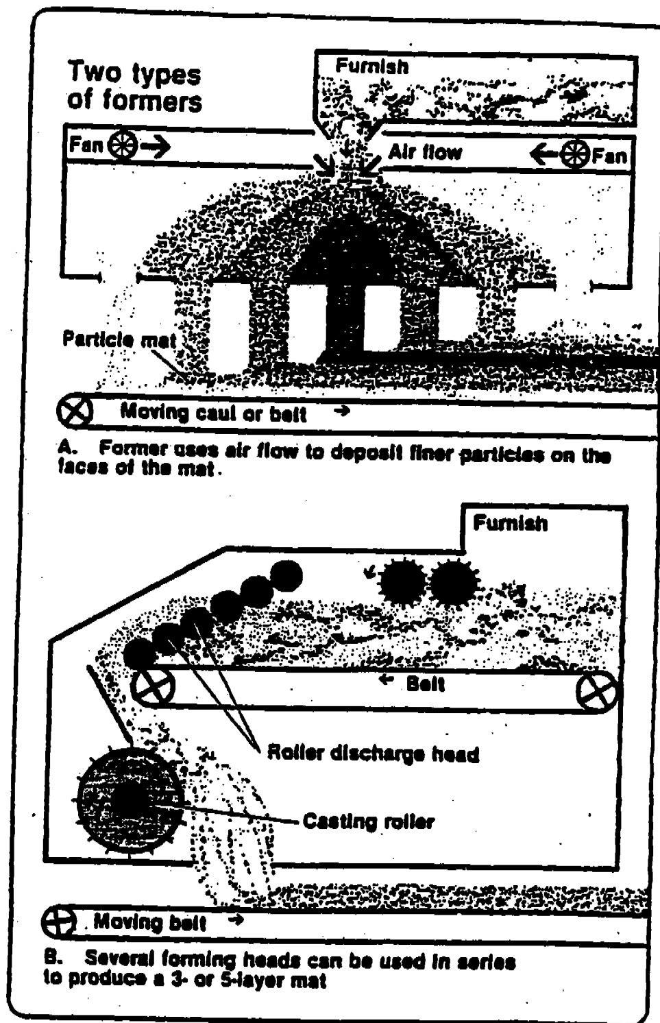
Figure 2-2. Particleboard forming machines. 2
