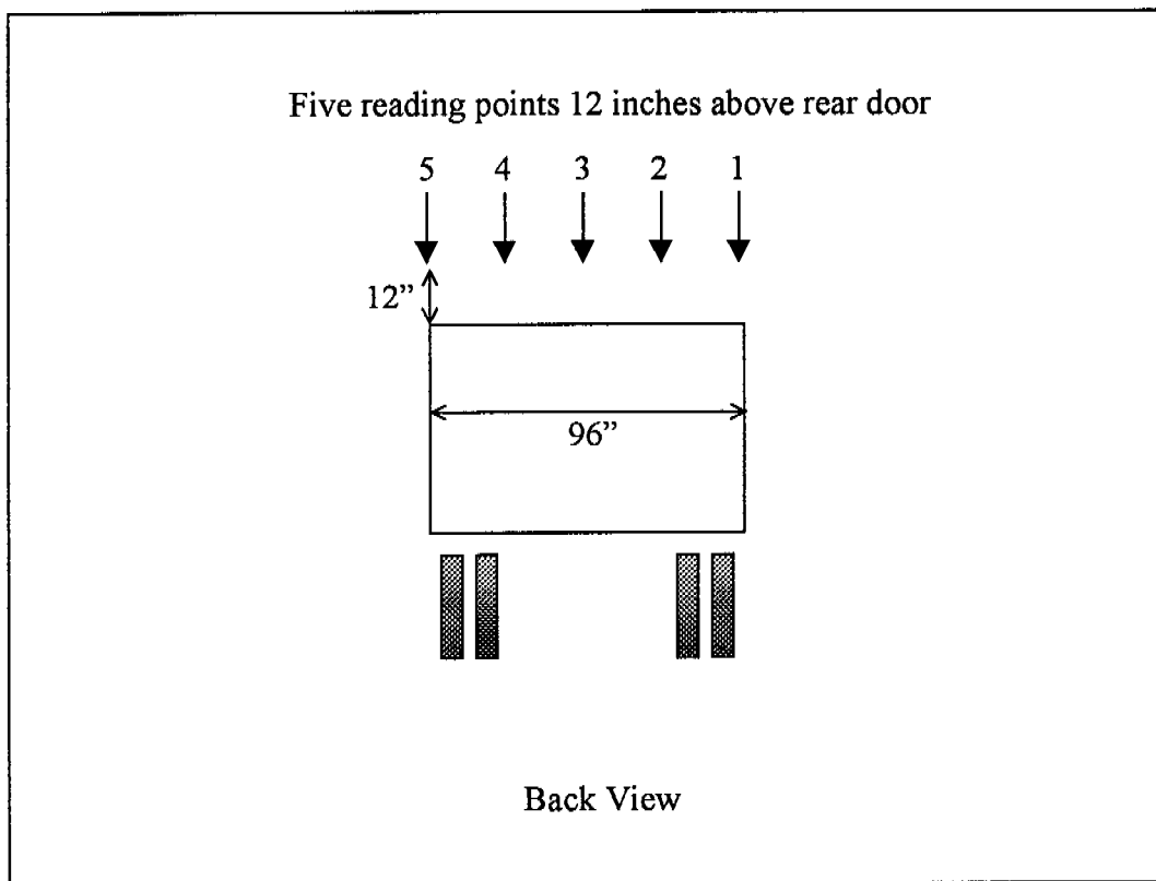
Figure 3.2 Velocity Measurement Locations and Dimensions of Transport Trucks
