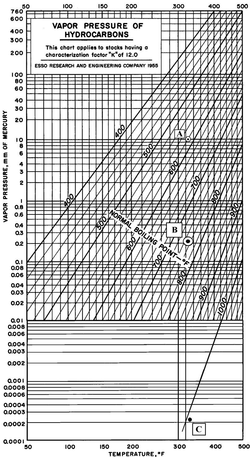
Fig. 5-25. Vapor pressure of hydrocarbon oils (low range). (Esso Research and Eng. Co.)
