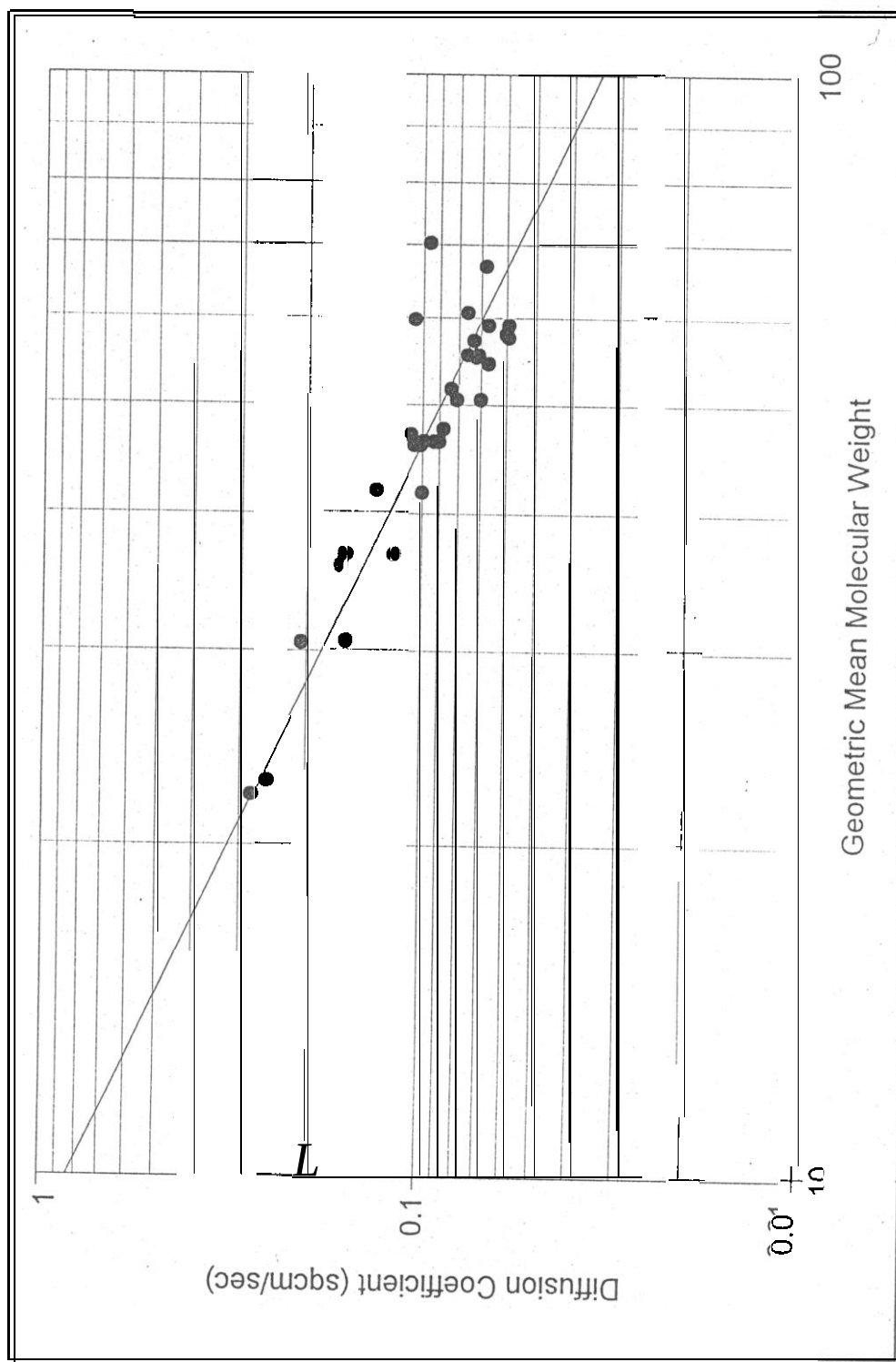
FIGURE 4.1 Diffusion Coefficients of Various Compounds in Air at 25°C [8]
