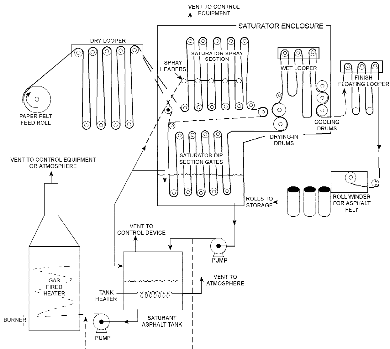
Figure 11.2-2. Asphalt-saturated felt manufacturing process. 1,2 (SCC = Source Classification Code)
